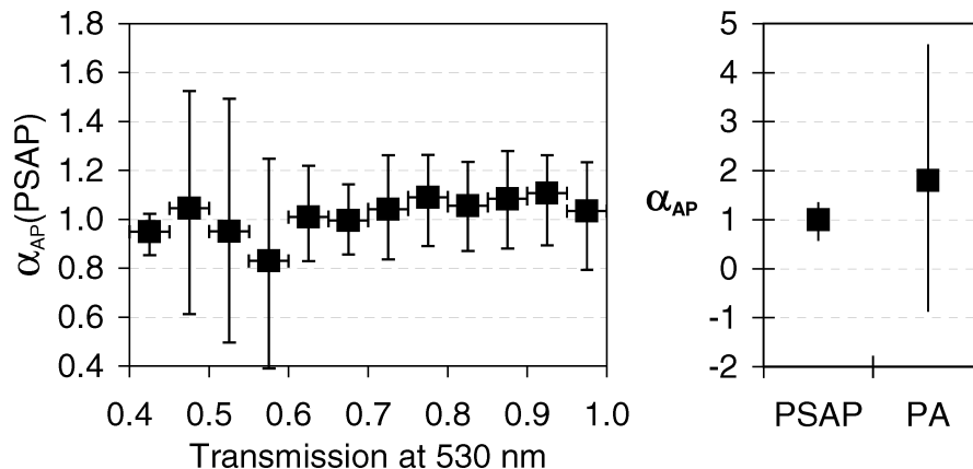
Figure 11. Ångström exponent of absorption coefficient during RAOS outdoor air experiment. Left: \alpha_{AP}(\text{PSAP}) for wavelength range 467–660 nm as a function transmission. Right: average and 5th and 95th percentiles of \alpha_{AP}(\text{PSAP}) for wavelength range 467–660 nm and \alpha_{AP}(\text{PA}) for wavelength range 532–1047 nm.
