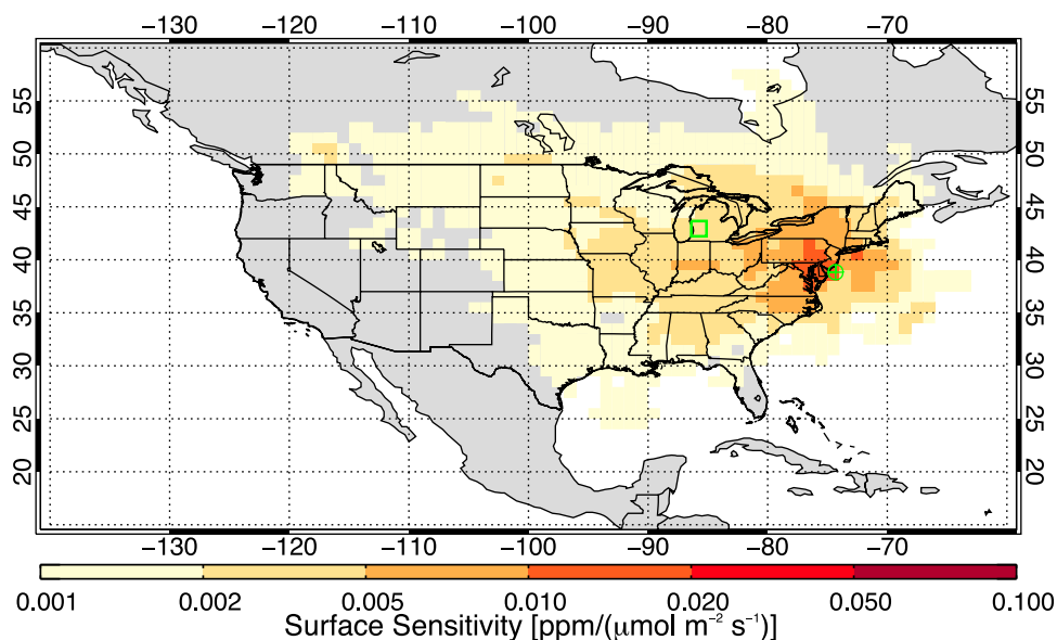
Figure 8. Average footprint for all samples collected at CMA below 2600 m asl. Footprints were calculated using the FLEXPART Lagrangian particle dispersion model as described in the text. The green crosshair is the release point (the location of the site CMA) and the green square is the ‘centroid’ of the footprint, that is, the point at which footprint contributions are equal to the north and south and east and west, respectively.
