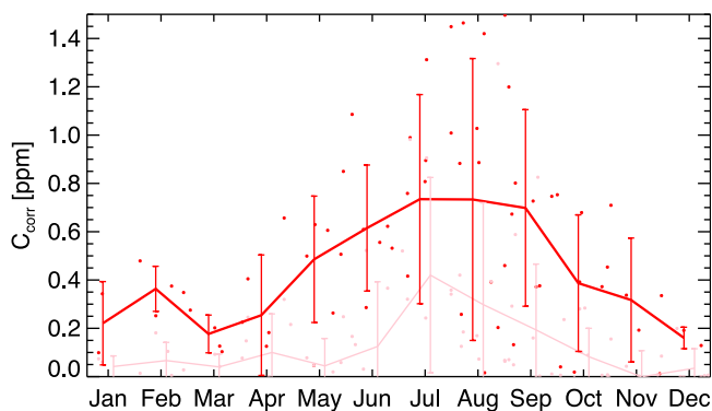
Figure 2. The correction term, C_{\text{corr}} , (see equation (2c)) for all samples by month for site CMA. Red circles are individual corrections for lower altitude samples ( \sim 300 m asl) and pink circles are corrections for mid-level altitudes ( \sim 2100 m asl). Solid lines with error bars show monthly averages for both altitudes.
