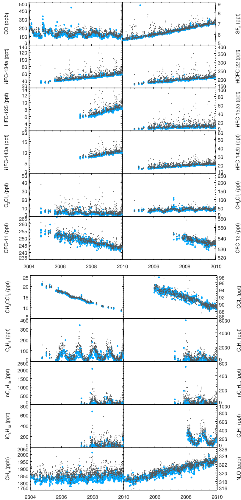
Figure 5. Time series of the 22 anthropogenic gases to which we compare C_{ff} and C_{tot} . As in Figure 4, blue represents samples collected above 2600 m asl and black represents samples below 2600 m asl.
