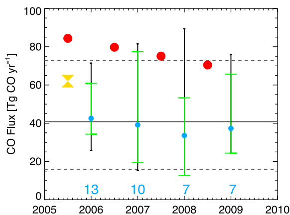
Figure 11. CO emissions for the USA for 2006–2009 derived from wintertime median atmospheric ratios (blue); EPA emission estimates (red) and EDGAR emission estimates (yellow). Top-down, C_{\text{ff}} -based emissions are plotted on the year boundary to reflect the fact that they are calculated using November–February ratios, whereas inventory-based emissions are plotted at mid-year. 2005–2009 emissions and uncertainty from Table 3 are shown as the gray solid and dashed lines. As with Figure 10, error bars (blue and gray) are the propagated 16th and 84th percentiles of the atmospheric ratio distribution transformed into emissions. Green error bars for the C_{\text{ff}} -based emissions are the 95% confidence intervals of the medians, derived from a bootstrap (with replacement) calculation. Blue numbers across the x axis reflect how many wintertime measurements were used in the calculations.
