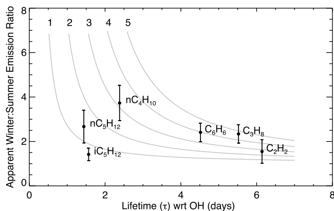
Figure 9. July atmospheric lifetime for NMHCs plotted against the apparent winter:summer emissions ratio. Values are taken from Table 2. Also plotted in gray are theoretical relationships between winter:summer apparent emission ratios (given aseasonal emissions) for atmospheric residence times between 1 and 5 days (denoted by numerals atop the curves), based on the integrated 1st order rate equation: [X] = [X]_0 \exp[-t/\tau] , where [X]_0 and [X] are the winter and summer NMHC concentrations, respectively. Note that C_{fr} , the denominator of the apparent emission ratio is not impacted by reaction with OH. The error bars are calculated by propagating the 95% confidence intervals (taken as the average of the +47.5% and -47.5%) through the quotient of the winter:summer ratio.
