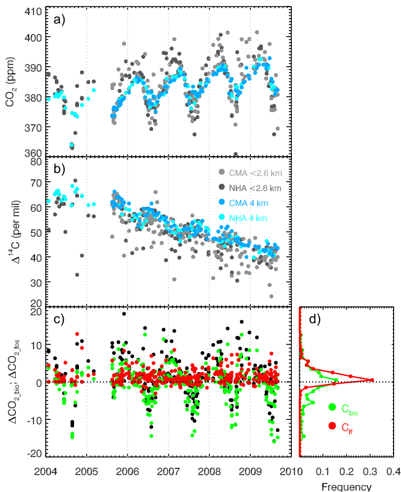
Figure 4. Observations of CO 2 and Δ 14 C used in this study. (a) The subset of CO 2 observations from NHA and CMA for which we also have Δ 14 C observations. Blue colors (cyan = NHA; light blue = CMA) represent those samples above 2600 m asl (typically ~4000 m asl), which we take to be background samples in equations (2a)–(2c); black/gray colors (black = NHA; gray = CMA) represent samples below 2600 m asl. (b) The values of Δ 14 C for the same air samples. (c) The lower troposphere CO 2 enhancement or depletion (C tot , black) split into fossil (C ff , red) and terrestrial biological (C bio , green) components using equations (2a)–(2c). (d) A projection of C ff and C bio onto the vertical axis as a histogram.
