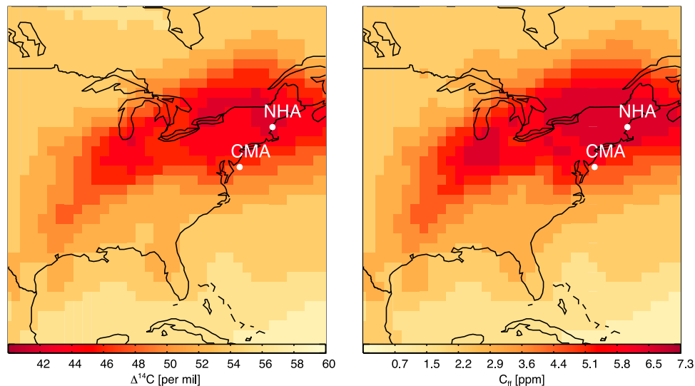
Figure 1. Model representations of (left) \Delta^{14}\text{C} and (right) the fossil fuel component of total \text{CO}_2 ( C_{\text{ff}} ) in the atmosphere near the surface over North America. Simulations were performed using the TM5 model at 1^\circ \times 1^\circ over North America with inputs for all \text{CO}_2 and \Delta^{14}\text{C} budget terms listed in equations (1a) and (1b), with the exception of nuclear reactor emissions. The fossil fuel emissions used in the model are the same as those used in the CarbonTracker data assimilation and are based on the CDIAC USA and global totals [Boden et al. , 2009], USA national seasonality [Blasing et al. , 2005] and the spatial patterns from the EDGAR inventory (see carbontracker.noaa.gov). The color scales in the two panels are not adjusted to maximize similarity between the \Delta^{14}\text{C} and C_{\text{ff}} per se, but rather scaled to the theoretical relationship between \Delta^{14}\text{C} and C_{\text{ff}} of -2.7 \text{‰ ppm}^{-1} .
