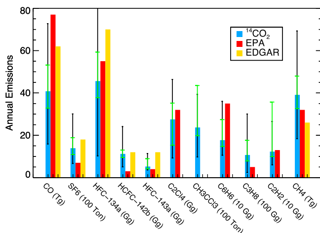
Figure 10. Emissions of selected gases for the U.S. derived from median atmospheric ratios (blue); EPA emission estimates (red) and EDGAR emission estimates (yellow). Black error bars are the propagated 16th and 84th percentiles of the apparent emission ratio distribution, and green error bars represent the 95% confidence intervals of the median emission values. This calculation assumes that the emission ratios derived for the northeast U.S. are valid nationally and we include the (generally) larger distribution-based error bars as a proxy for unaccounted for differences between northeastern and national apparent emission ratios (see main text).
