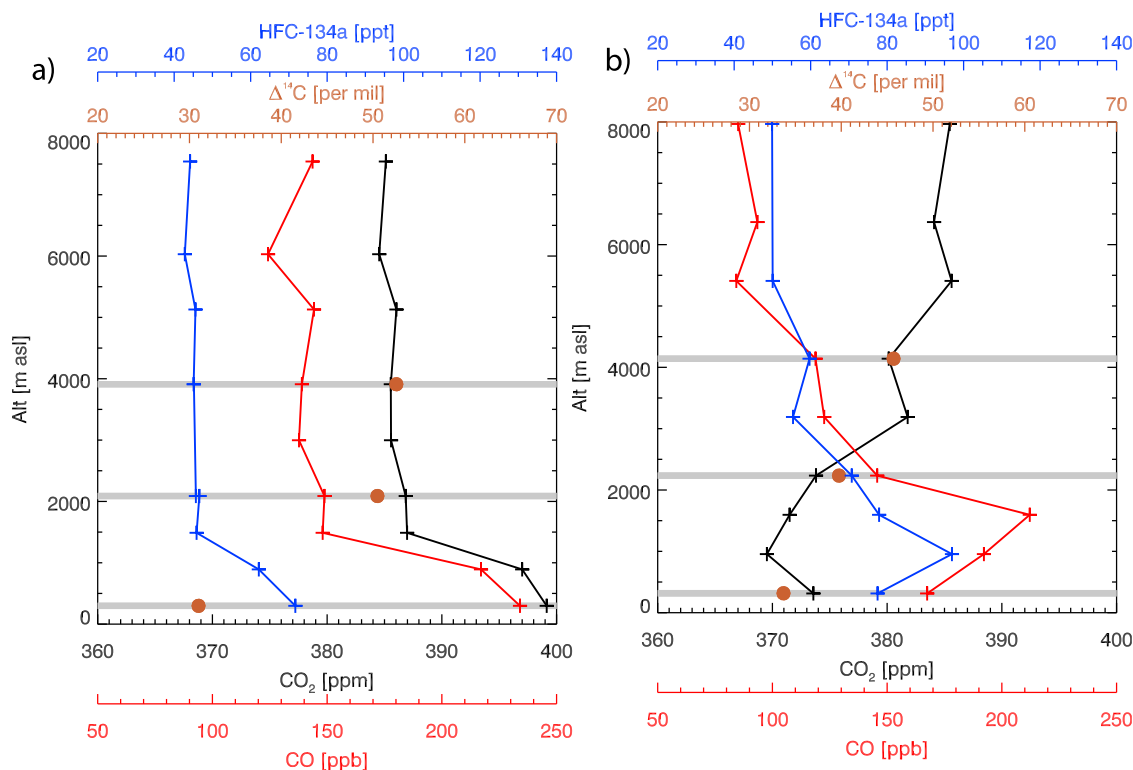
Figure 3. Example vertical profiles (a) above site CMA (offshore from Cape May, NJ) from Feb. 21, 2007 and (b) above site NHA (offshore from Portsmouth, NH) from July 10, 2008. Black, red and blue pluses connected with a line represent nine air samples collected between the surface and 8 km asl, with results for \text{CO}_2 , CO, and HFC-134a, respectively. Brown circles represent values from the three altitudes at which \Delta^{14}\text{C} is analyzed. Grey bars highlight the altitudes at which all gases are measured. Figure 3a shows a typical profile in which \text{CO}_2 , CO and HFC-134a are elevated and \Delta^{14}\text{C} is reduced, due to anthropogenic emissions. Figure 3b shows a summertime example where fossil fuel \text{CO}_2 is masking the true extent of net photosynthetic uptake by the terrestrial biosphere.
