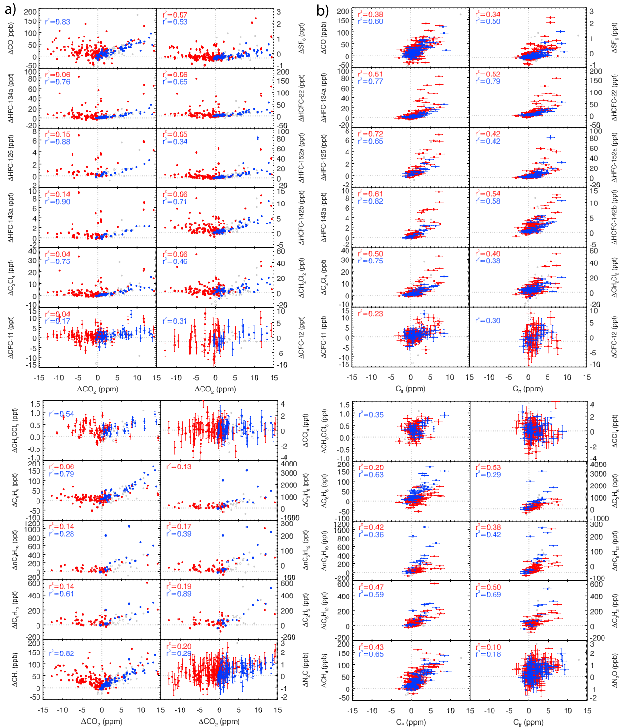
Figure 6. Scatterplots of (a) \Delta\text{CO}_2 (lower troposphere minus free troposphere \text{CO}_2 , referred to as C_{\text{tot}} in the text), or (b) C_{\text{ff}} , versus \Delta_{\text{gas}} (lower troposphere minus free troposphere differences of the anthropogenic gases listed in Tables 1a, 1b and 1c). Red circles represent samples collected between May and September and blue circles represent samples collected between December and February. Grey circles represent samples collected during other months. Open circles represent our “mid-level” samples from 2000 – 2600 m asl; closed circles represent lower level samples 300–600 m asl. All plots have the same x axis ( \text{CO}_2 ) scales and the y axis scales are the same for individual gases in Figures 6a and 6b. X and y error bars are plotted for all summer and winter data, although in many cases error bars are smaller than the symbol sizes. r^2 values are printed on each graph and colored according to season for all regressions in which the r^2 is significantly different from zero at p < 0.05 (two-tailed).
