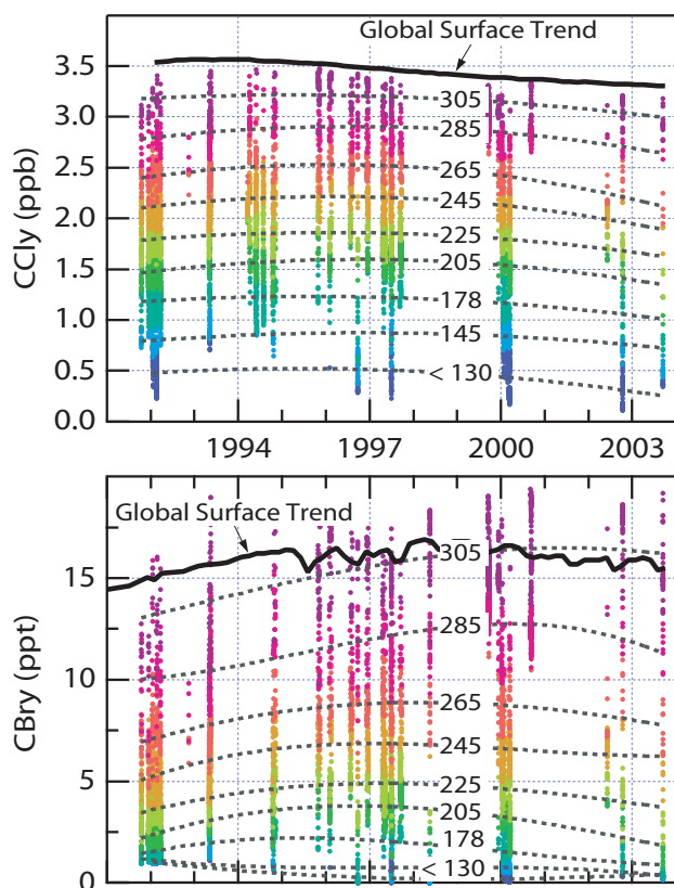
Figure 5.22. Trends in organic chlorine (top) and bromine (bottom) in the stratosphere from ACATS-IV and LACE flights during 1991-2003. \text{CCl}_y and \text{CBr}_y data are colored according to their \text{N}_2\text{O} mixing ratio bin with bin midpoints labeled on the plot. The six highest bins are 20 ppb \text{N}_2\text{O} in width (i.e., midpoint 305 for 295-315 ppb bin), the next lowest two bins are 30 ppb wide, and the lowest bin incorporates all \text{N}_2\text{O} mixing ratios <130. \text{N}_2\text{O} bins group the air masses sampled according to their photochemical histories (see text). Dashed curves are 3 rd -order polynomial fits to binned data for the 12-year period.
