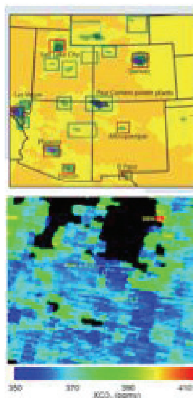
Figure F-2. Column CO 2 from SCHIAMACHY (ESA).
