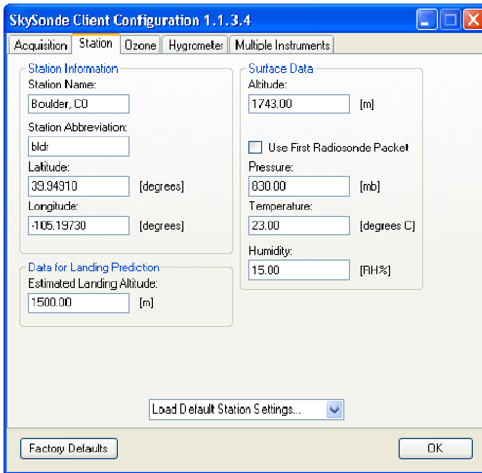
Figure 3: The Station tab in the SkySonde Client's configuration dialog
