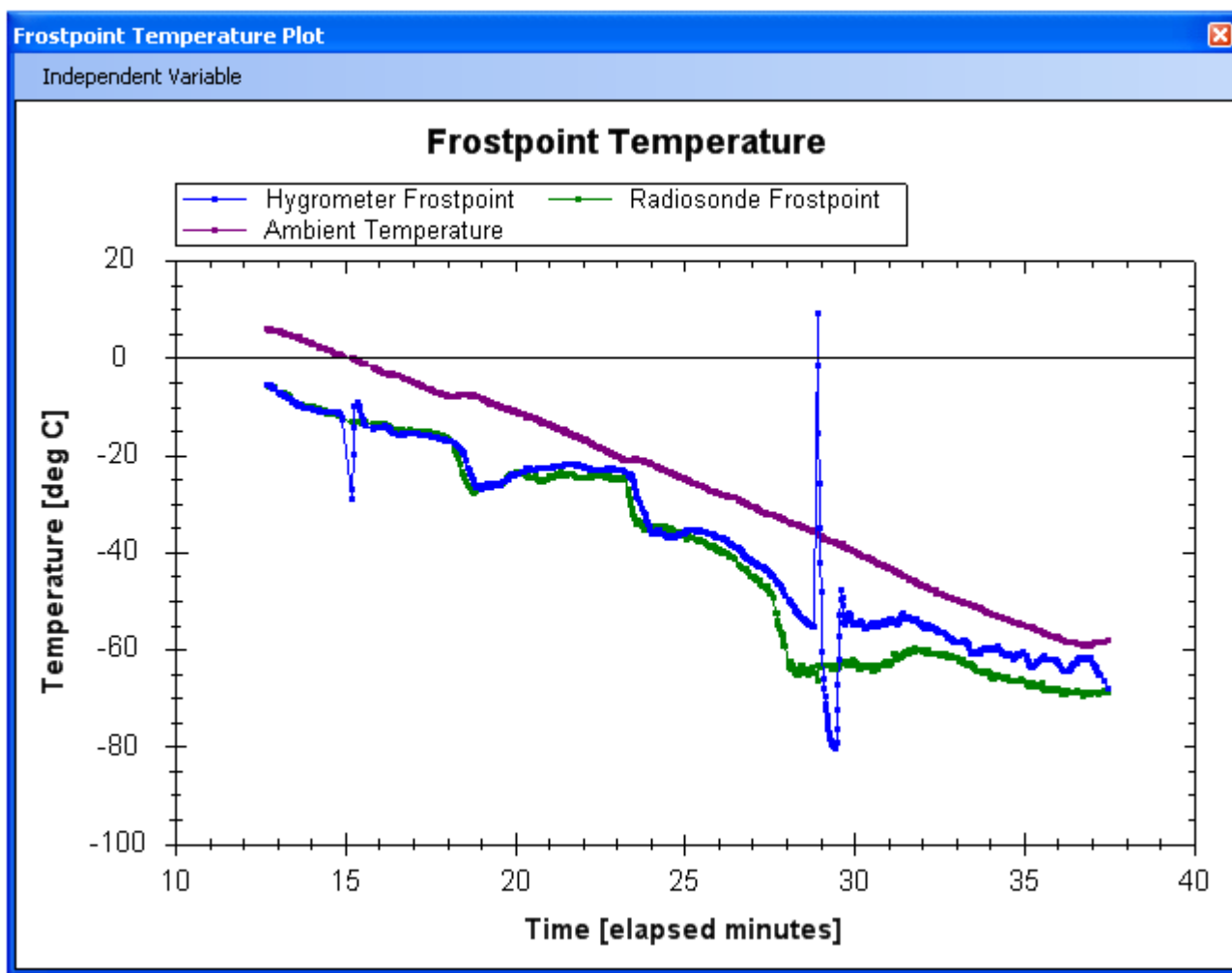
Figure 8: A time plot of the hygrometer's frostpoint temperature
