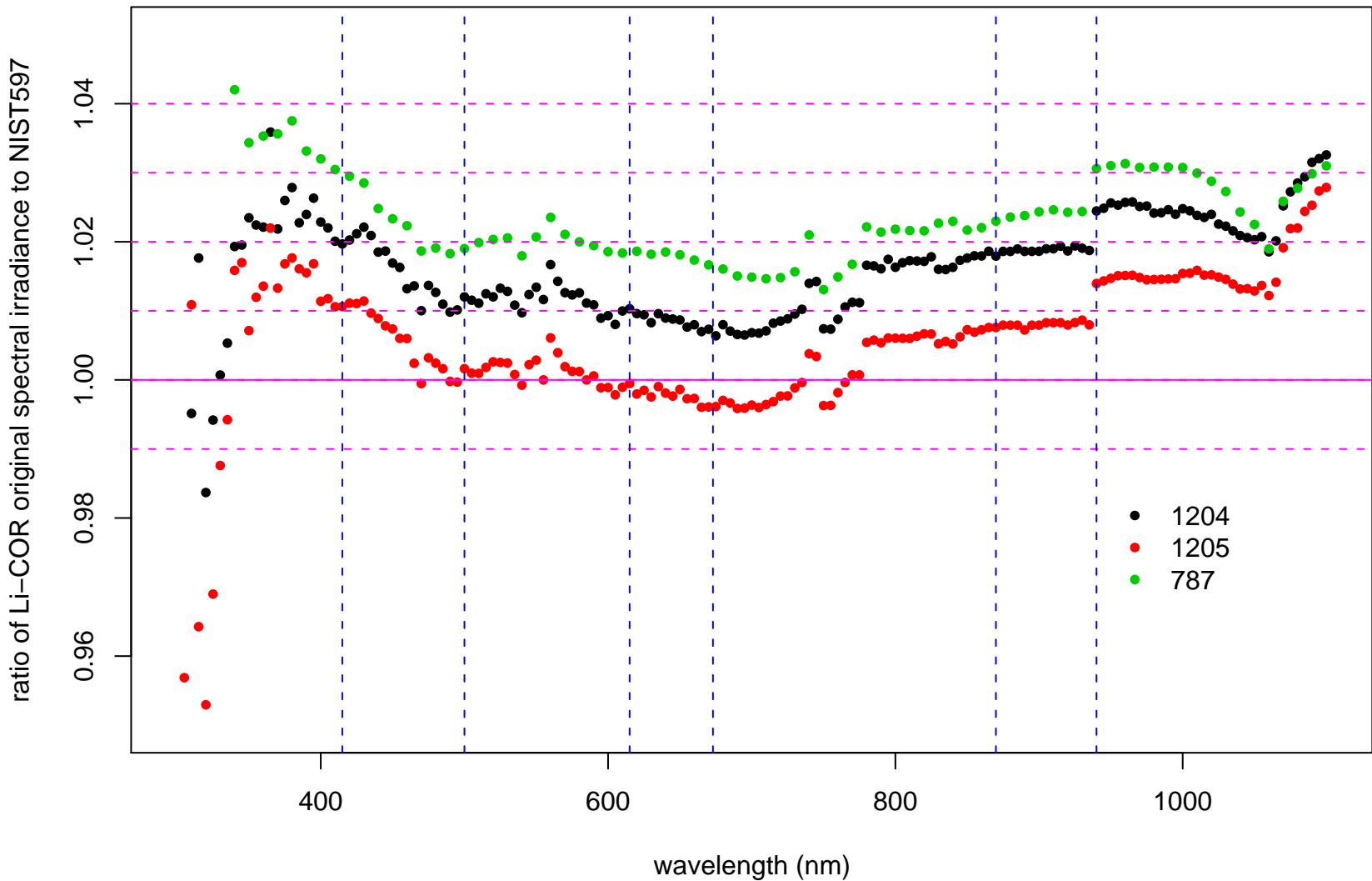
Cal on 11-21-2007; Vertical Lines are MFRSR Wavelengths
