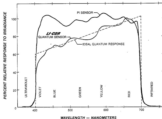
Figure 1. Typical spectral response of LI-COR Quantum Sensors and a photosynthetic irradiance sensor vs. wavelength and ideal quantum response.
