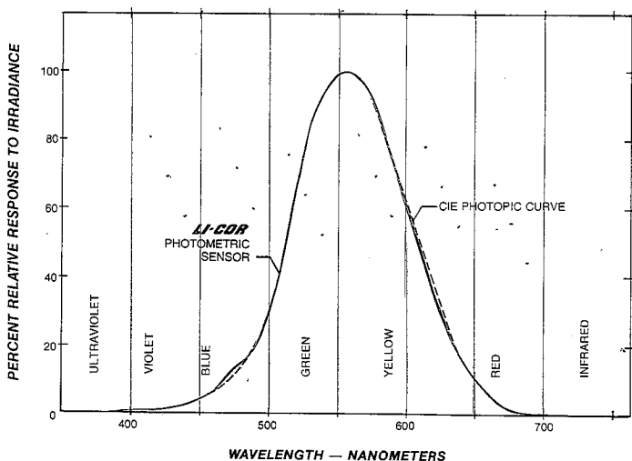
Figure 3. Typical spectral response of LI-COR Photometric Sensors vs. the CIE photopic response curve.
