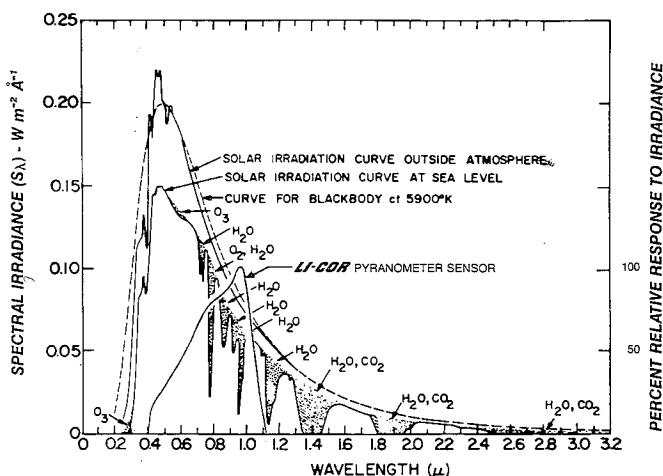
Figure 4. The LI-200SA Pyranometer spectral response is illustrated along with the energy distribution in the solar spectrum (5).
