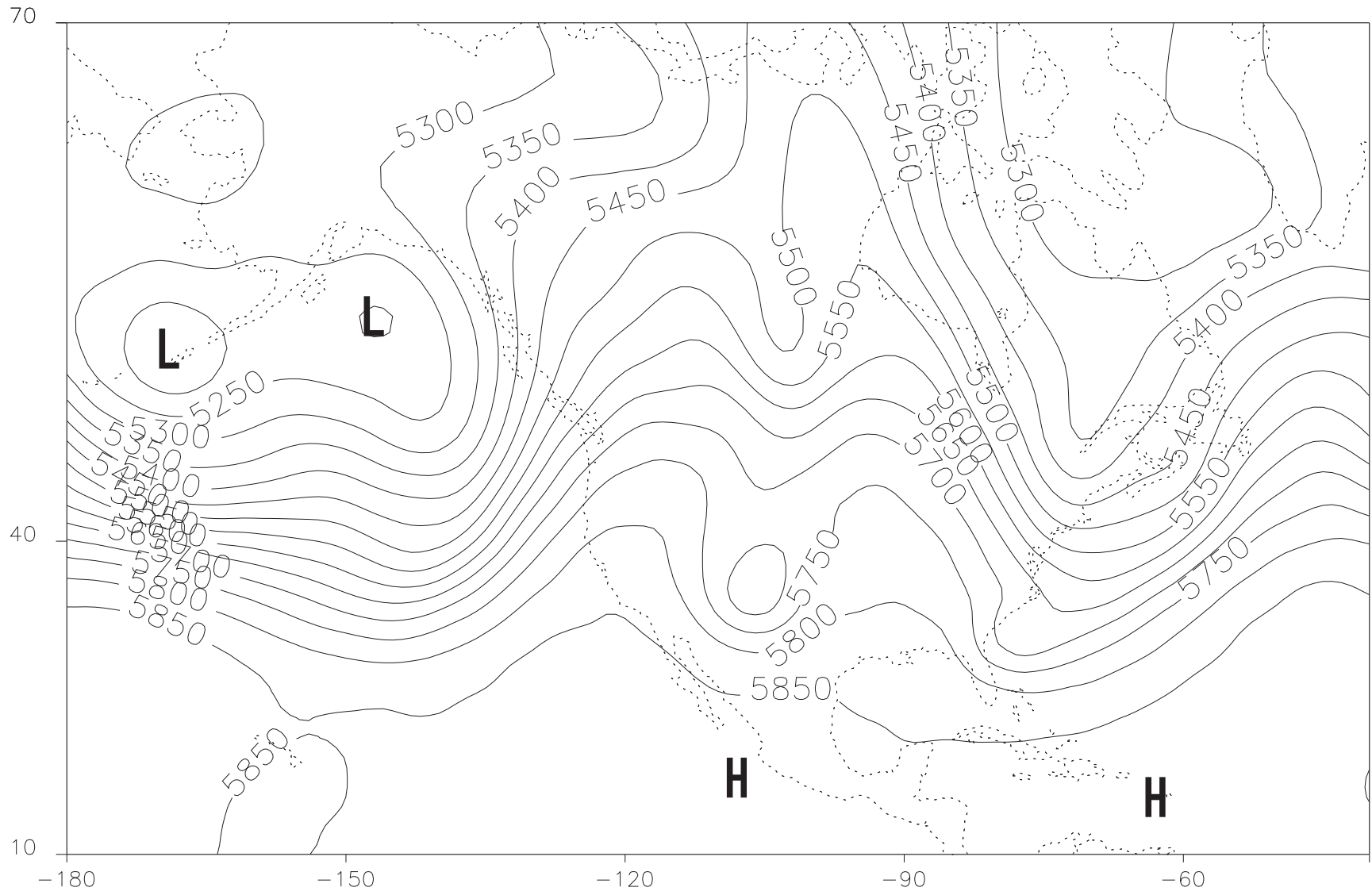
Elevation (m) of the 500 hPa Surface on 2000/4/30 at 12UT
