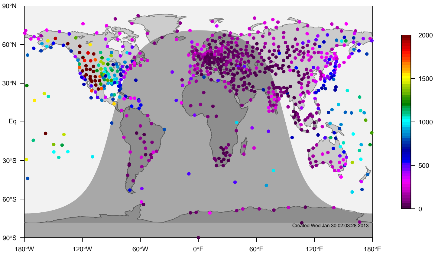
IGRA mixing height at 0UTC for May (1981-2006)
