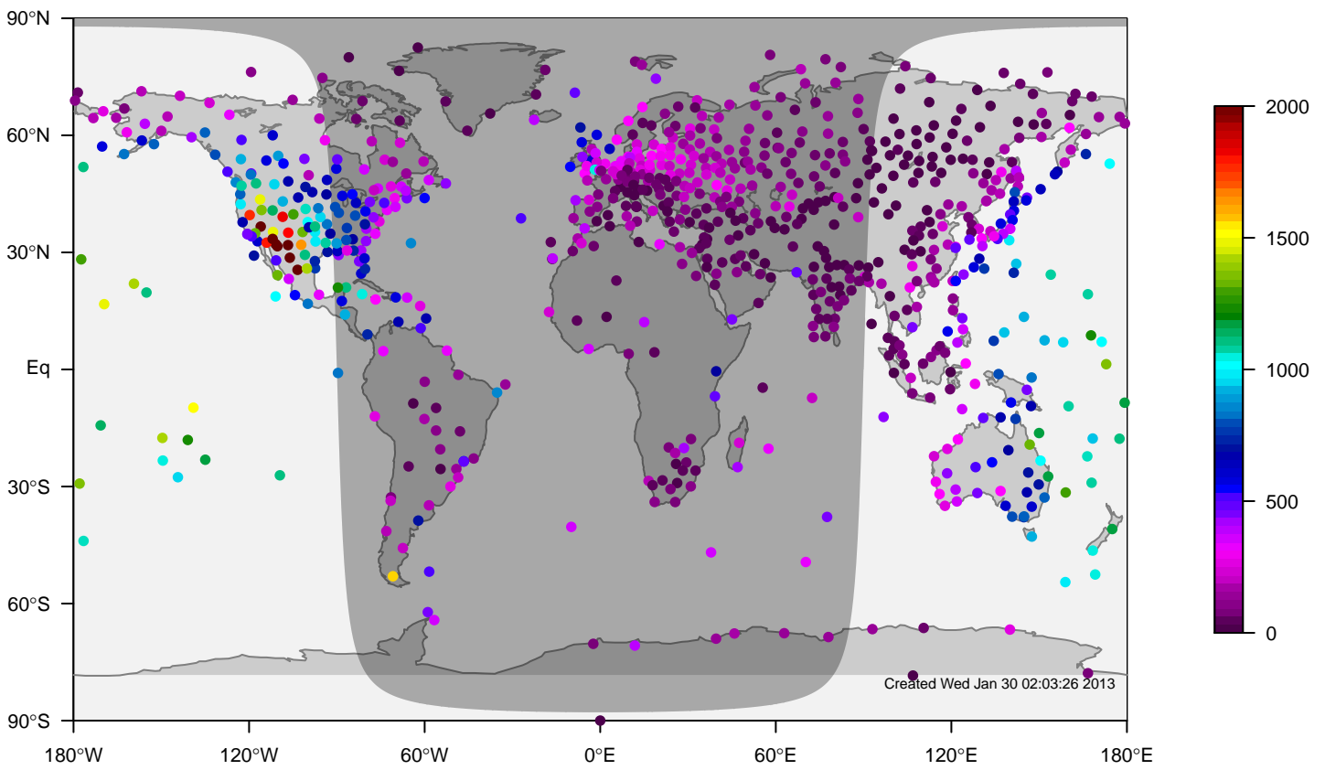
IGRA mixing height at OUTC for March (1981–2006)
