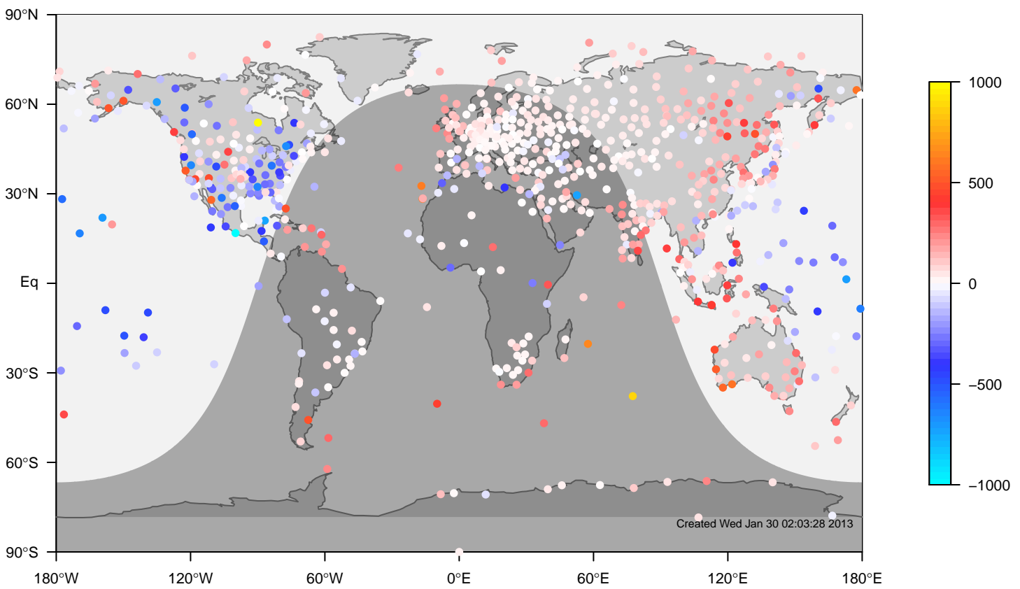
ERA-i minus IGRA bias at 0UTC for June (1981-2006)
