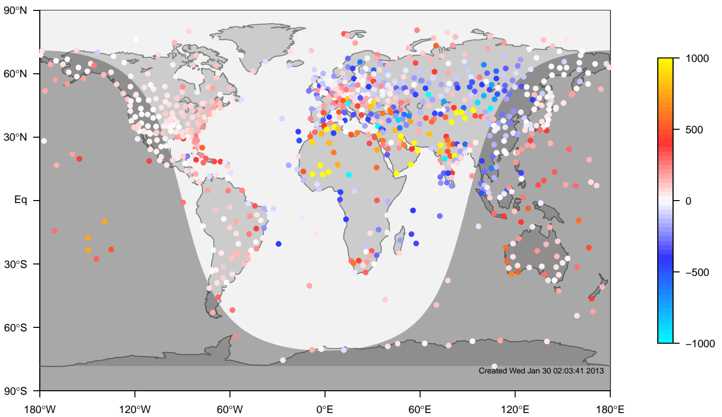
ERA-i minus IGRA bias at 12UTC for May (1981-2006)
