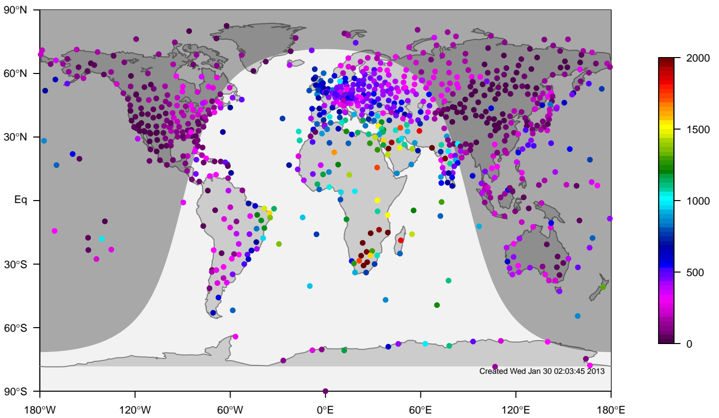
IGRA mixing height at 12UTC for November (1981-2006)
