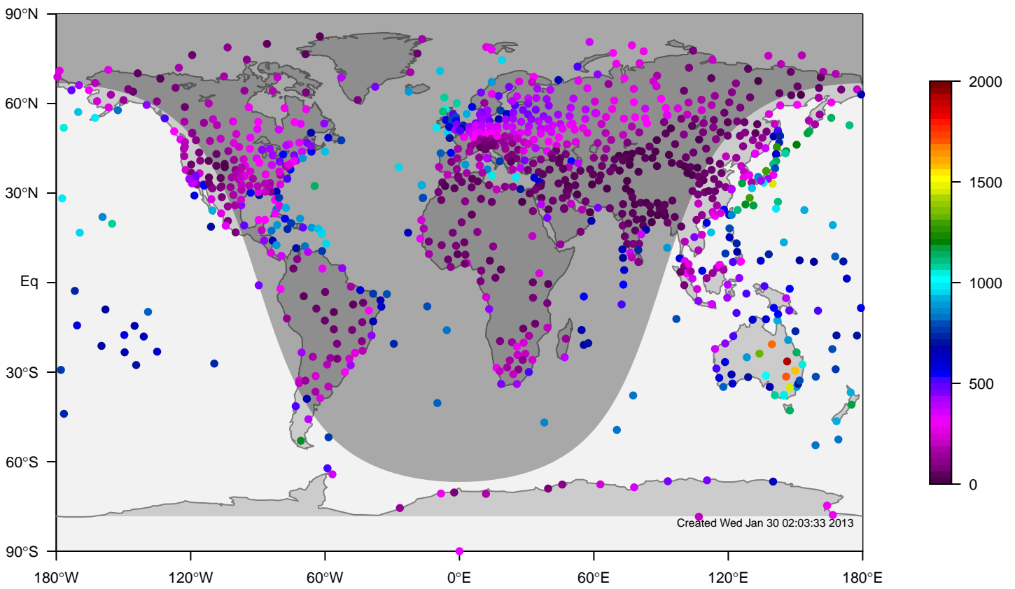
ERA-i mixing height at 0UTC for December (1981-2006)
