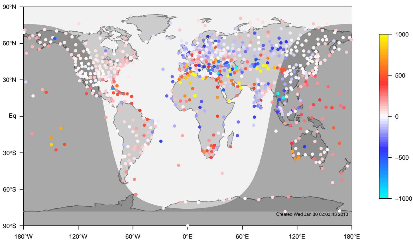
ERA-i minus IGRA bias at 12UTC for August (1981-2006)
