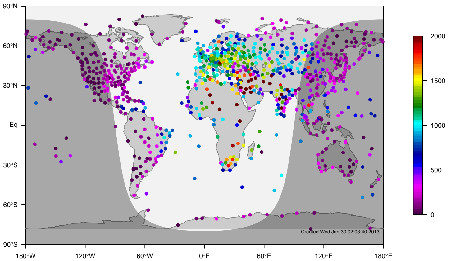
IGRA mixing height at 12UTC for April (1981-2006)
