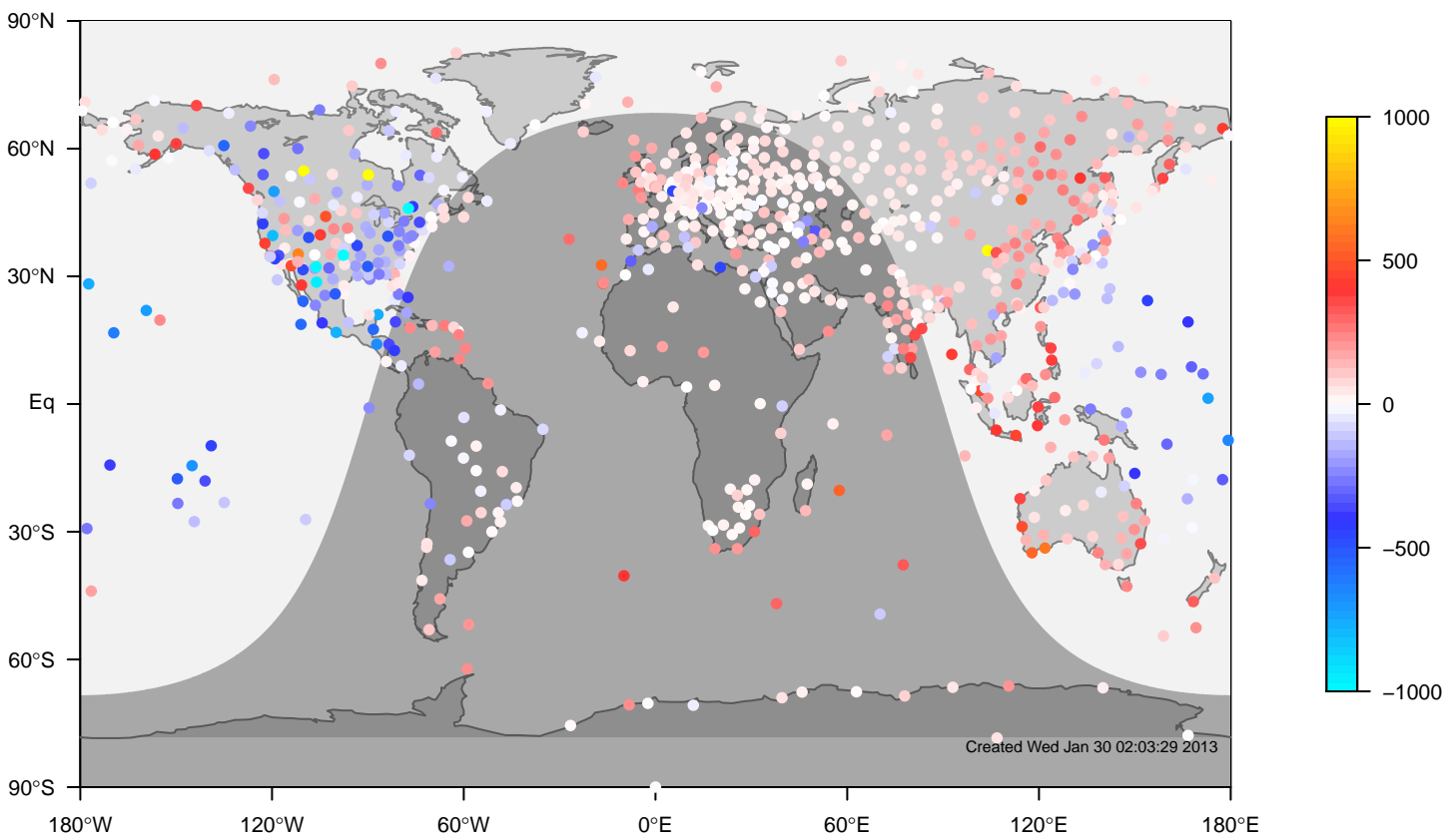
ERA-i minus IGRA bias at 0UTC for July (1981-2006)
