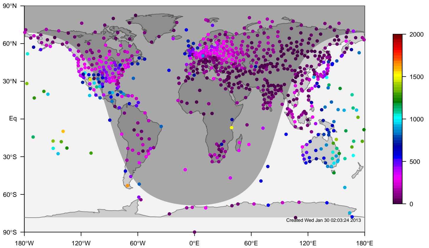
IGRA mixing height at OUTC for January (1981–2006)
