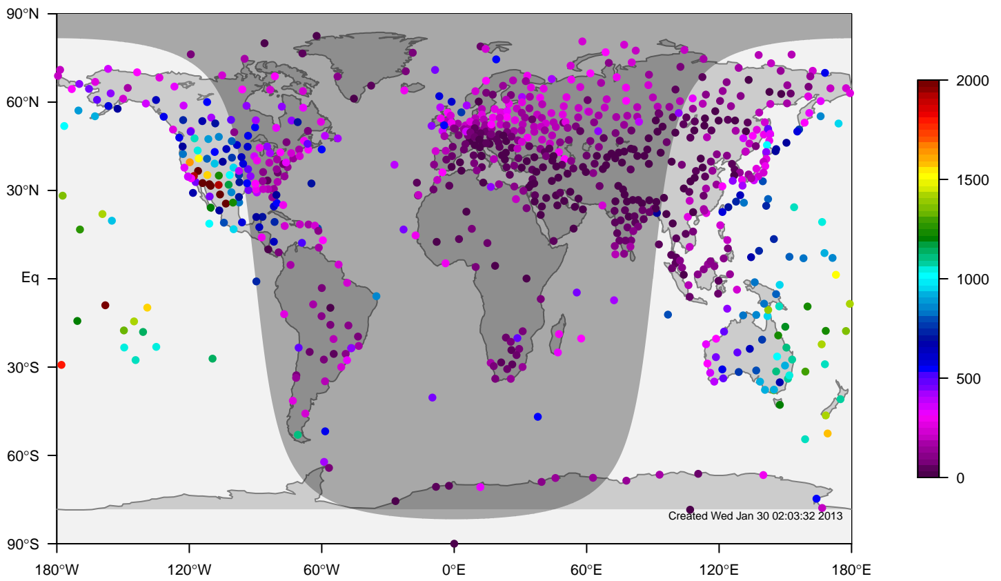
IGRA mixing height at 0UTC for October (1981-2006)
