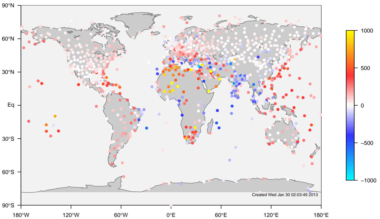
ERA-i minus IGRA all-season bias at 12UTC (1981 - 2006)
