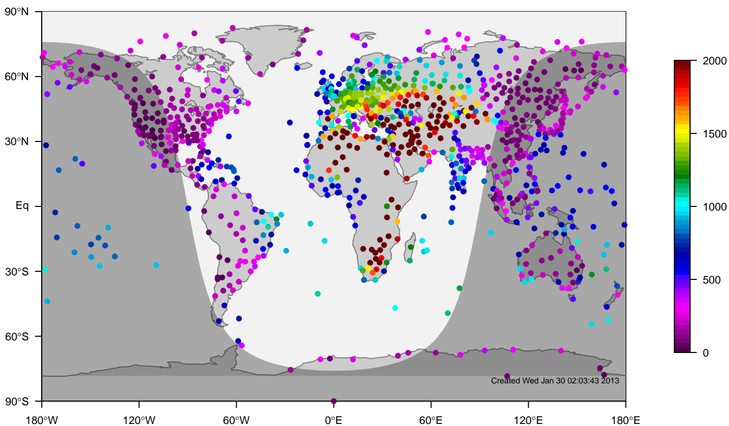
ERA-i mixing height at 12UTC for August (1981-2006)
