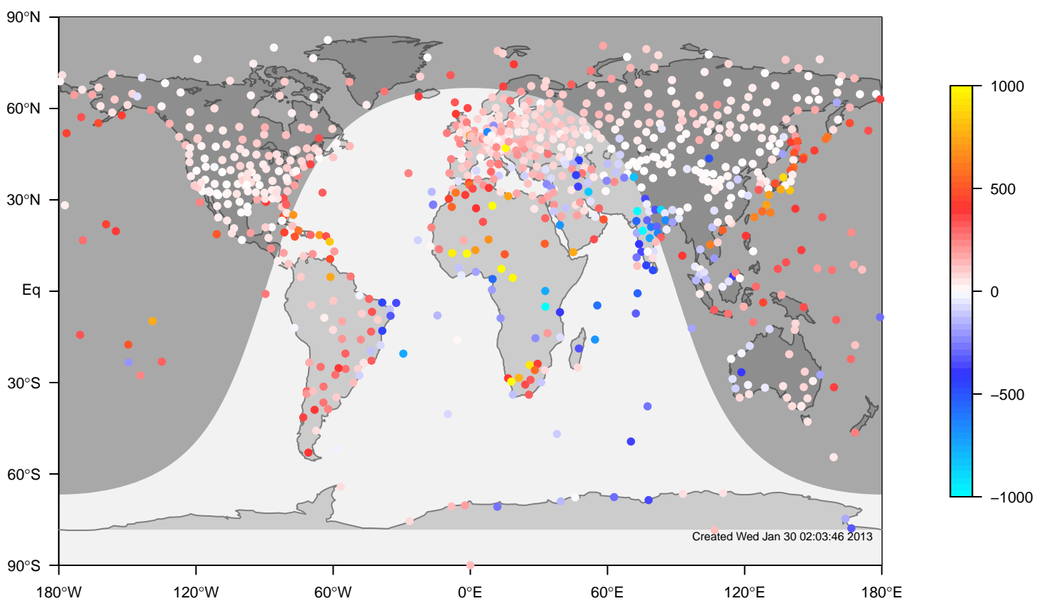
ERA-i minus IGRA bias at 12UTC for December (1981–2006)
