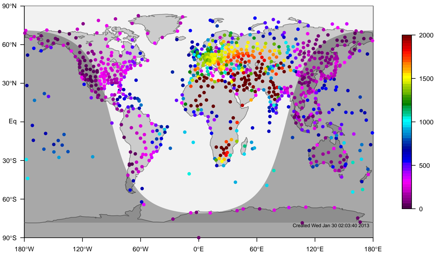
ERA-i mixing height at 12UTC for May (1981-2006)
