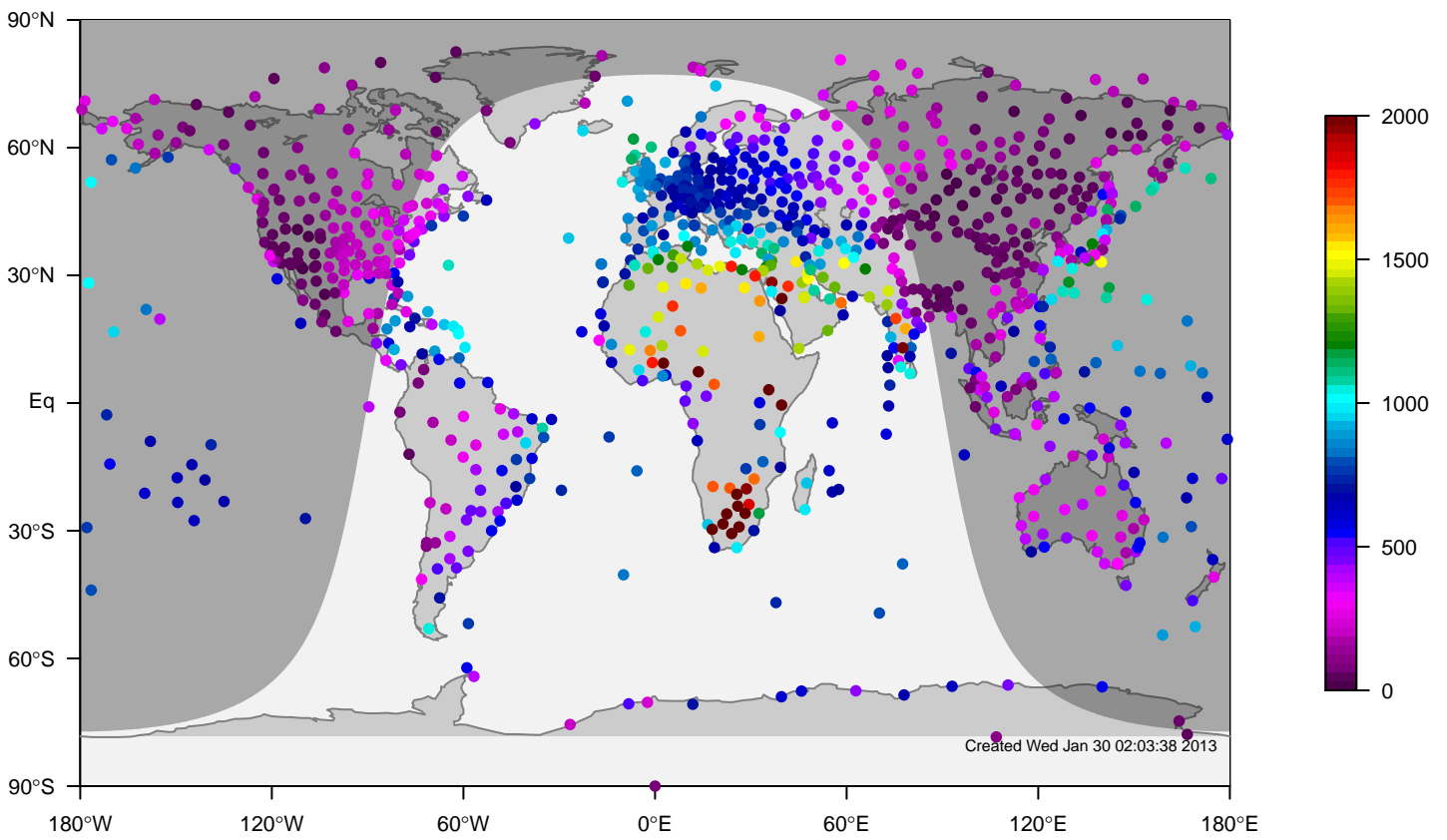
ERA-i mixing height at 12UTC for February (1981-2006)
