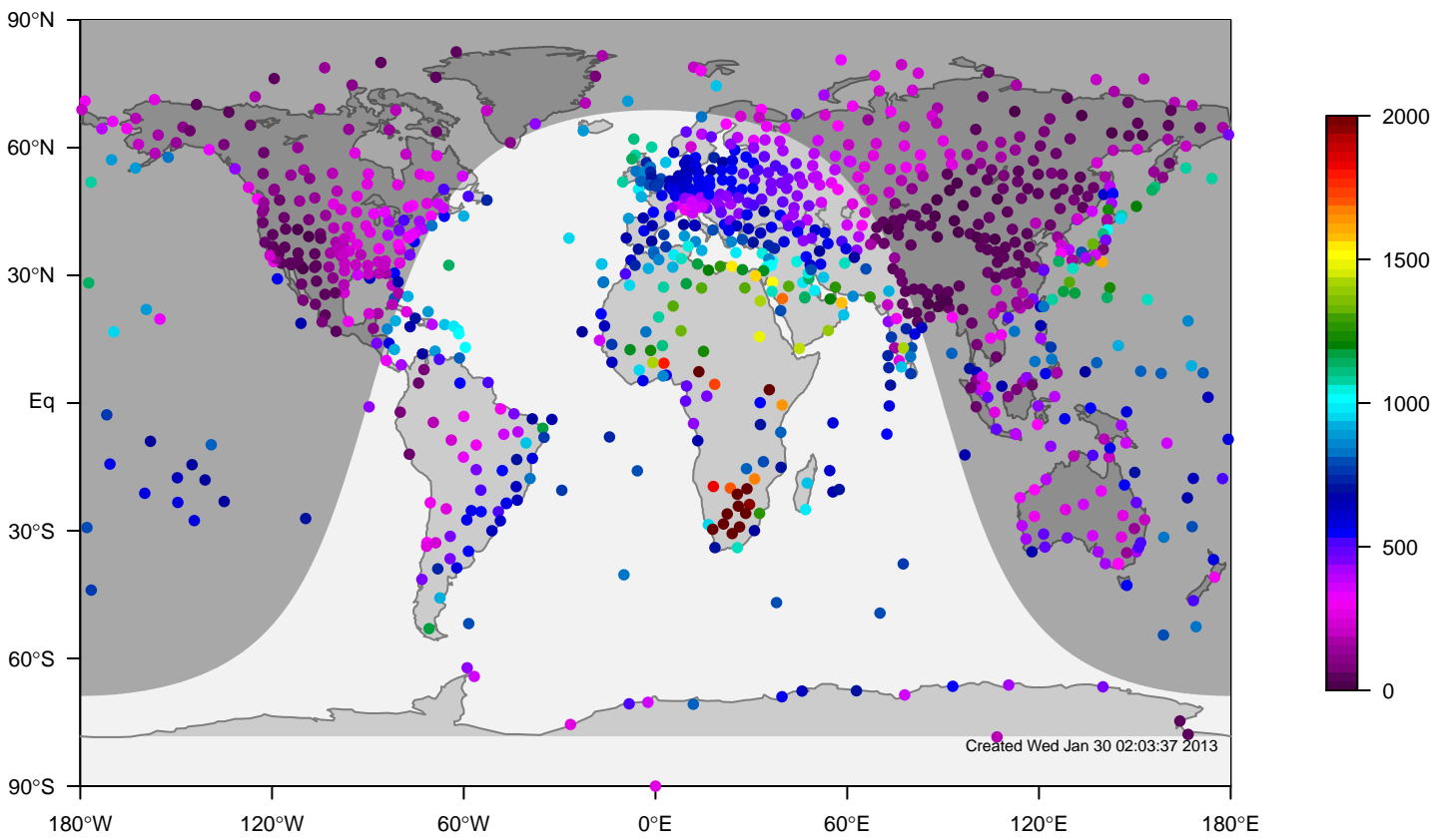
ERA-i mixing height at 12UTC for January (1981-2006)
