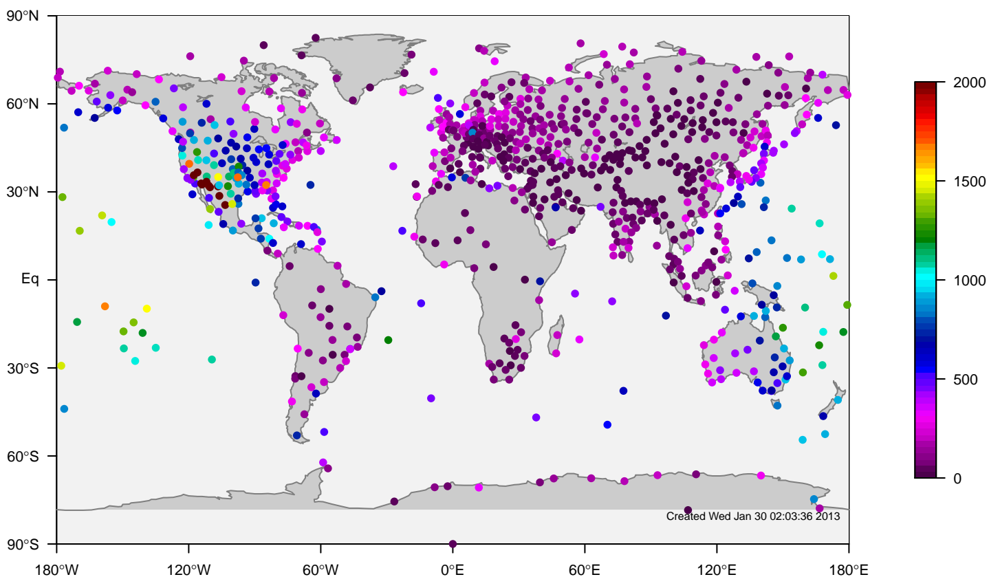
IGRA all-season mixing height at OUTC (1981-2006)
