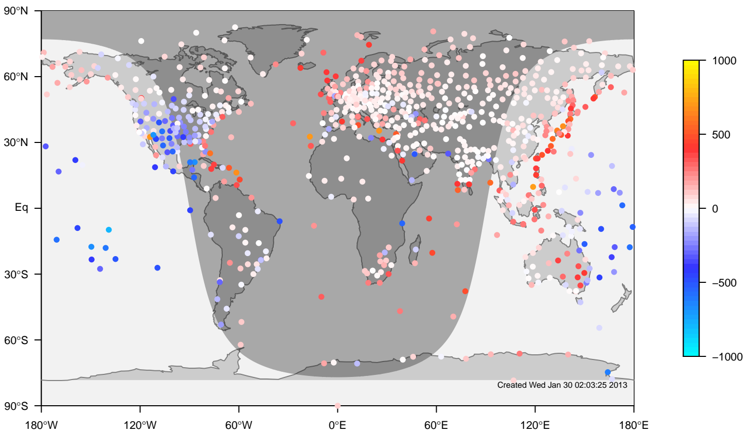
ERA-i minus IGRA bias at OUTC for February (1981-2006)
