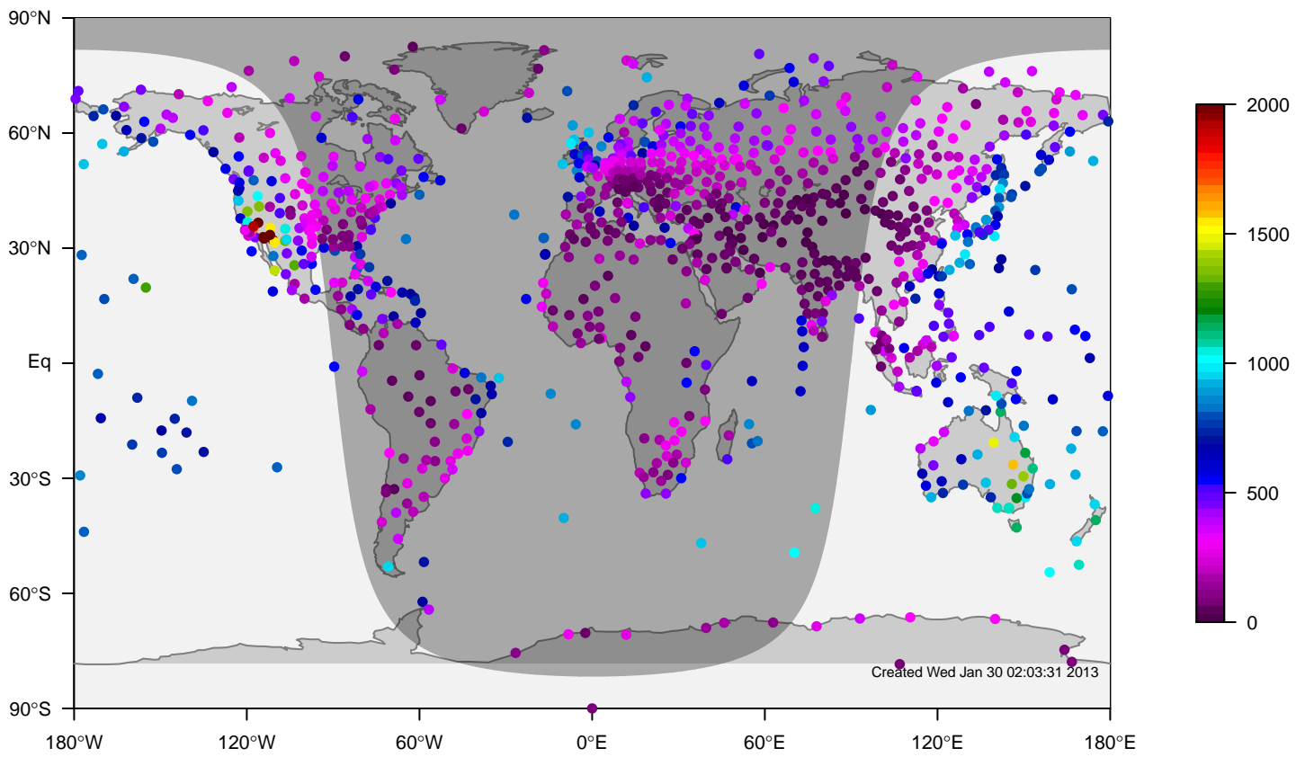
ERA-i mixing height at 0UTC for October (1981-2006)
