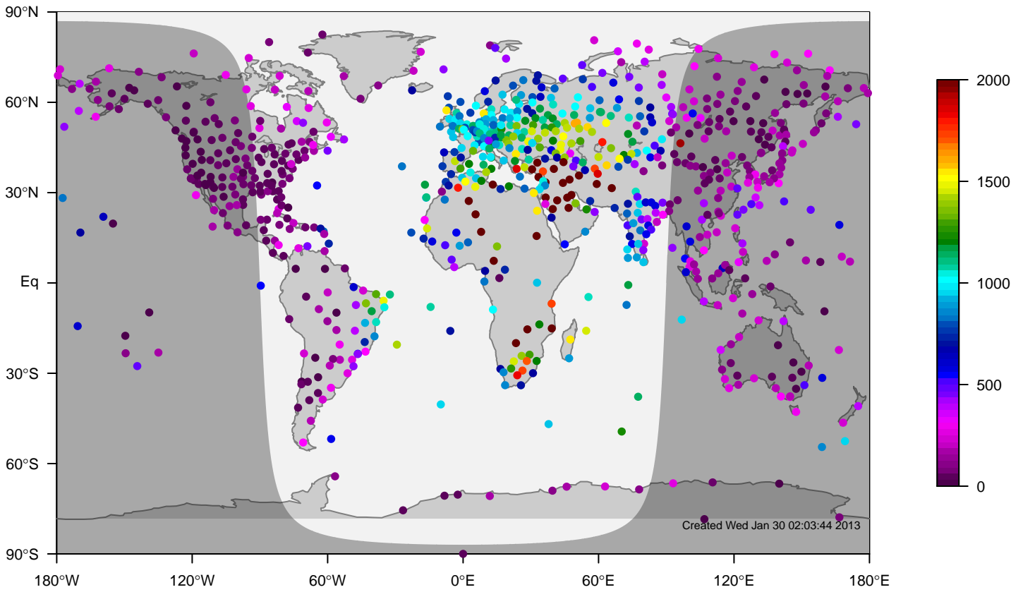
IGRA mixing height at 12UTC for September (1981–2006)
