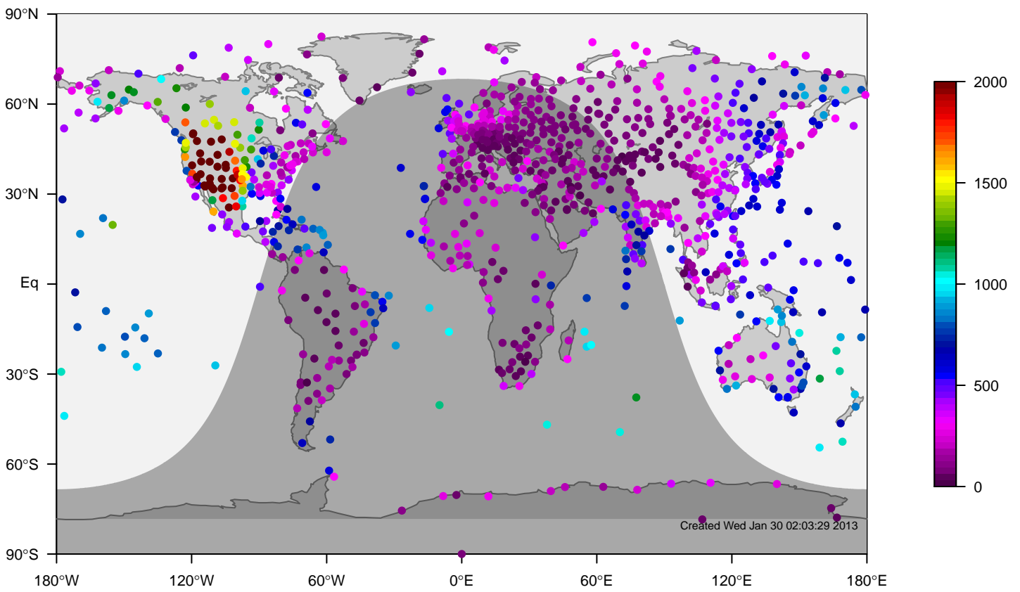
ERA-i mixing height at 0UTC for July (1981-2006)
