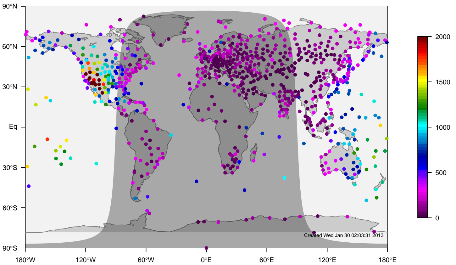
IGRA mixing height at 0UTC for September (1981–2006)
