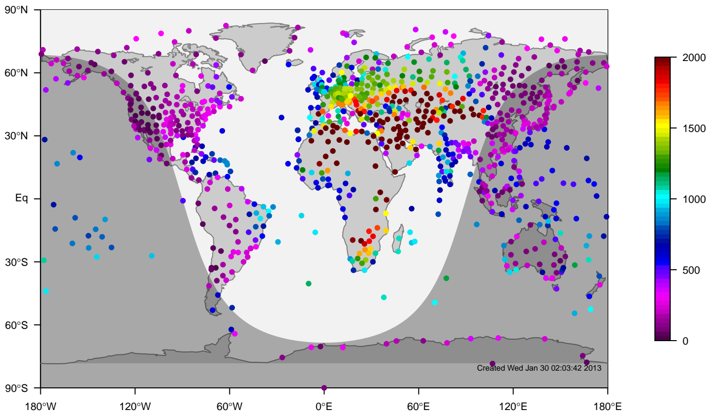
ERA-i mixing height at 12UTC for July (1981-2006)
