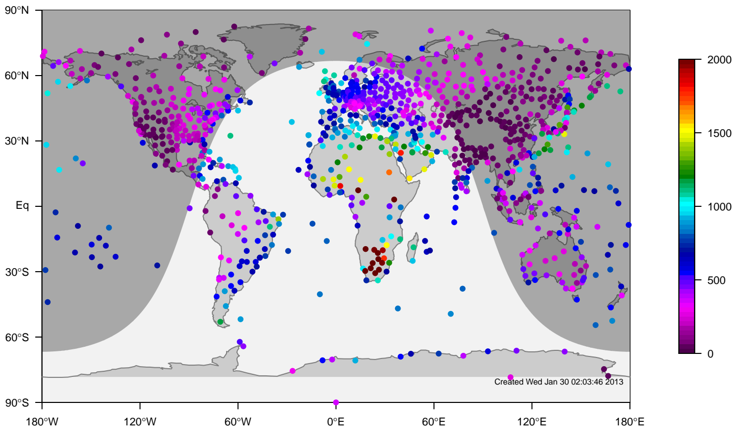
ERA-i mixing height at 12UTC for December (1981–2006)
