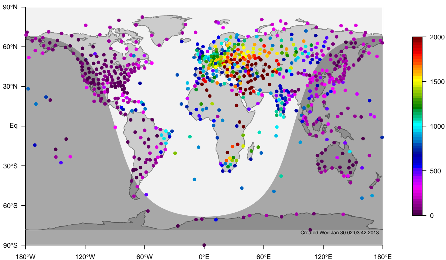
IGRA mixing height at 12UTC for July (1981-2006)
