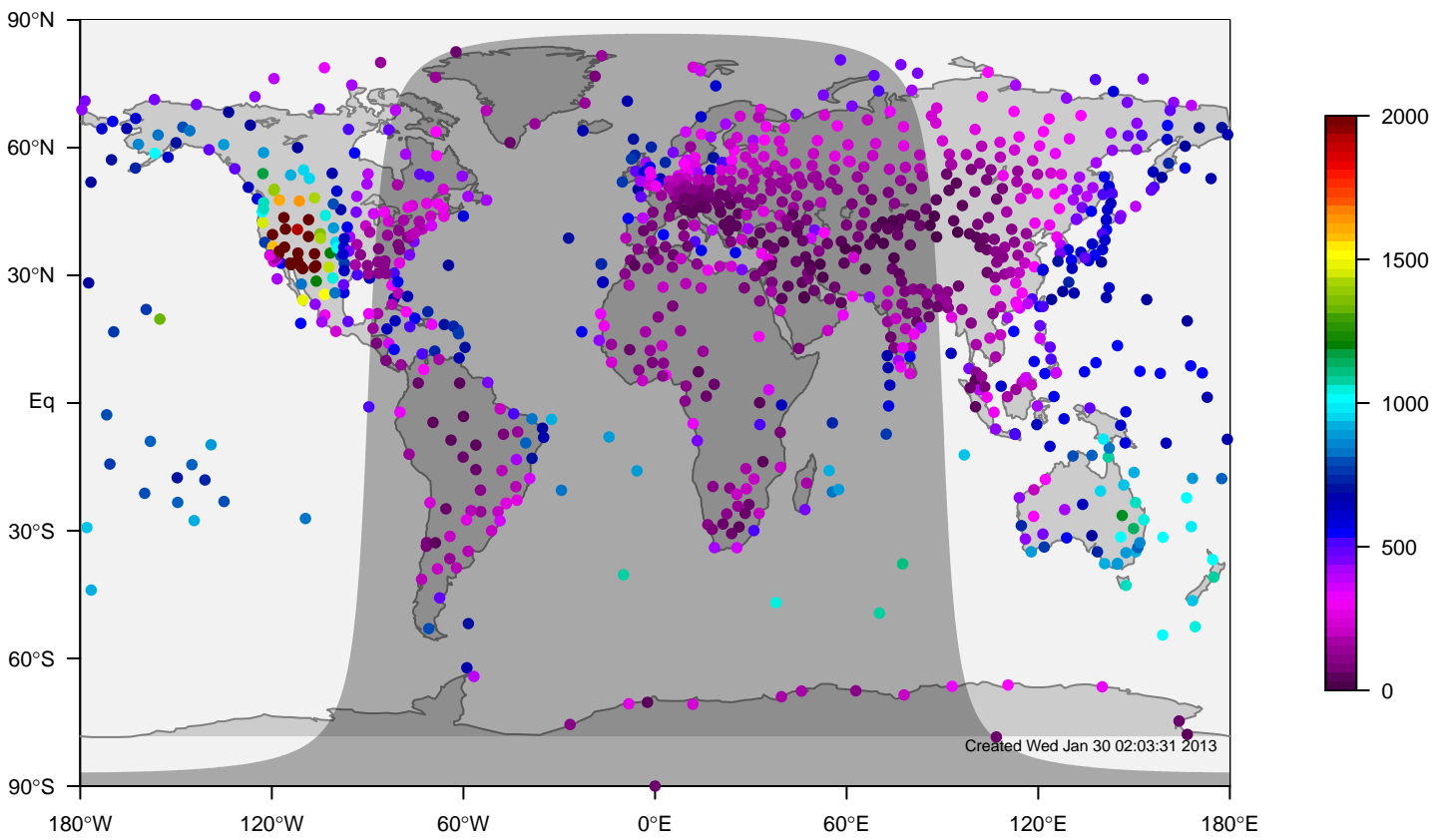
ERA-i mixing height at 0UTC for September (1981–2006)
