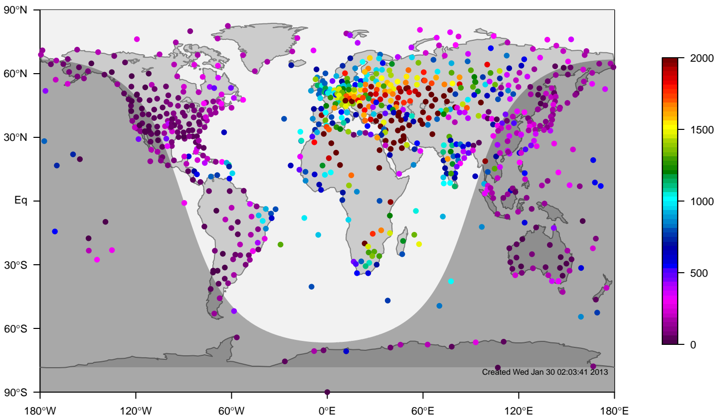
IGRA mixing height at 12UTC for June (1981-2006)
