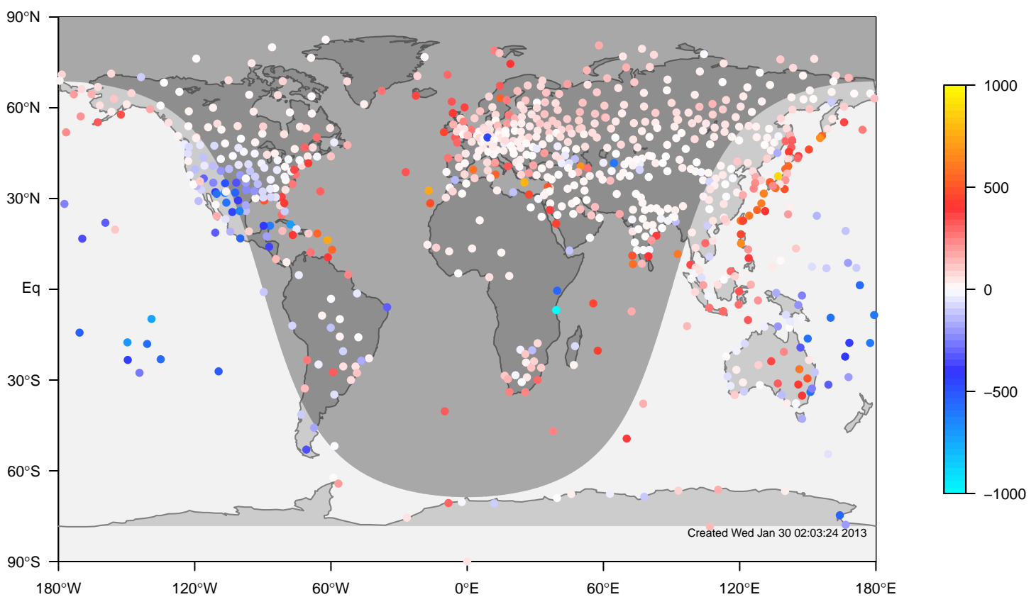
ERA-i minus IGRA bias at OUTC for January (1981–2006)
