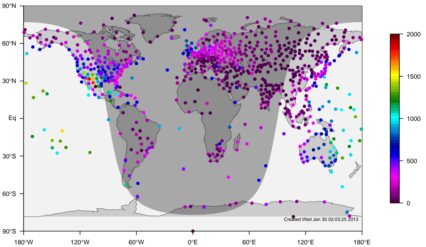
IGRA mixing height at OUTC for February (1981-2006)
