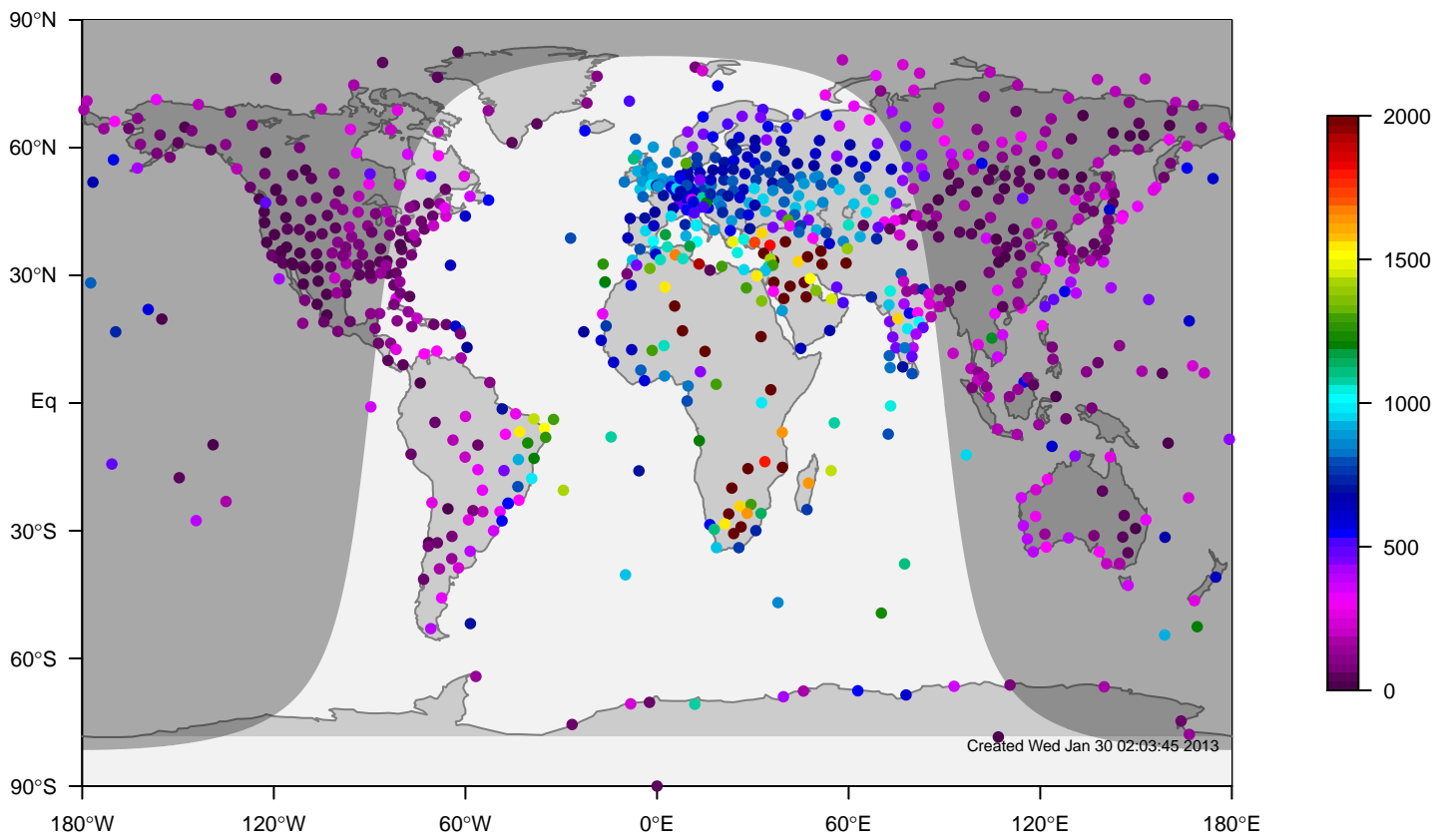
IGRA mixing height at 12UTC for October (1981-2006)
