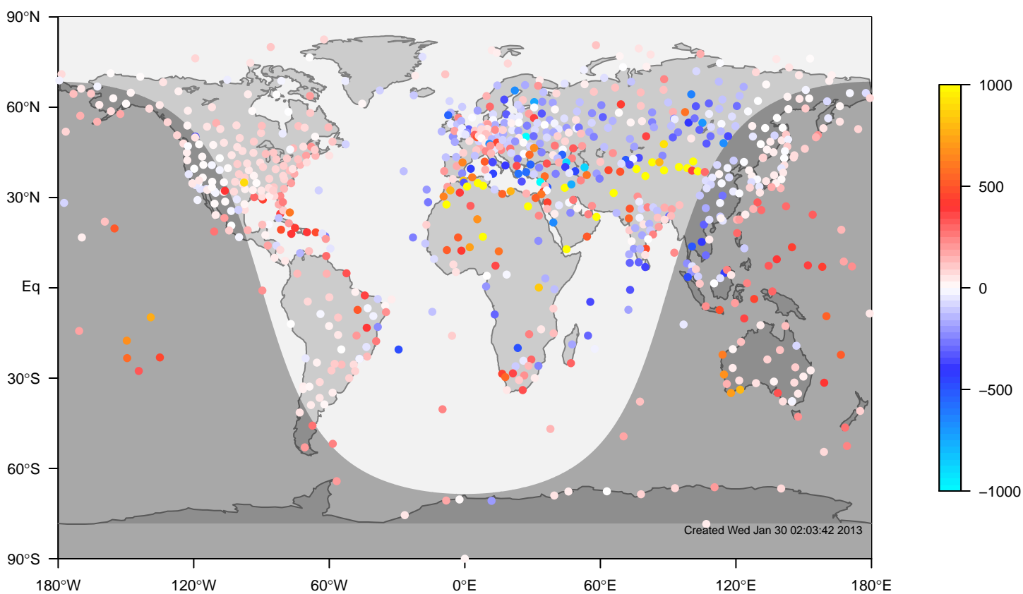
ERA-i minus IGRA bias at 12UTC for July (1981-2006)
