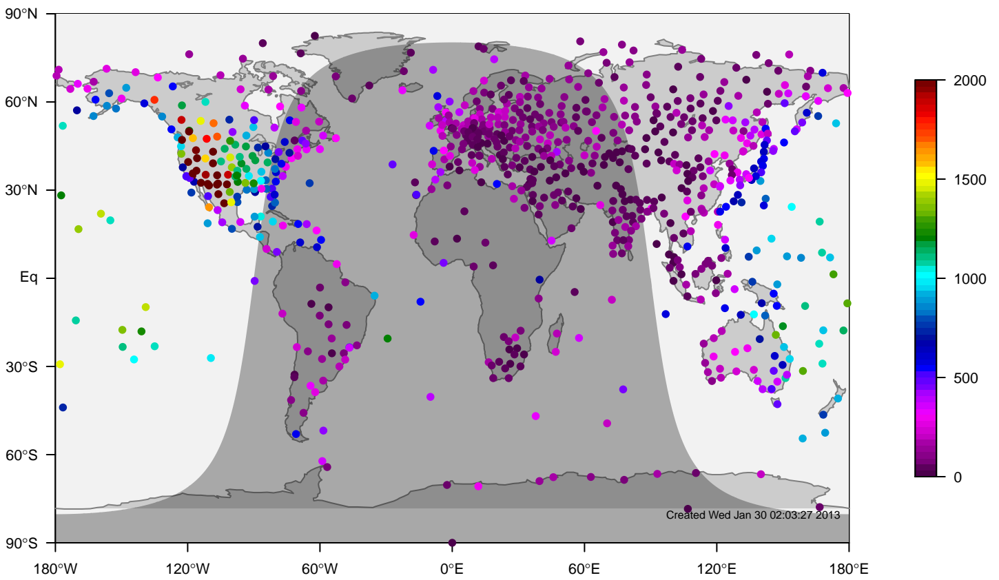
IGRA mixing height at 0UTC for April (1981-2006)
