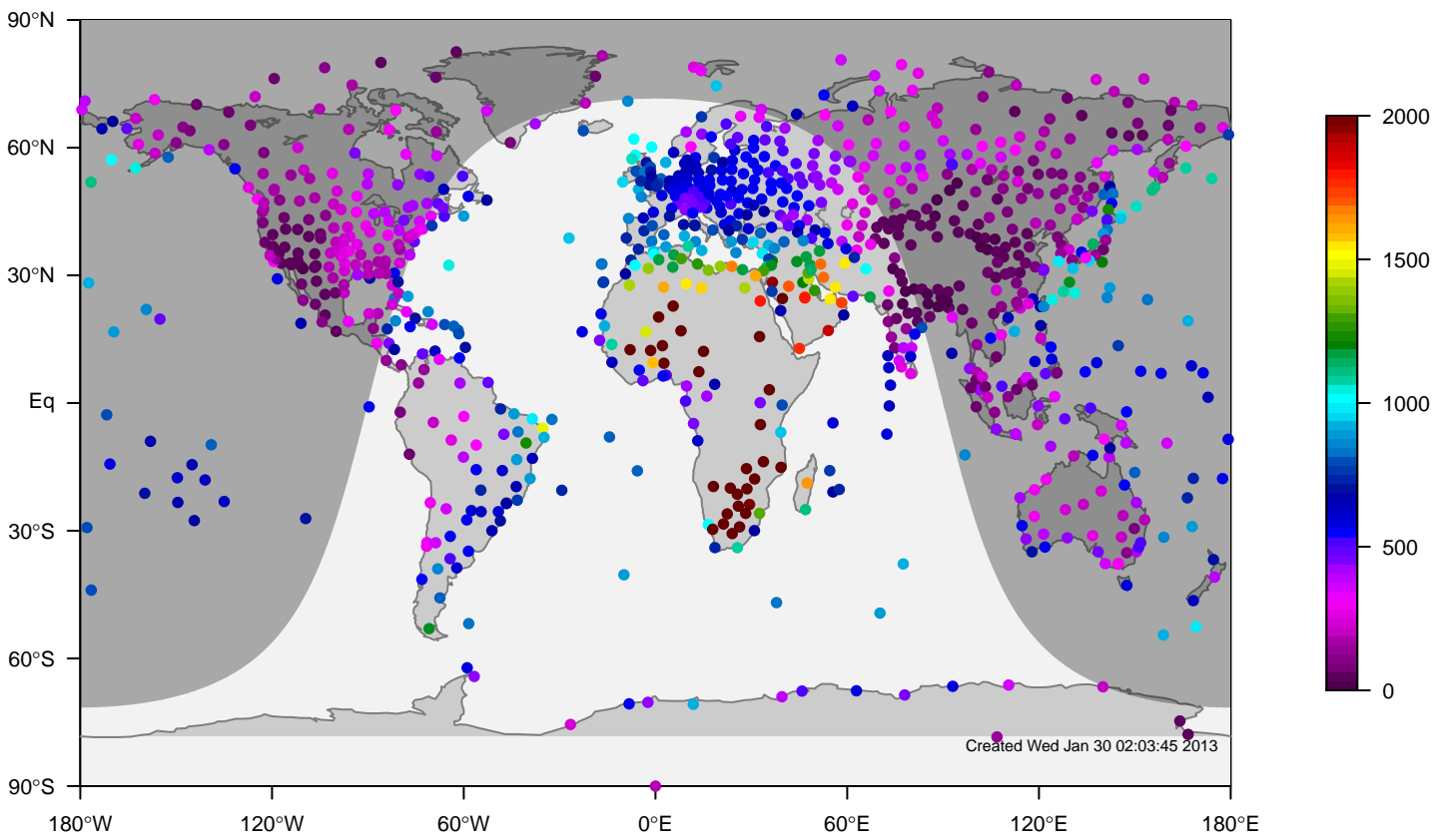
ERA-i mixing height at 12UTC for November (1981-2006)
