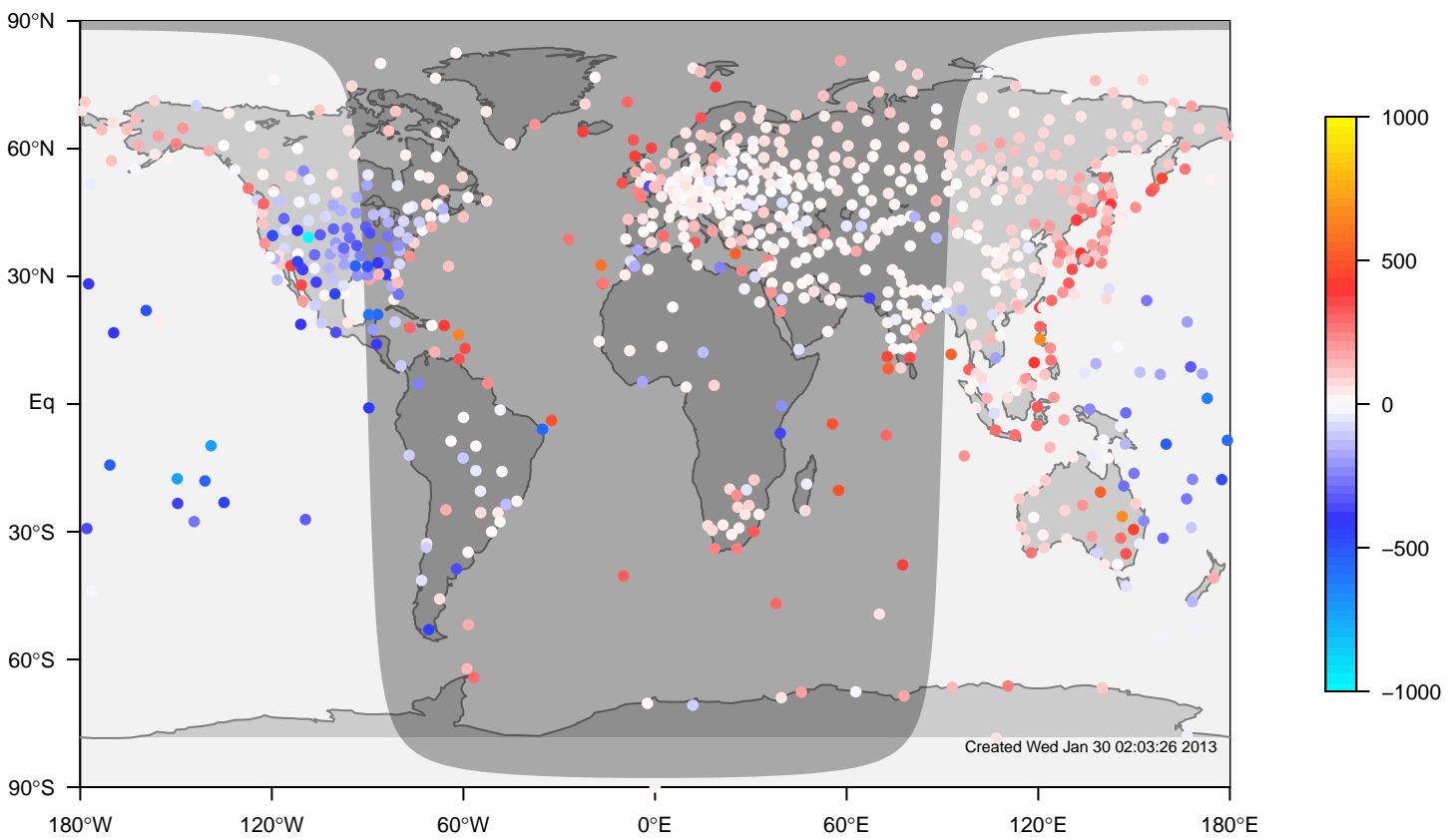
ERA-i minus IGRA bias at OUTC for March (1981–2006)
