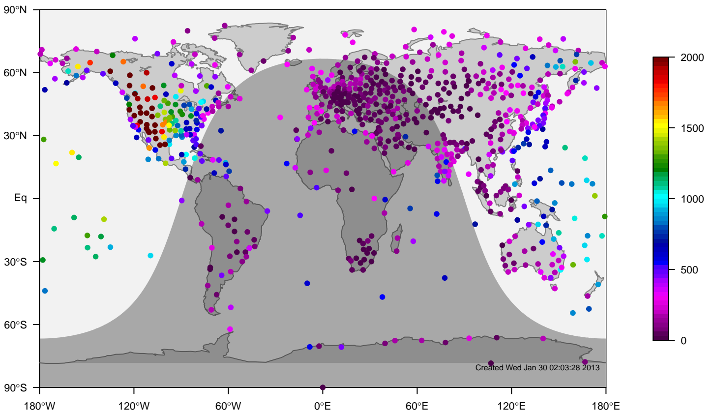
IGRA mixing height at 0UTC for June (1981-2006)
