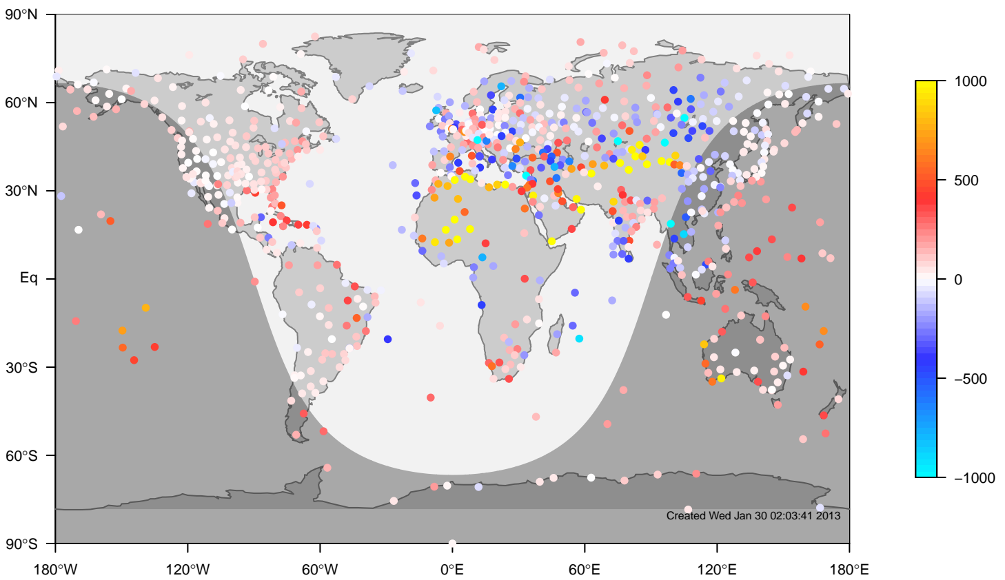
ERA-i minus IGRA bias at 12UTC for June (1981-2006)
