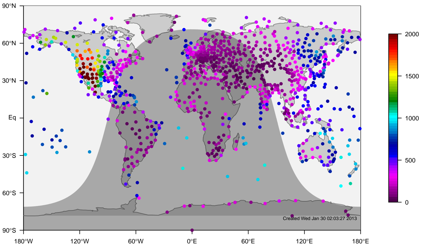
ERA-i mixing height at 0UTC for May (1981-2006)
