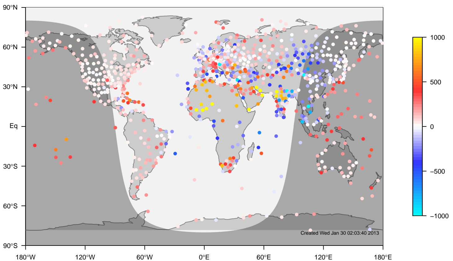
ERA-i minus IGRA bias at 12UTC for April (1981-2006)
