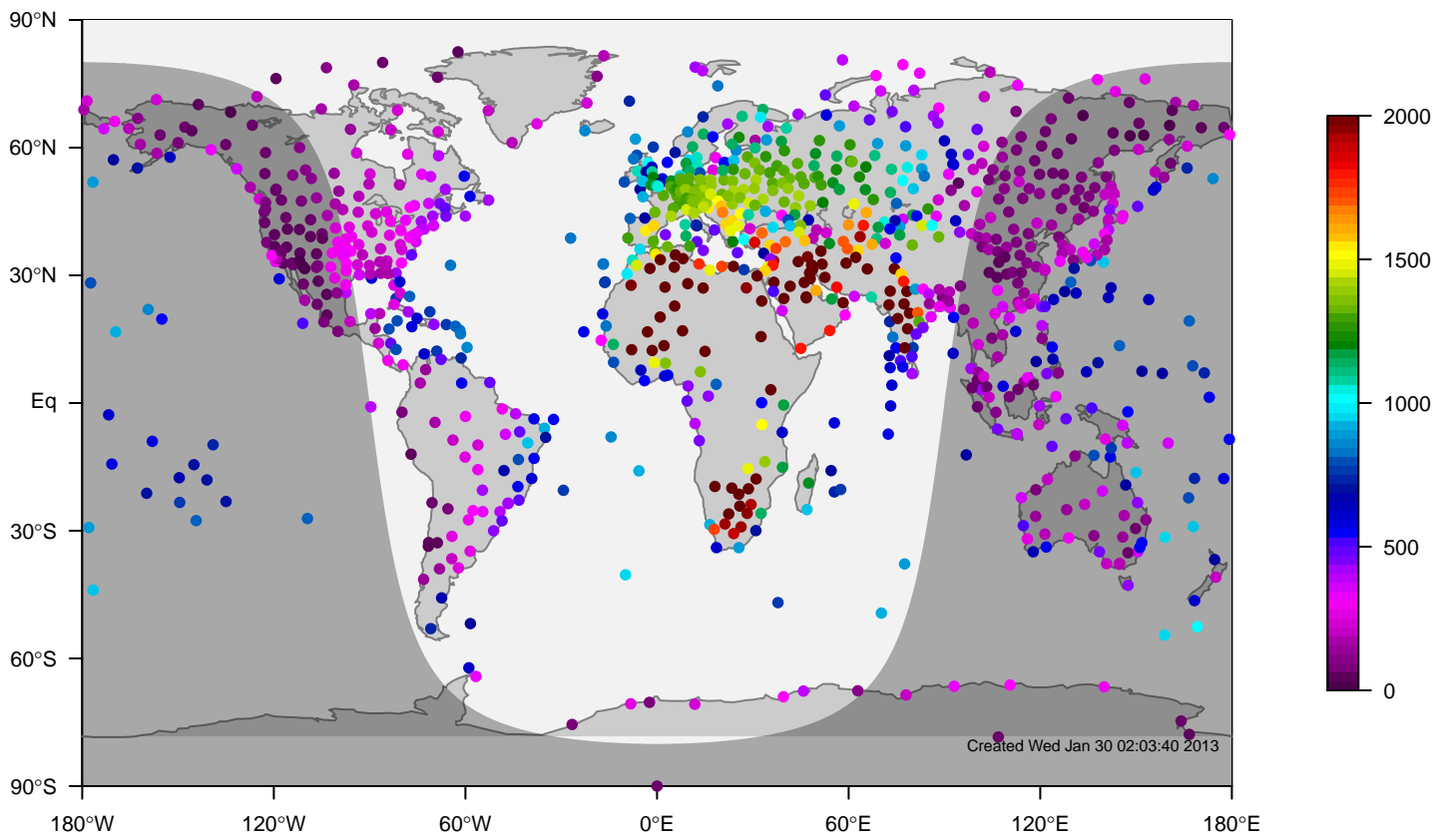
ERA-i mixing height at 12UTC for April (1981-2006)
