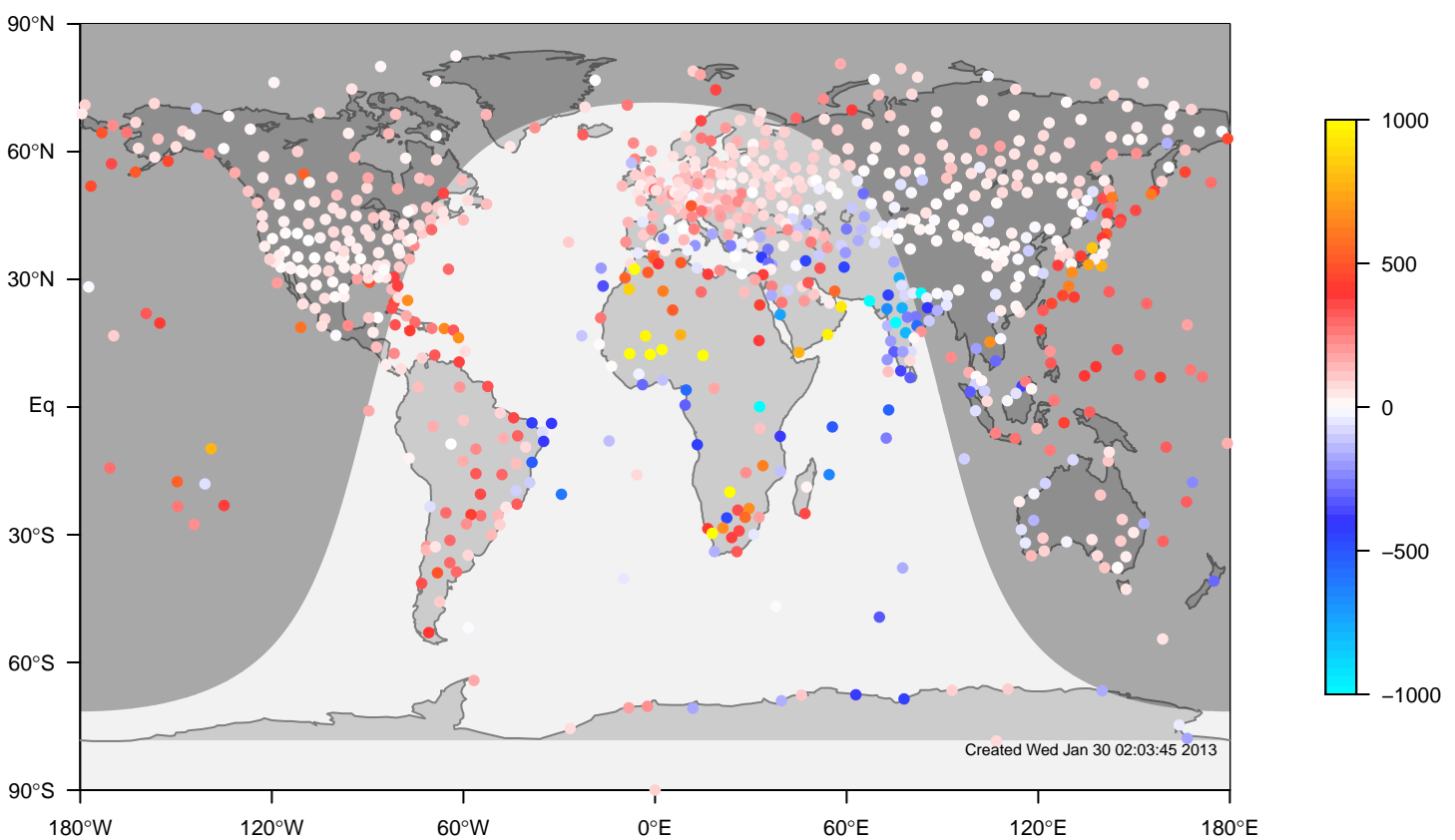
ERA-i minus IGRA bias at 12UTC for November (1981-2006)
