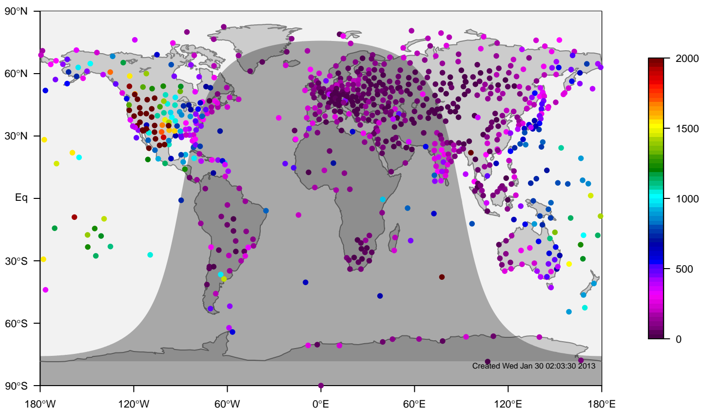
IGRA mixing height at 0UTC for August (1981-2006)
