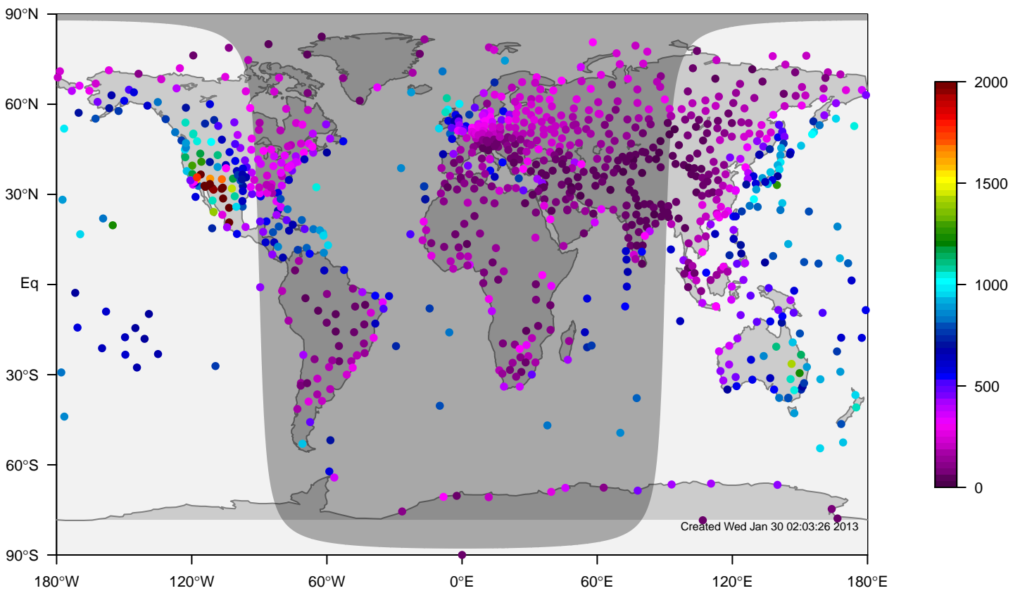
ERA-i mixing height at OUTC for March (1981–2006)
