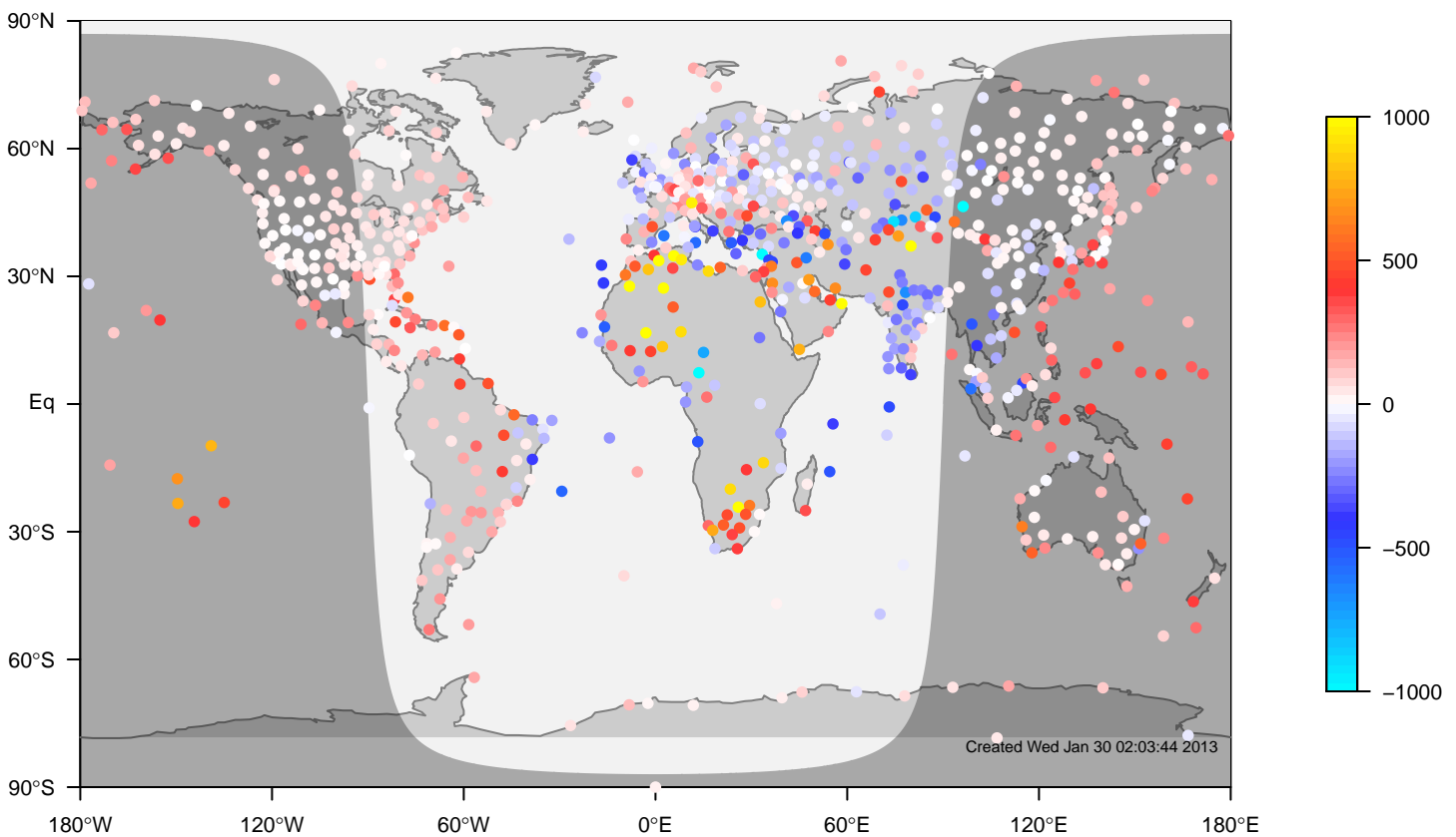
ERA-i minus IGRA bias at 12UTC for September (1981–2006)
