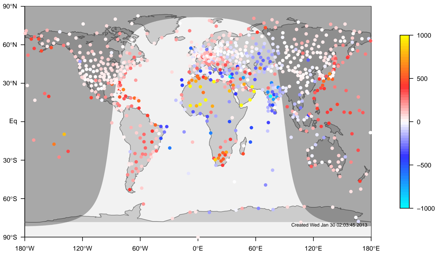
ERA-i minus IGRA bias at 12UTC for October (1981-2006)
