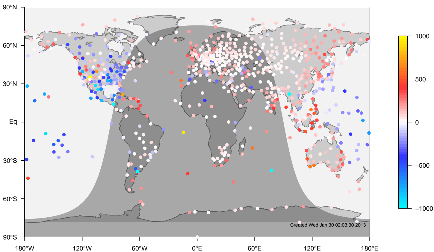
ERA-i minus IGRA bias at 0UTC for August (1981-2006)
