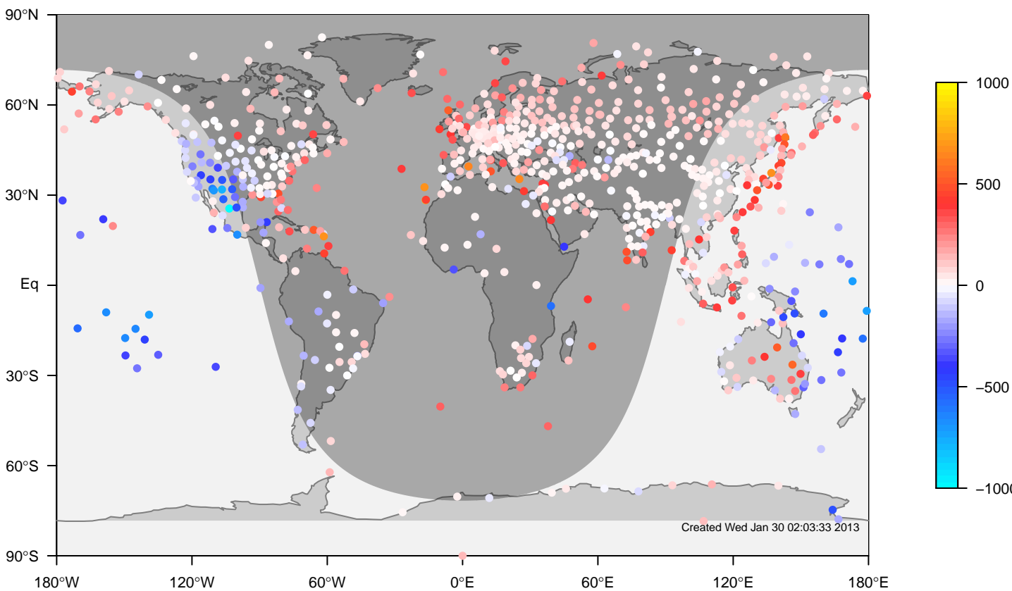
ERA-i minus IGRA bias at 0UTC for November (1981-2006)
