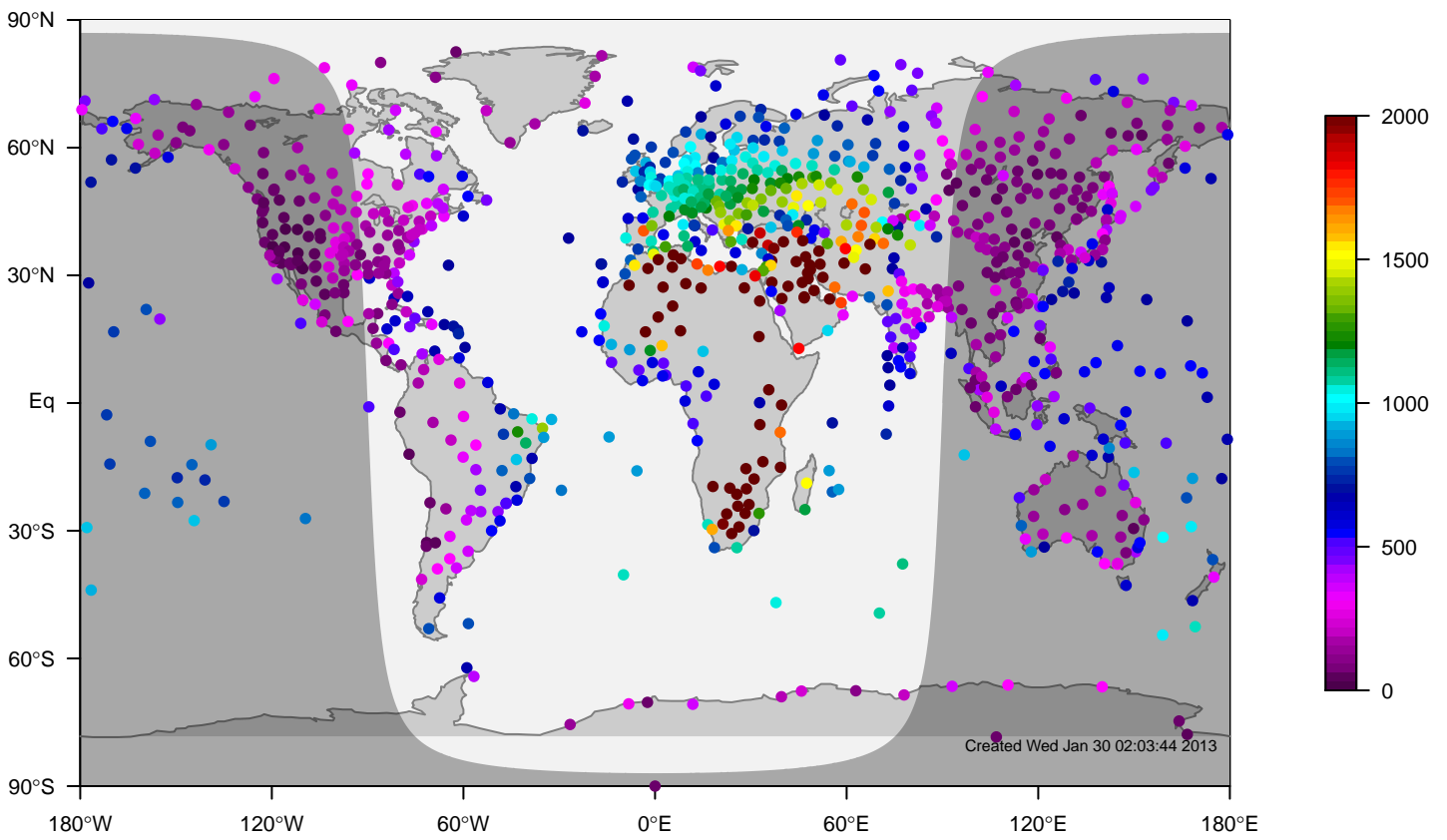
ERA-i mixing height at 12UTC for September (1981–2006)
