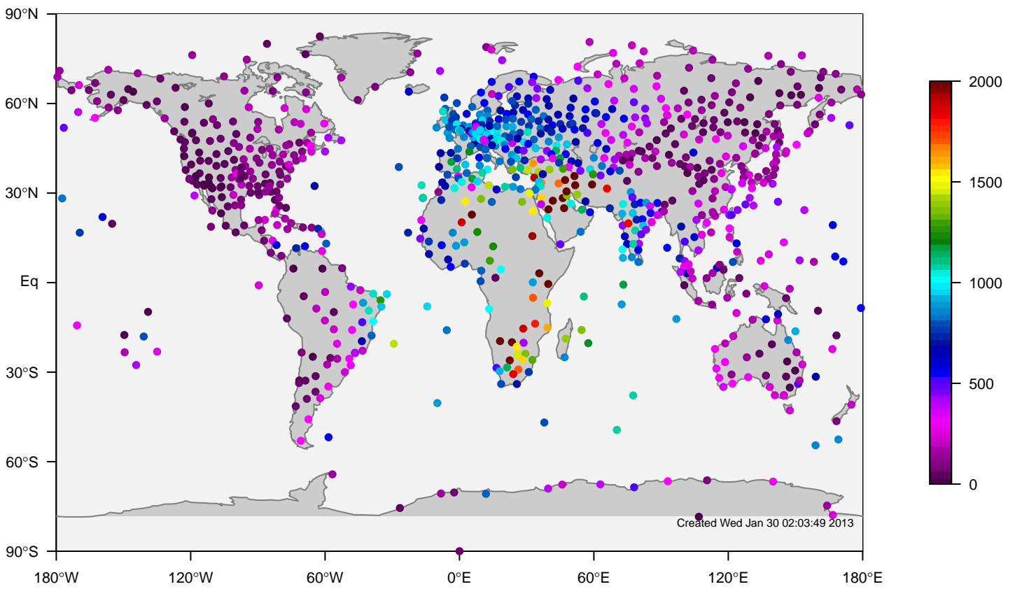
IGRA all-season mixing height at 12UTC (1981-2006)
