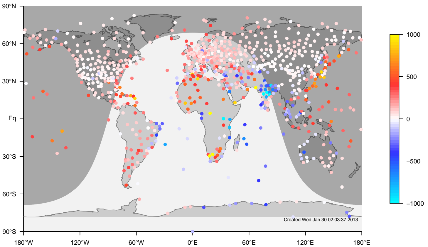
ERA-i minus IGRA bias at 12UTC for January (1981-2006)
