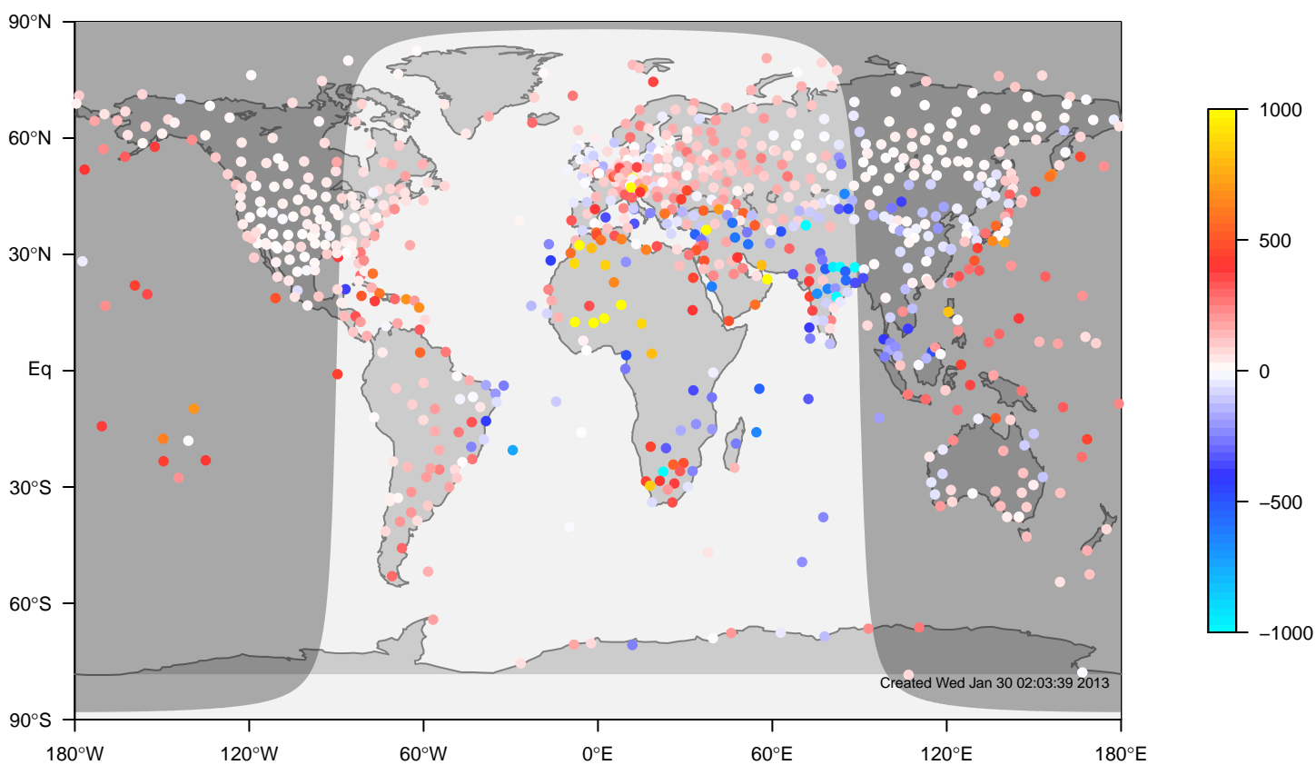
ERA-i minus IGRA bias at 12UTC for March (1981-2006)
