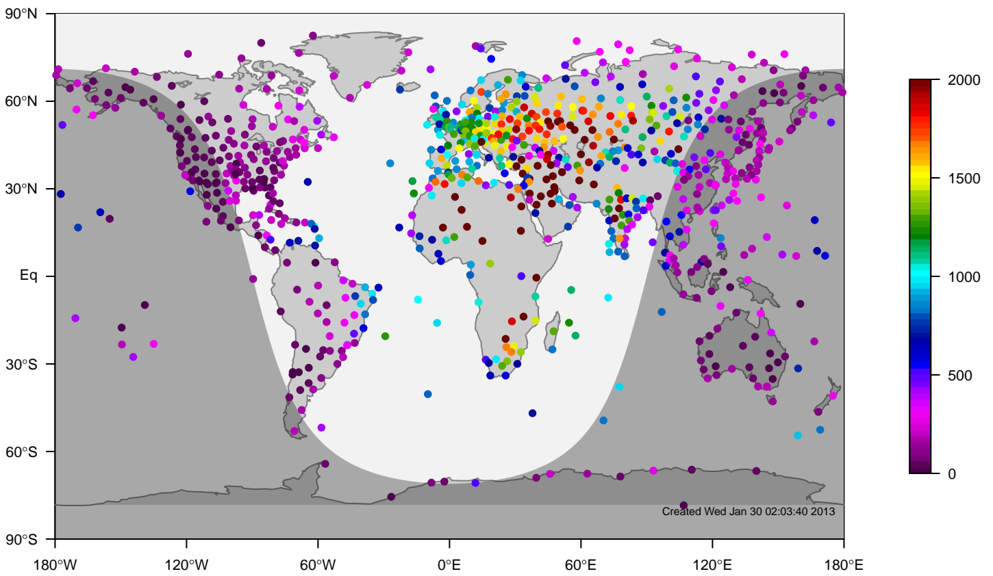
IGRA mixing height at 12UTC for May (1981-2006)
