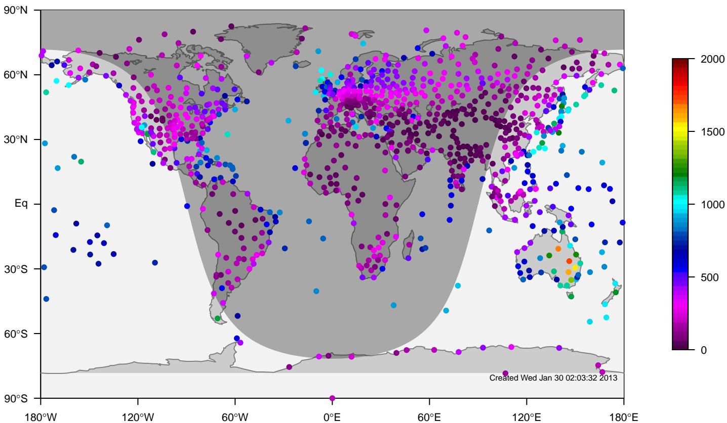
ERA-i mixing height at 0UTC for November (1981-2006)
