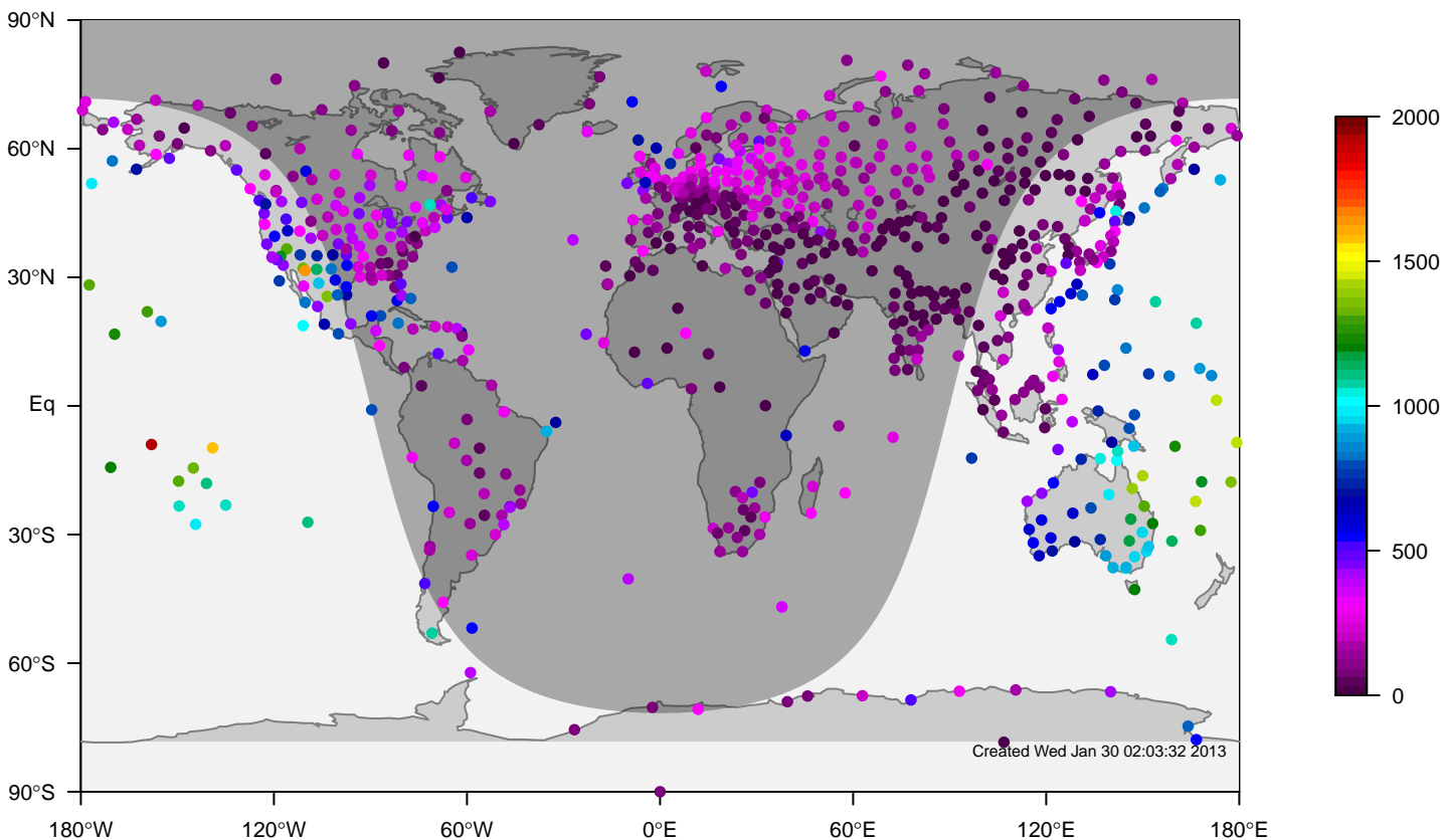
IGRA mixing height at 0UTC for November (1981-2006)
