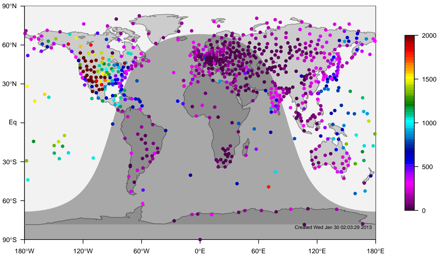
IGRA mixing height at 0UTC for July (1981-2006)
