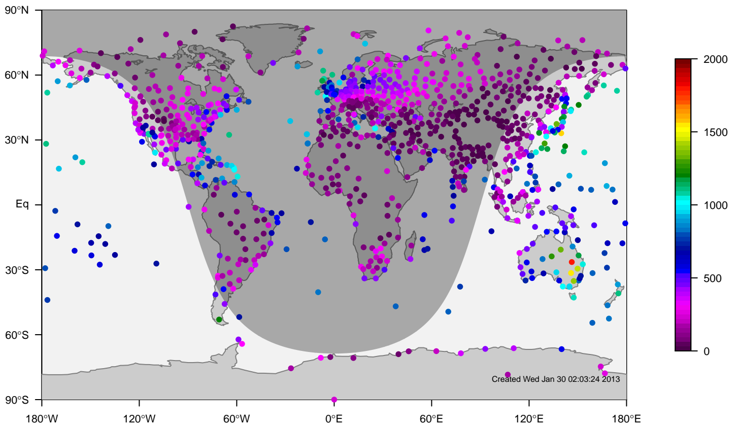
ERA-i mixing height at OUTC for January (1981–2006)
