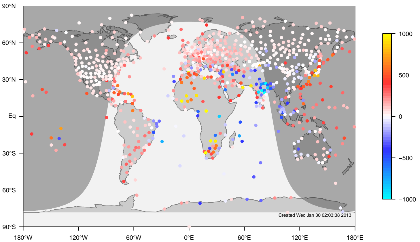
ERA-i minus IGRA bias at 12UTC for February (1981-2006)
