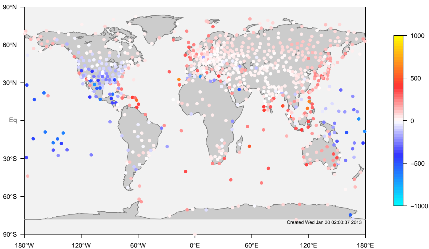
ERA-i minus IGRA all-season bias at OUTC (1981 - 2006)
