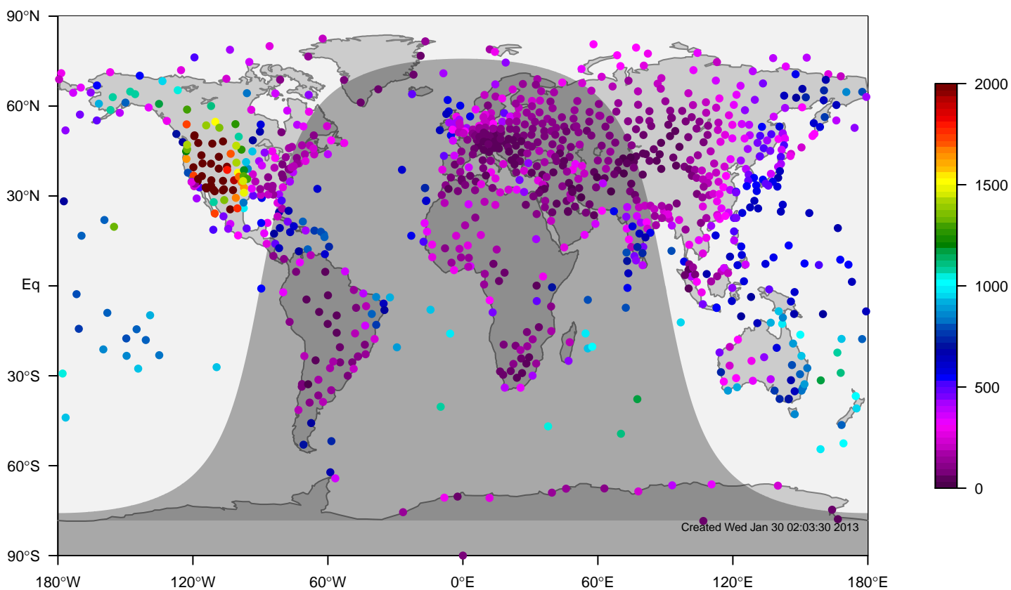
ERA-i mixing height at 0UTC for August (1981-2006)
