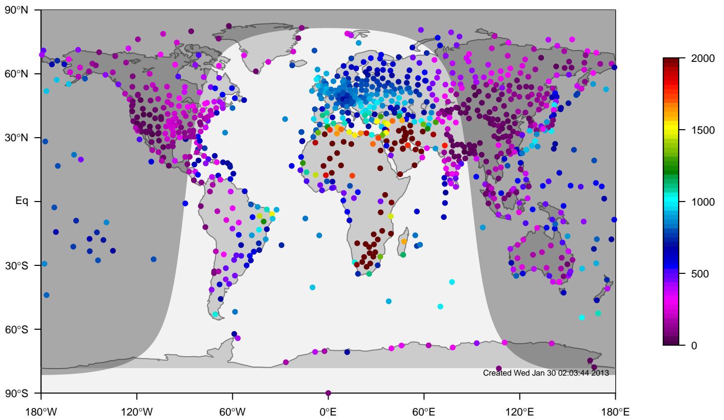
ERA-i mixing height at 12UTC for October (1981-2006)
