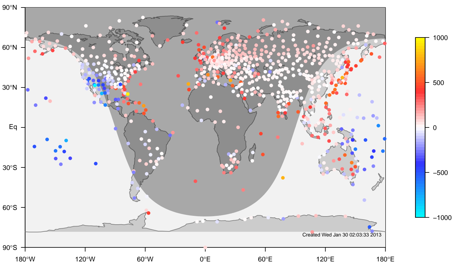
ERA-i minus IGRA bias at 0UTC for December (1981-2006)
