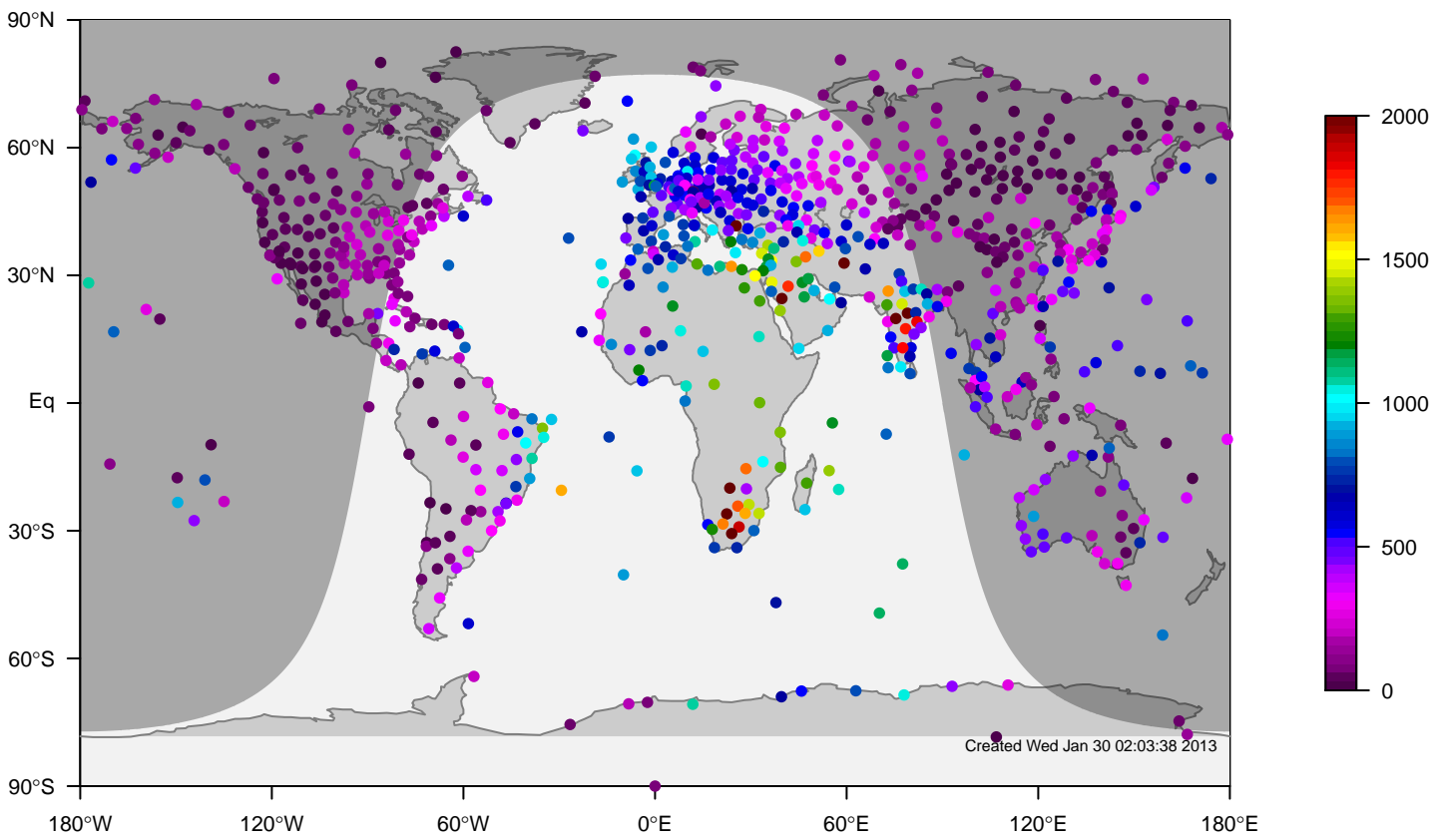
IGRA mixing height at 12UTC for February (1981-2006)
