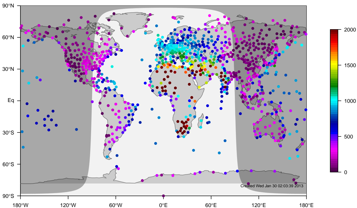
ERA-i mixing height at 12UTC for March (1981-2006)
