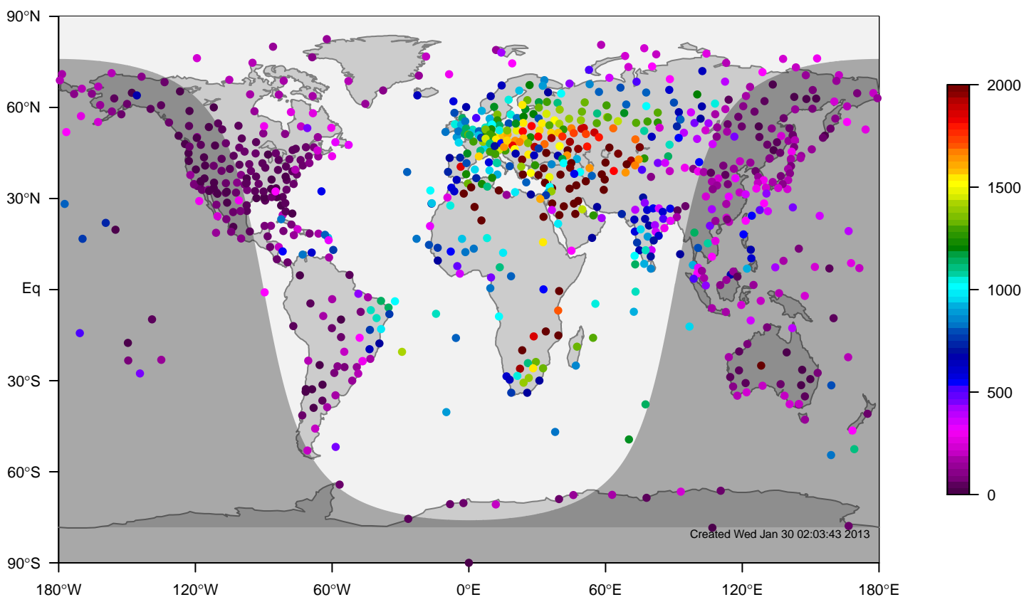
IGRA mixing height at 12UTC for August (1981-2006)
