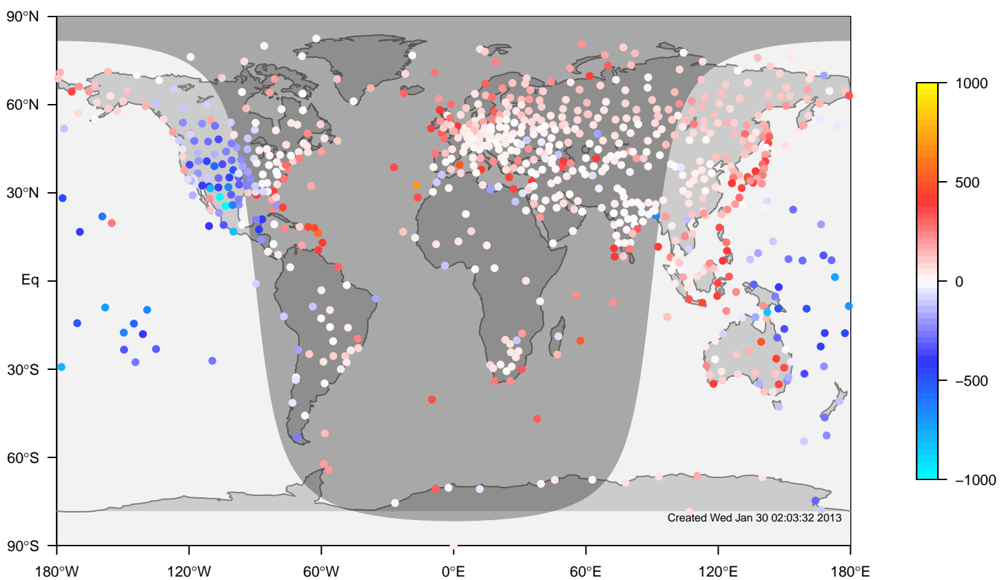
ERA-i minus IGRA bias at 0UTC for October (1981-2006)
