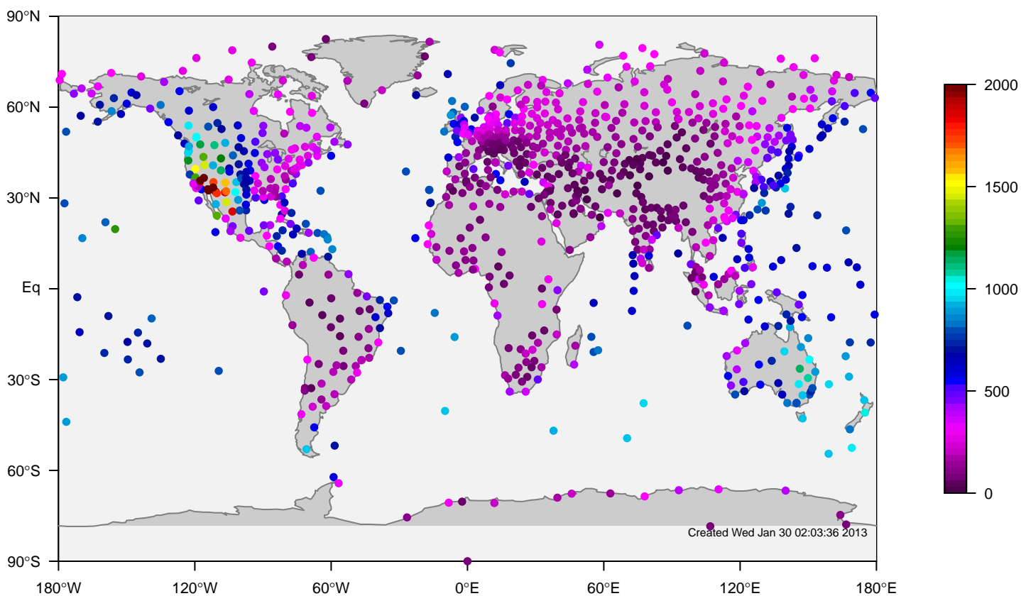
ERA-i all-season mixing height at OUTC (1981-2006)
