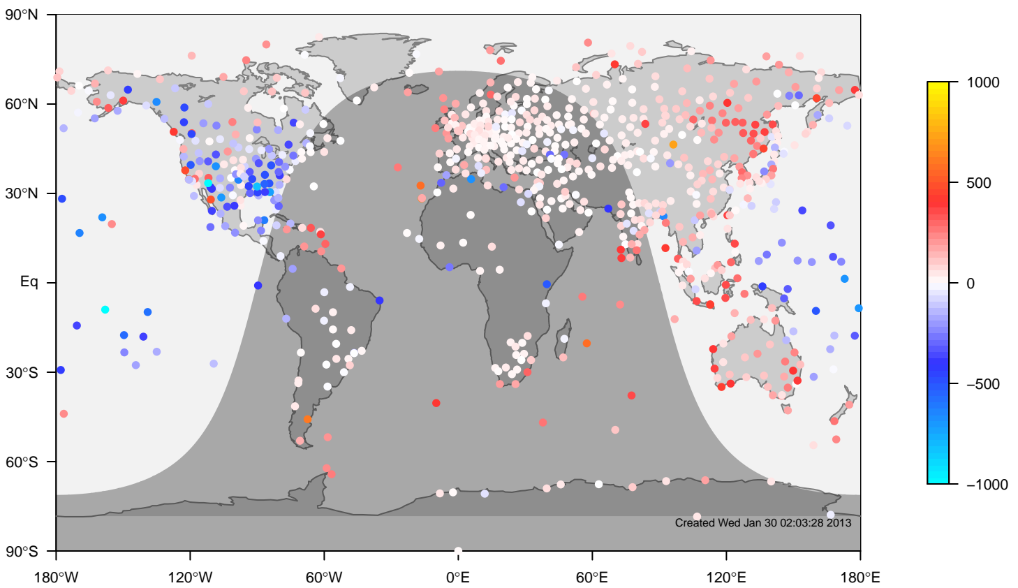
ERA-i minus IGRA bias at 0UTC for May (1981-2006)
