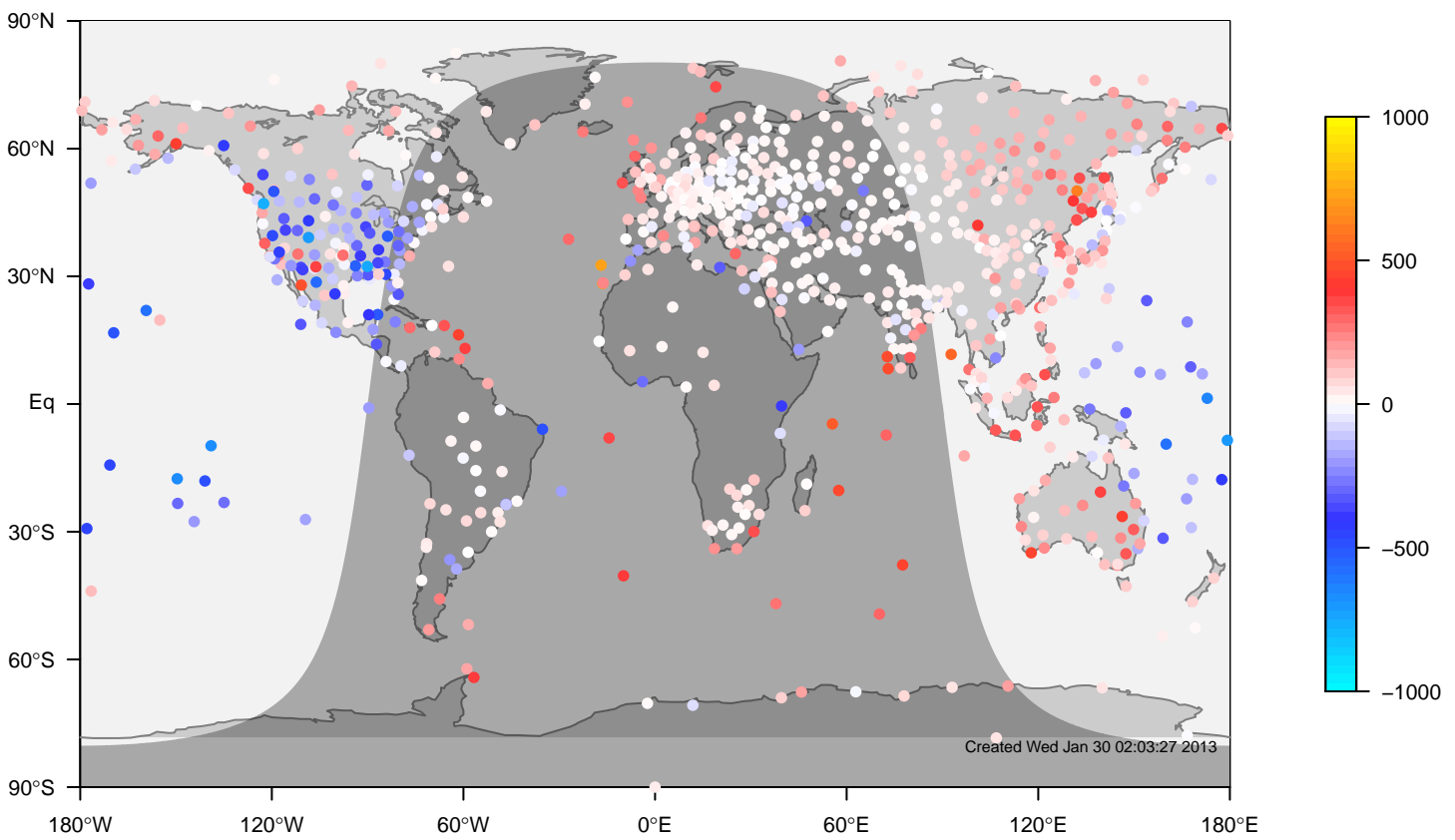
ERA-i minus IGRA bias at 0UTC for April (1981-2006)
