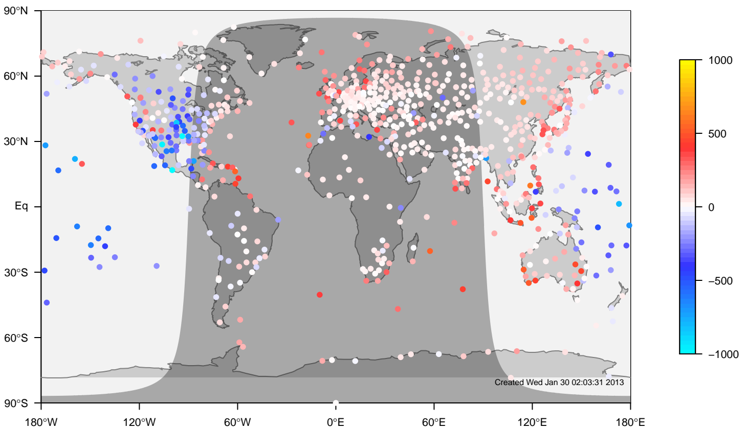
ERA-i minus IGRA bias at 0UTC for September (1981–2006)
