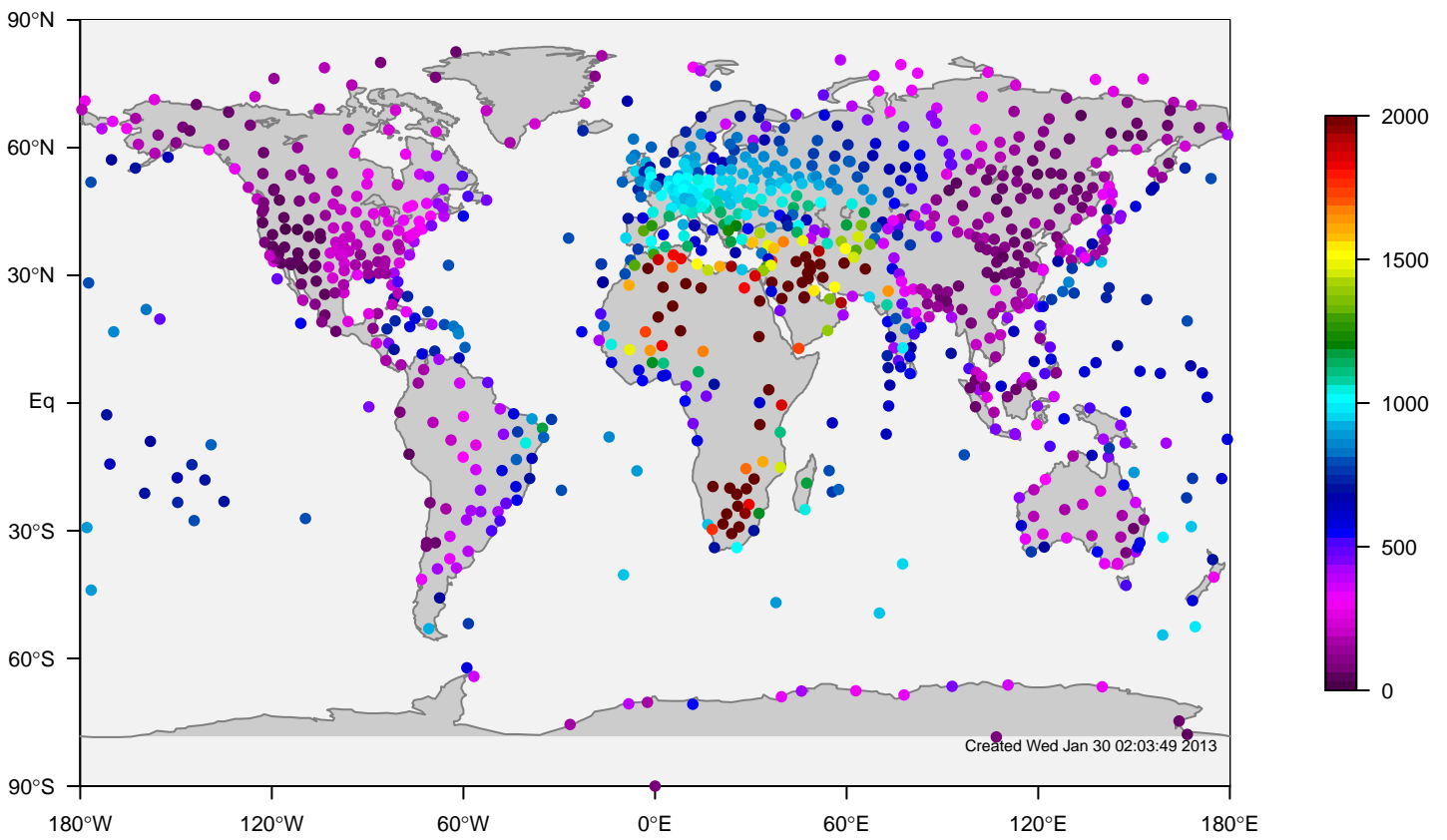
ERA-i all-season mixing height at 12UTC (1981-2006)
