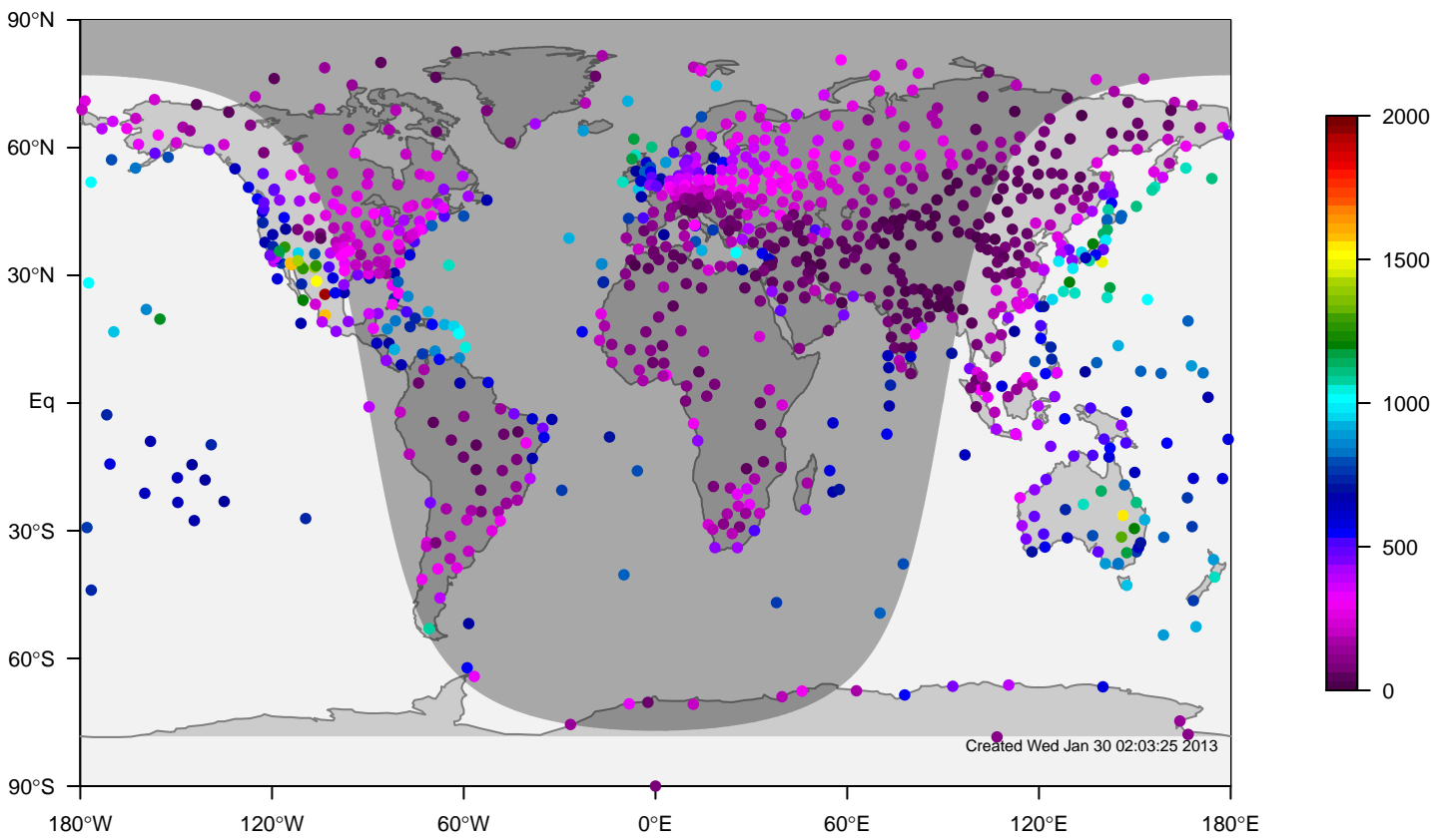
ERA-i mixing height at OUTC for February (1981-2006)
