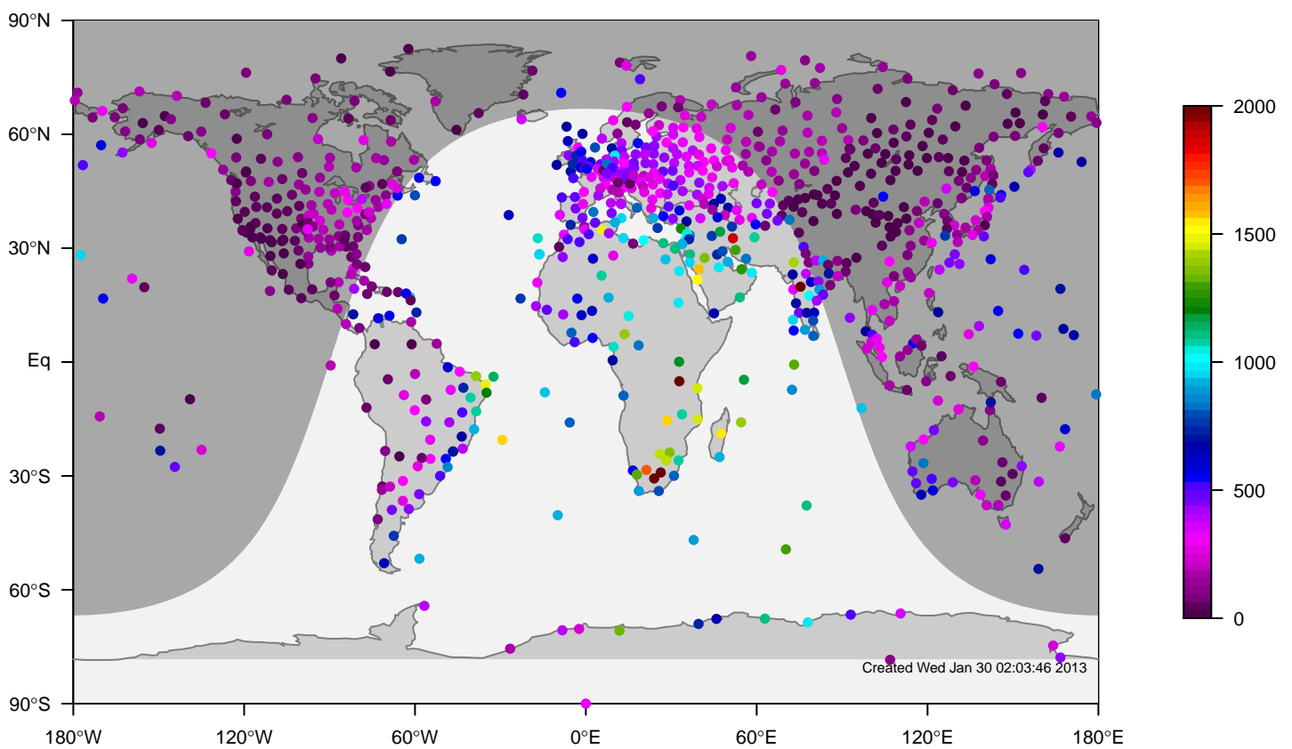
IGRA mixing height at 12UTC for December (1981–2006)
