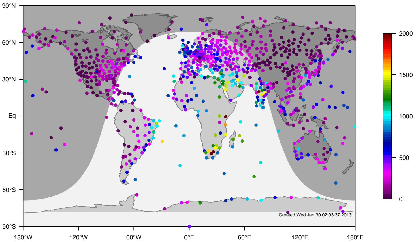
IGRA mixing height at 12UTC for January (1981-2006)
