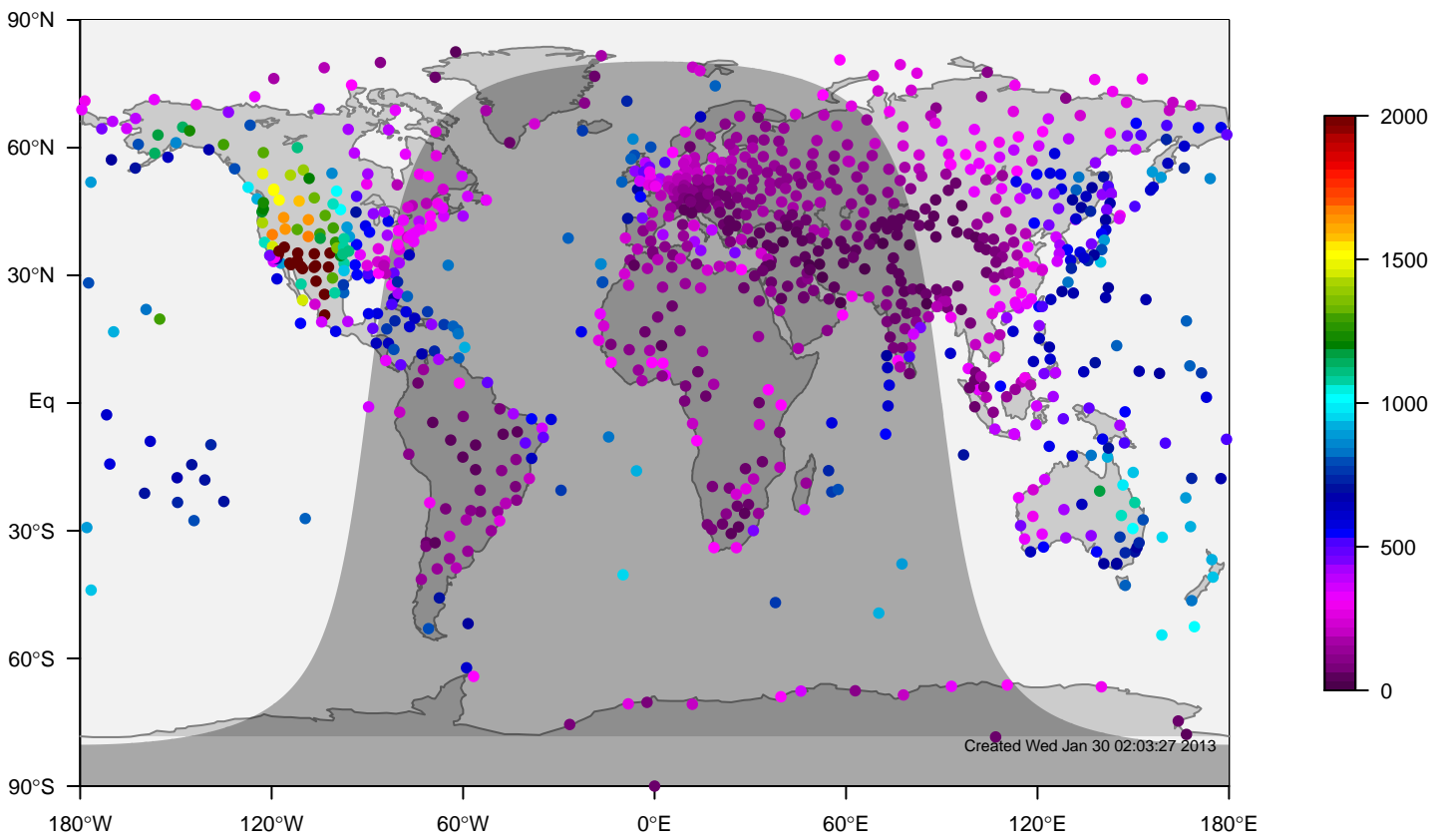
ERA-i mixing height at 0UTC for April (1981-2006)
