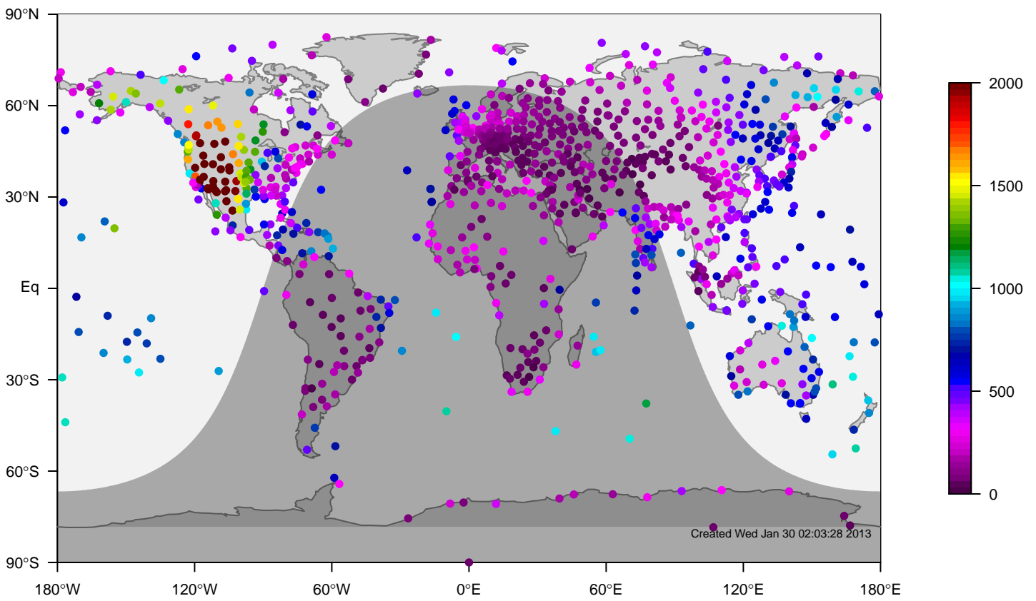
ERA-i mixing height at 0UTC for June (1981-2006)
