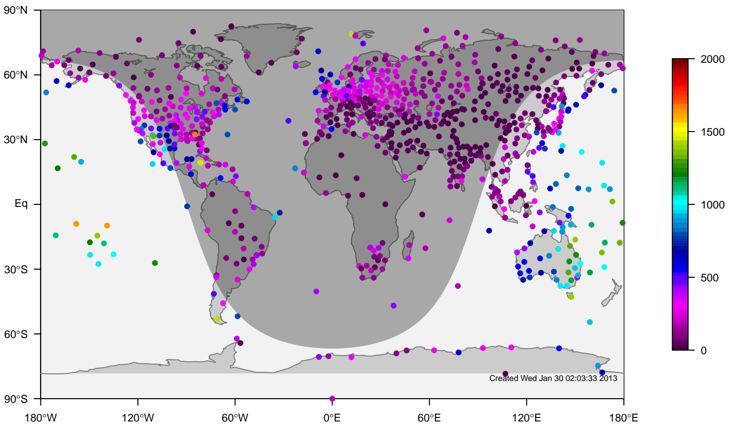
IGRA mixing height at 0UTC for December (1981-2006)
