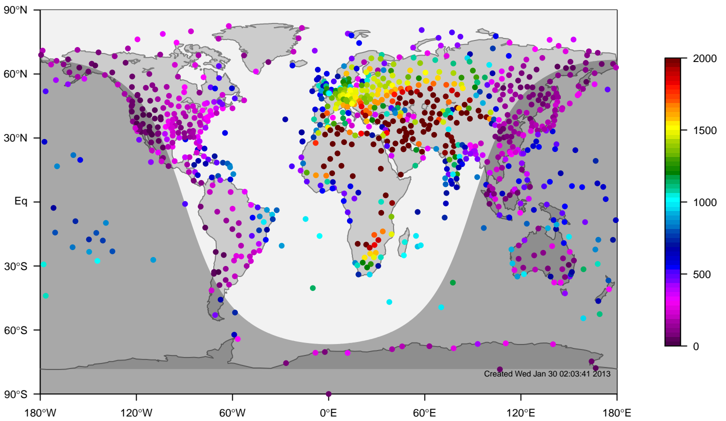
ERA-i mixing height at 12UTC for June (1981-2006)
