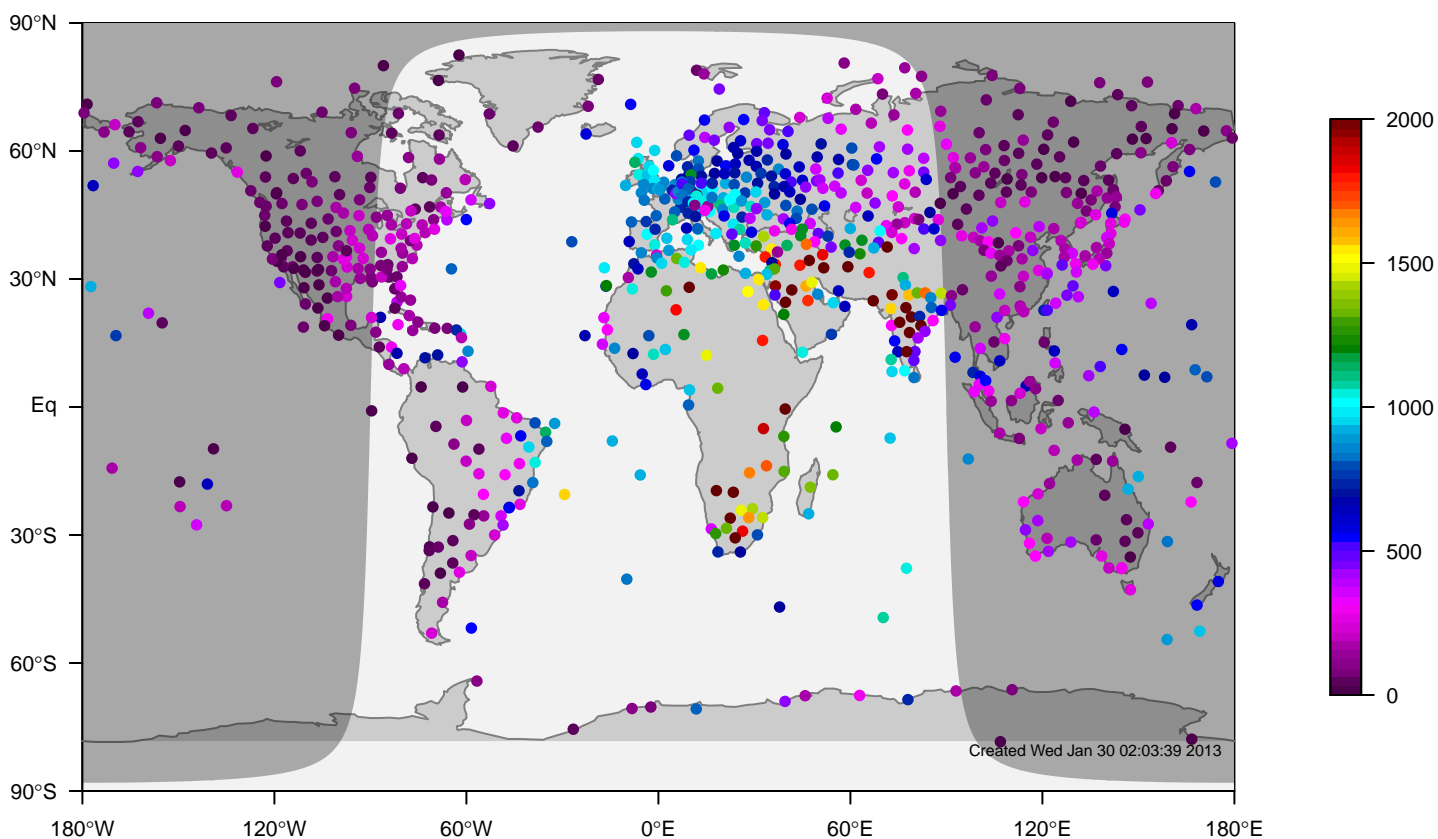
IGRA mixing height at 12UTC for March (1981-2006)
