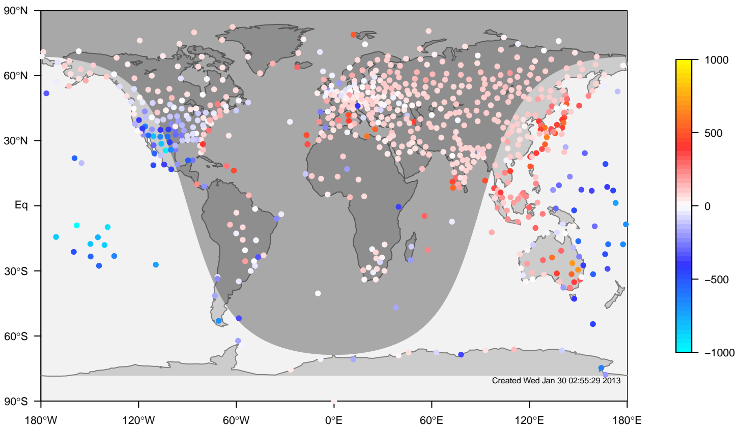
internal-TM5-ei-glb3x2 minus IGRA bias at 0UTC for January (1995-2011)
