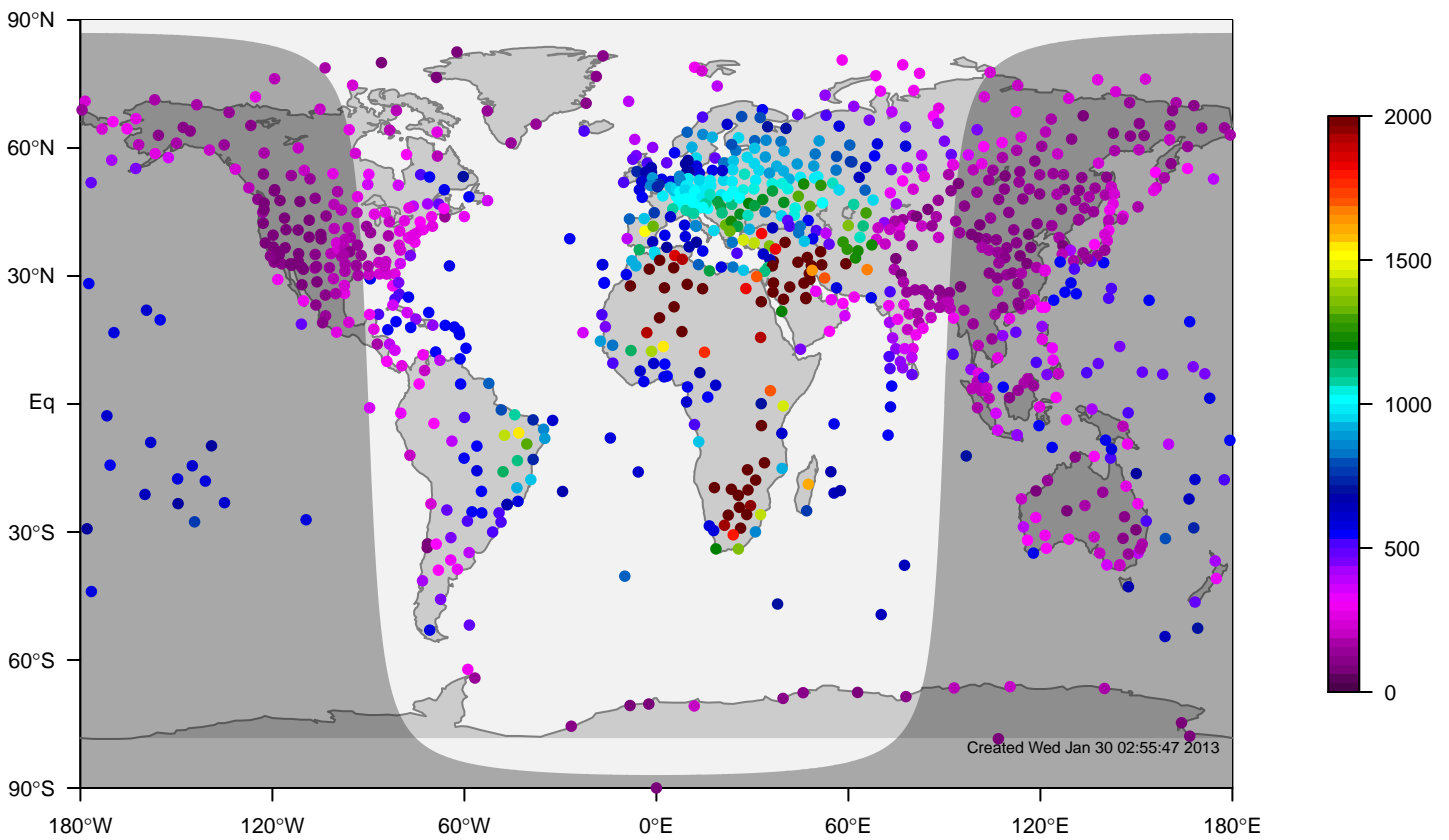
internal-TM5-ei-glb3x2 mixing height at 12UTC for September (1995-2011)
