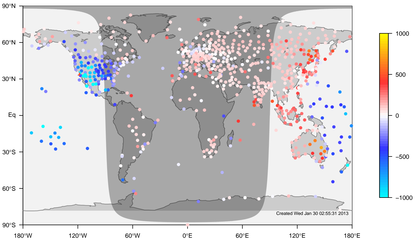
internal-TM5-ei-glb3x2 minus IGRA bias at 0UTC for March (1995-2011)
