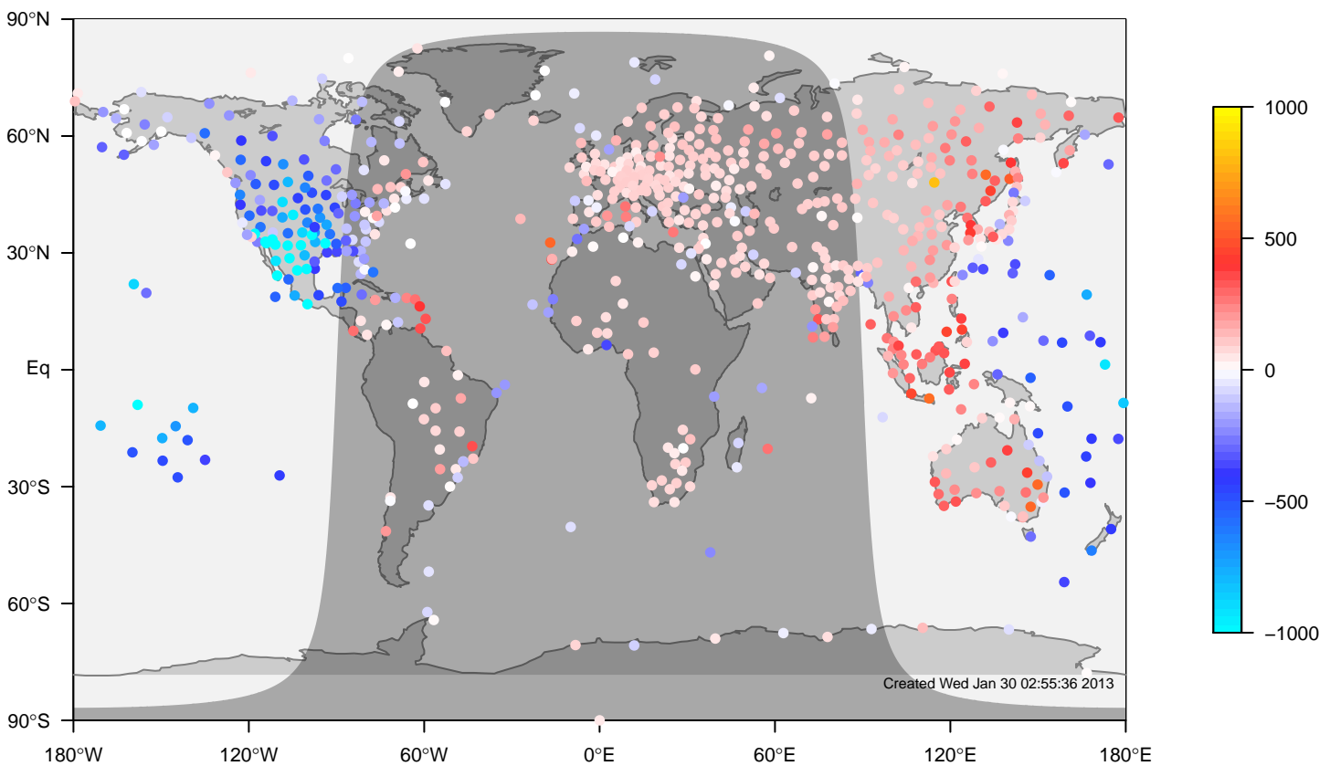
internal-TM5-ei-glb3x2 minus IGRA bias at 0UTC for September (1995-2011)
