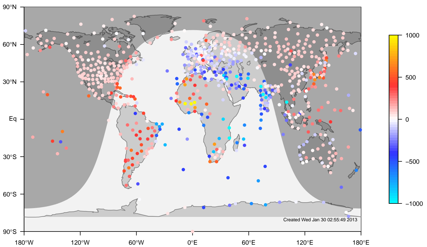
internal-TM5-ei-glb3x2 minus IGRA bias at 12UTC for November (1995-2011)
