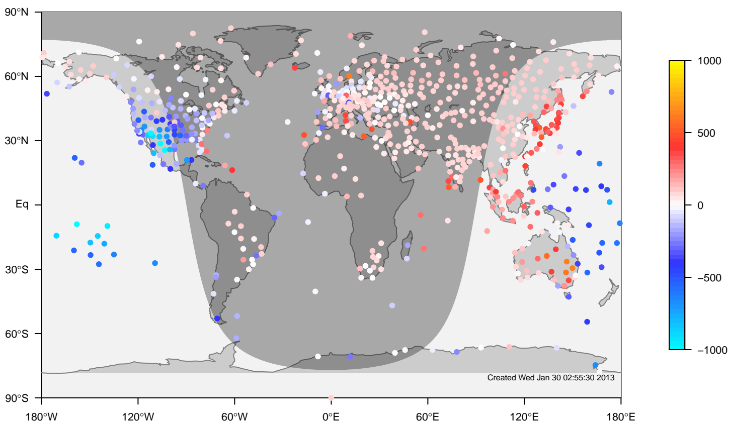
internal-TM5-ei-glb3x2 minus IGRA bias at 0UTC for February (1995-2011)
