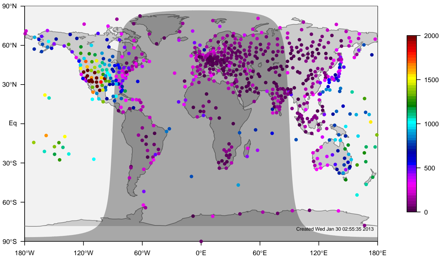
IGRA mixing height at 0UTC for September (1995-2011)
