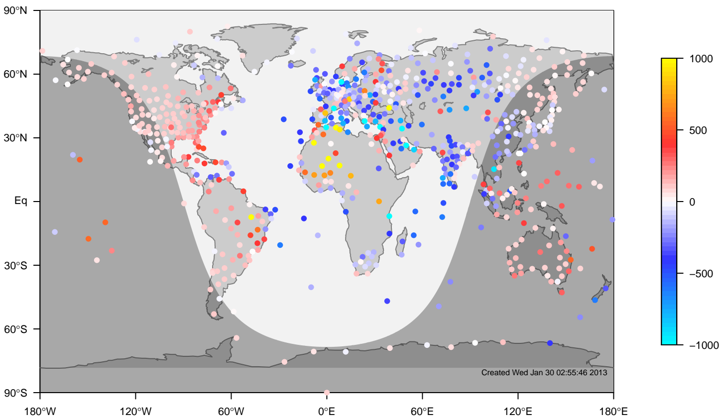
internal-TM5-ei-glb3x2 minus IGRA bias at 12UTC for July (1995-2011)
