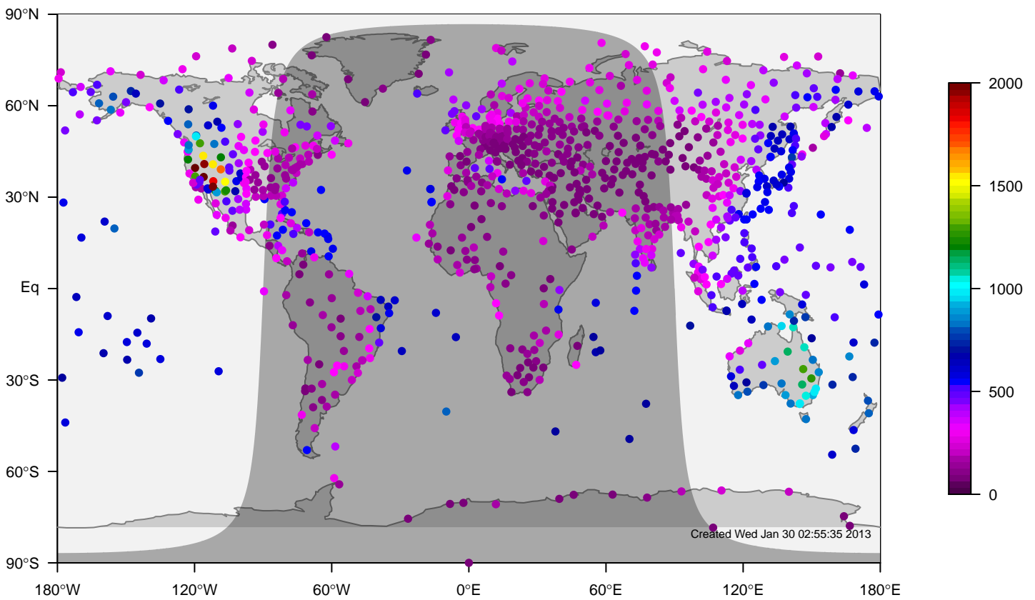
internal-TM5-ei-glb3x2 mixing height at 0UTC for September (1995-2011)
