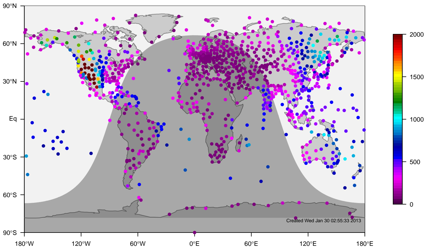
internal-TM5-ei-glb3x2 mixing height at 0UTC for June (1995-2011)
