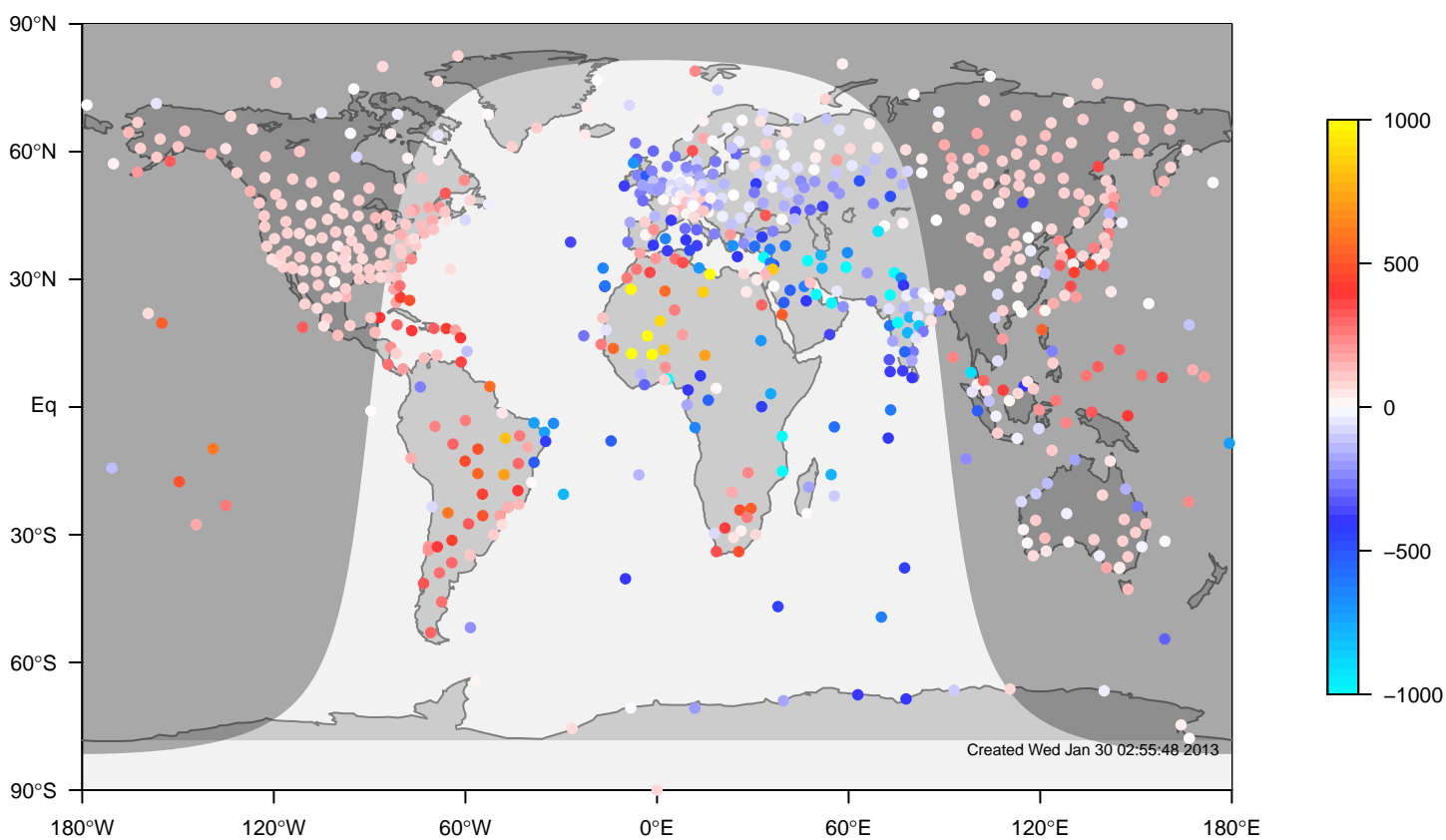
internal-TM5-ei-glb3x2 minus IGRA bias at 12UTC for October (1995-2011)
