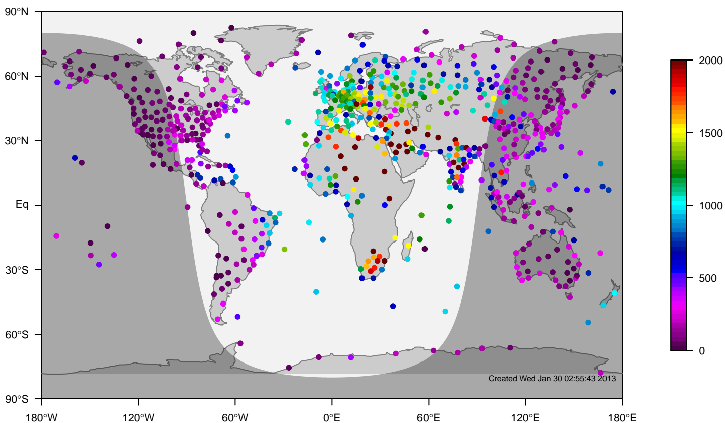
IGRA mixing height at 12UTC for April (1995-2011)
