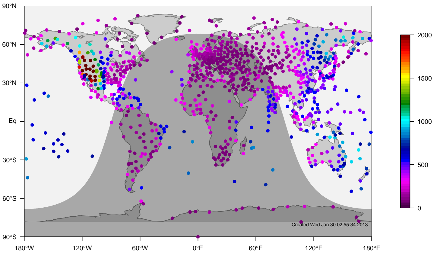
internal-TM5-ei-glb3x2 mixing height at 0UTC for July (1995-2011)
