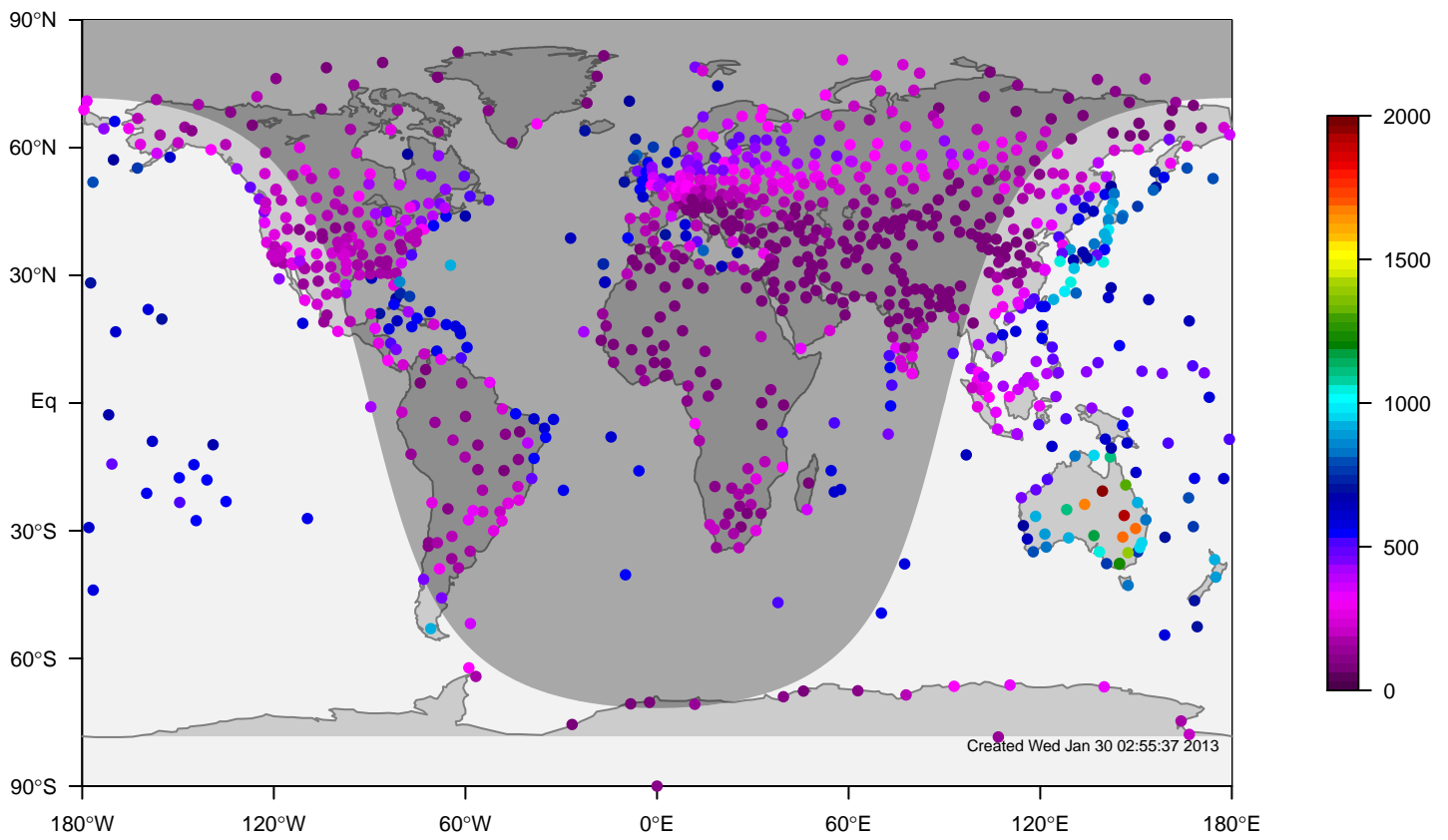
internal-TM5-ei-glb3x2 mixing height at 0UTC for November (1995-2011)
