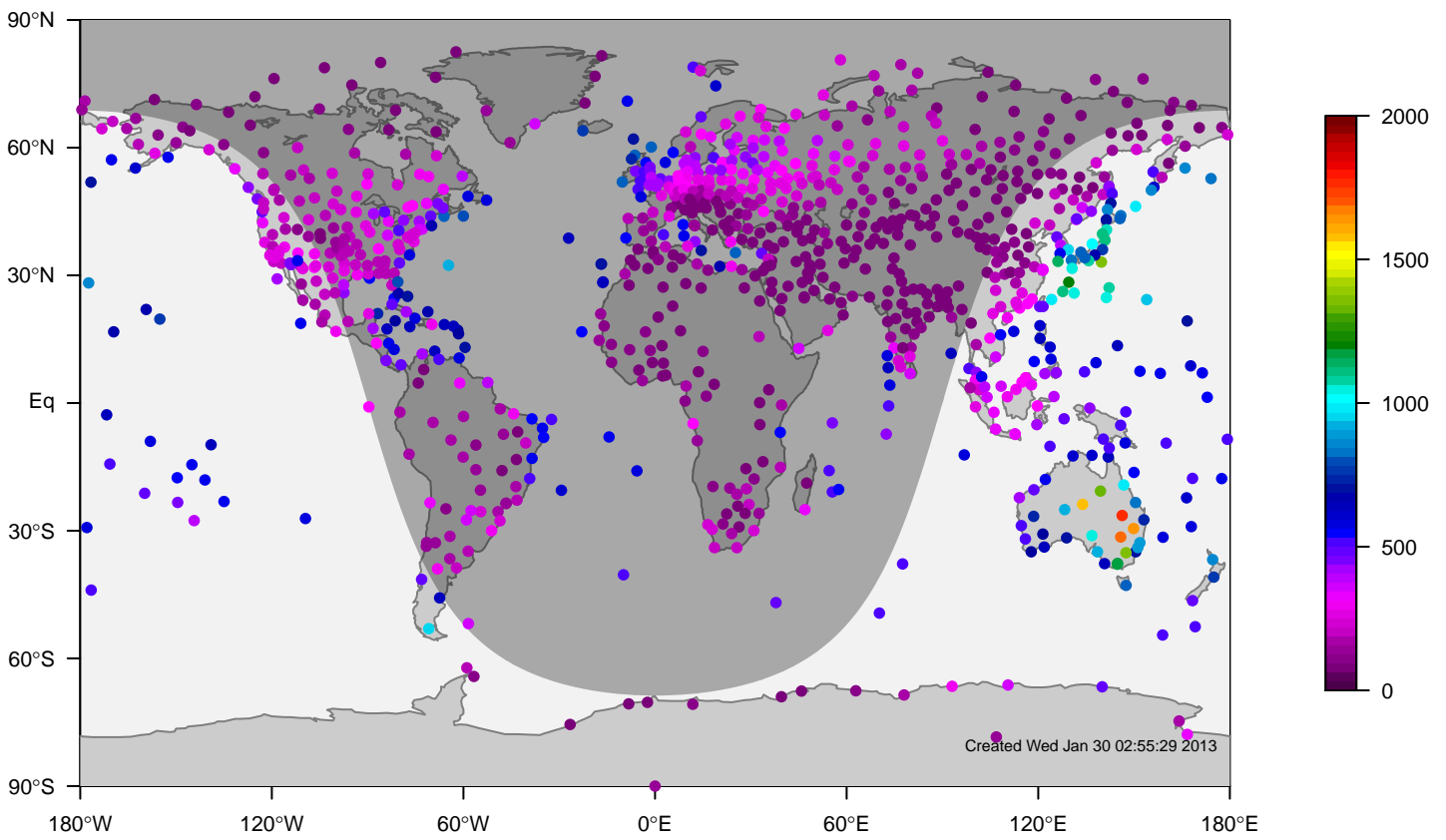
internal-TM5-ei-glb3x2 mixing height at 0UTC for January (1995-2011)
