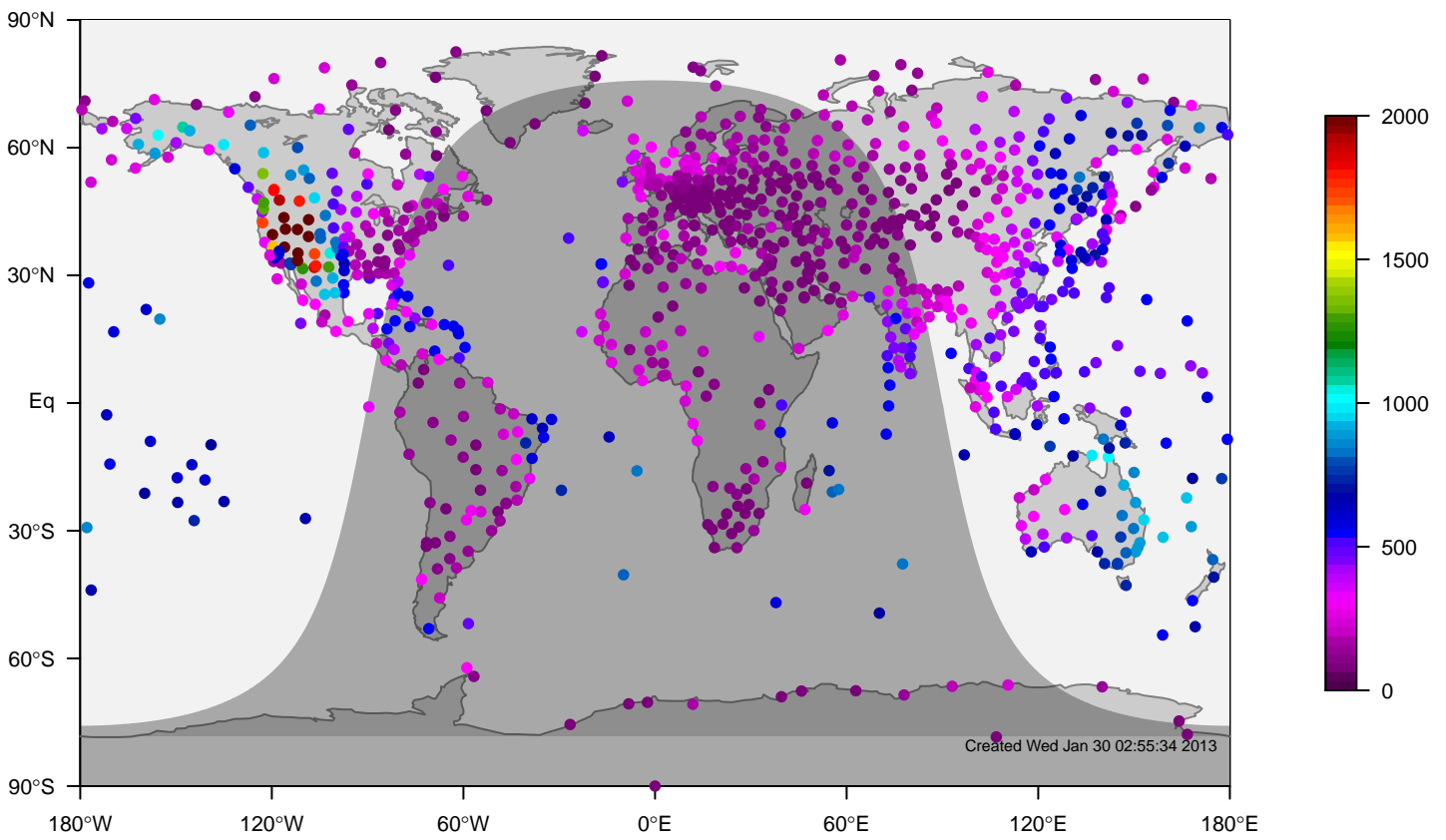
internal-TM5-ei-glb3x2 mixing height at 0UTC for August (1995-2011)
