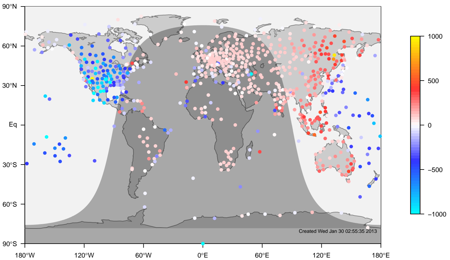
internal-TM5-ei-glb3x2 minus IGRA bias at 0UTC for August (1995-2011)
