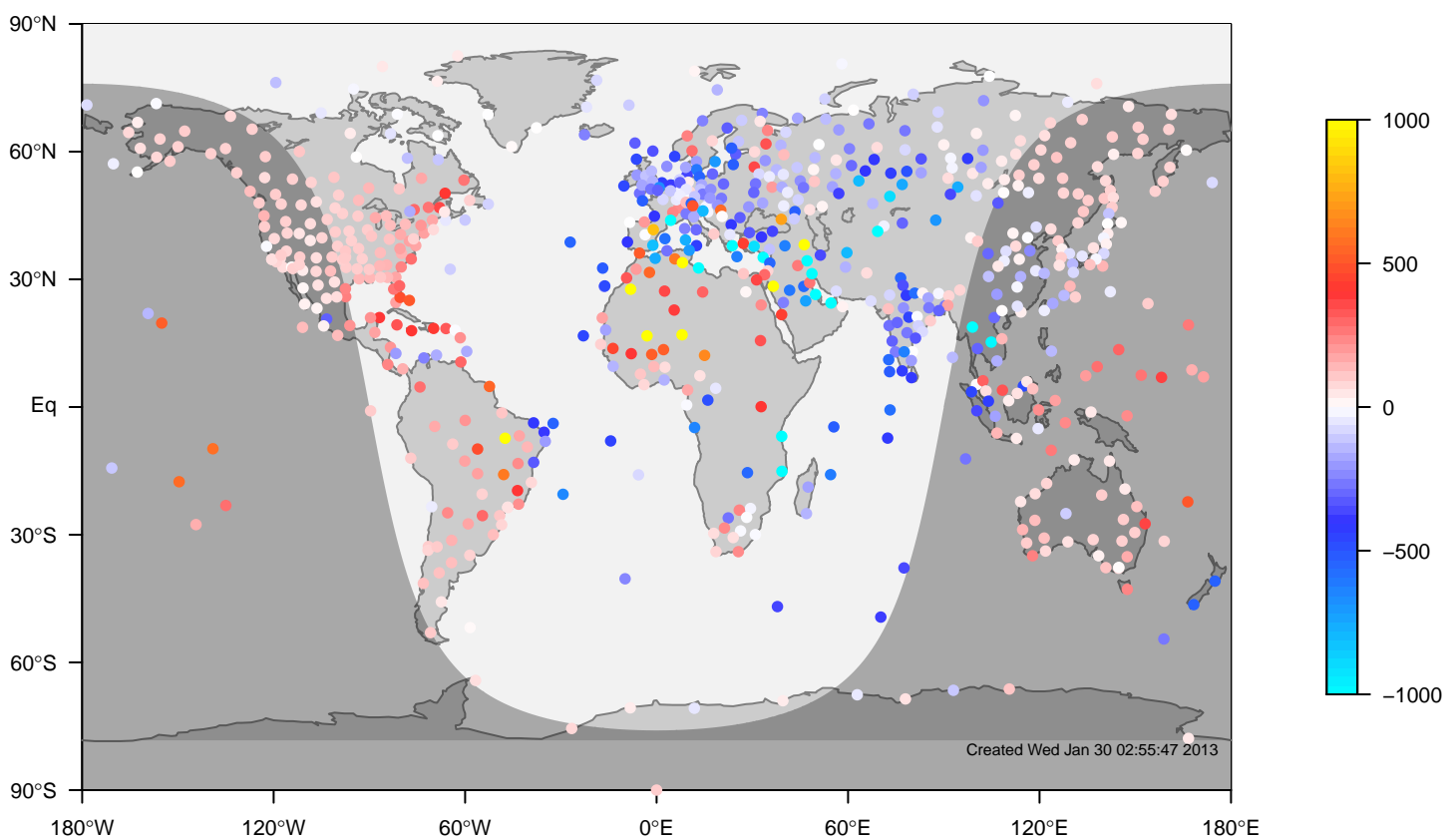
internal-TM5-ei-glb3x2 minus IGRA bias at 12UTC for August (1995-2011)
