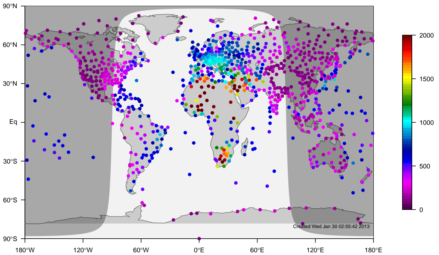
internal-TM5-ei-glb3x2 mixing height at 12UTC for March (1995-2011)
