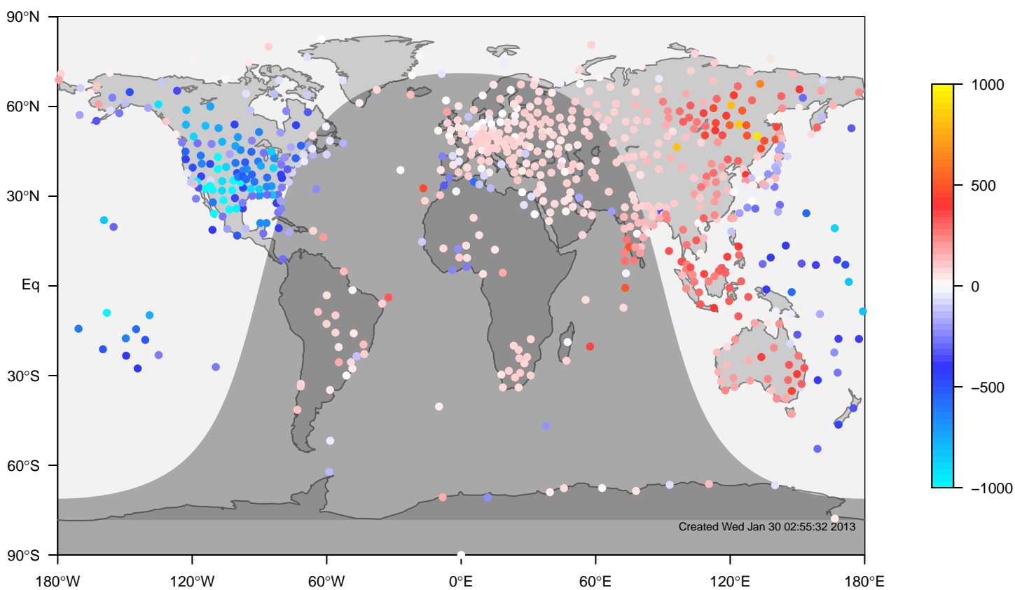
internal-TM5-ei-glb3x2 minus IGRA bias at 0UTC for May (1995-2011)
