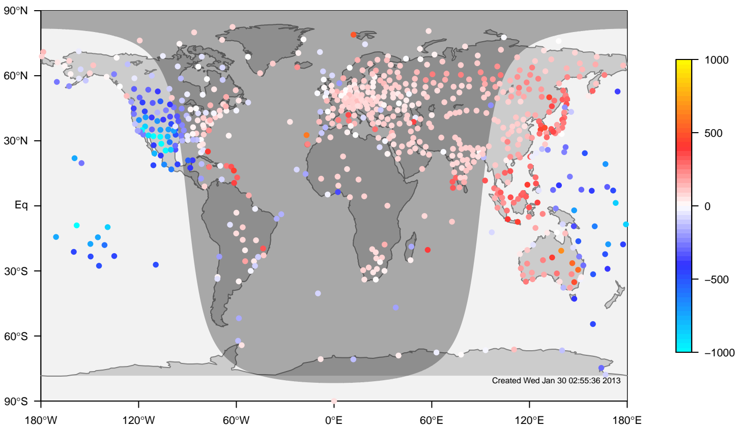
internal-TM5-ei-glb3x2 minus IGRA bias at 0UTC for October (1995-2011)
