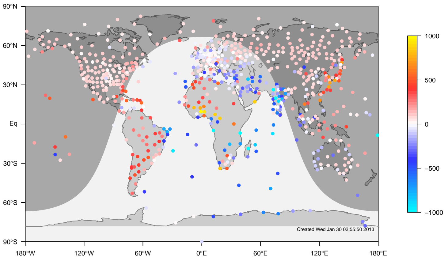
internal-TM5-ei-glb3x2 minus IGRA bias at 12UTC for December (1995-2011)
