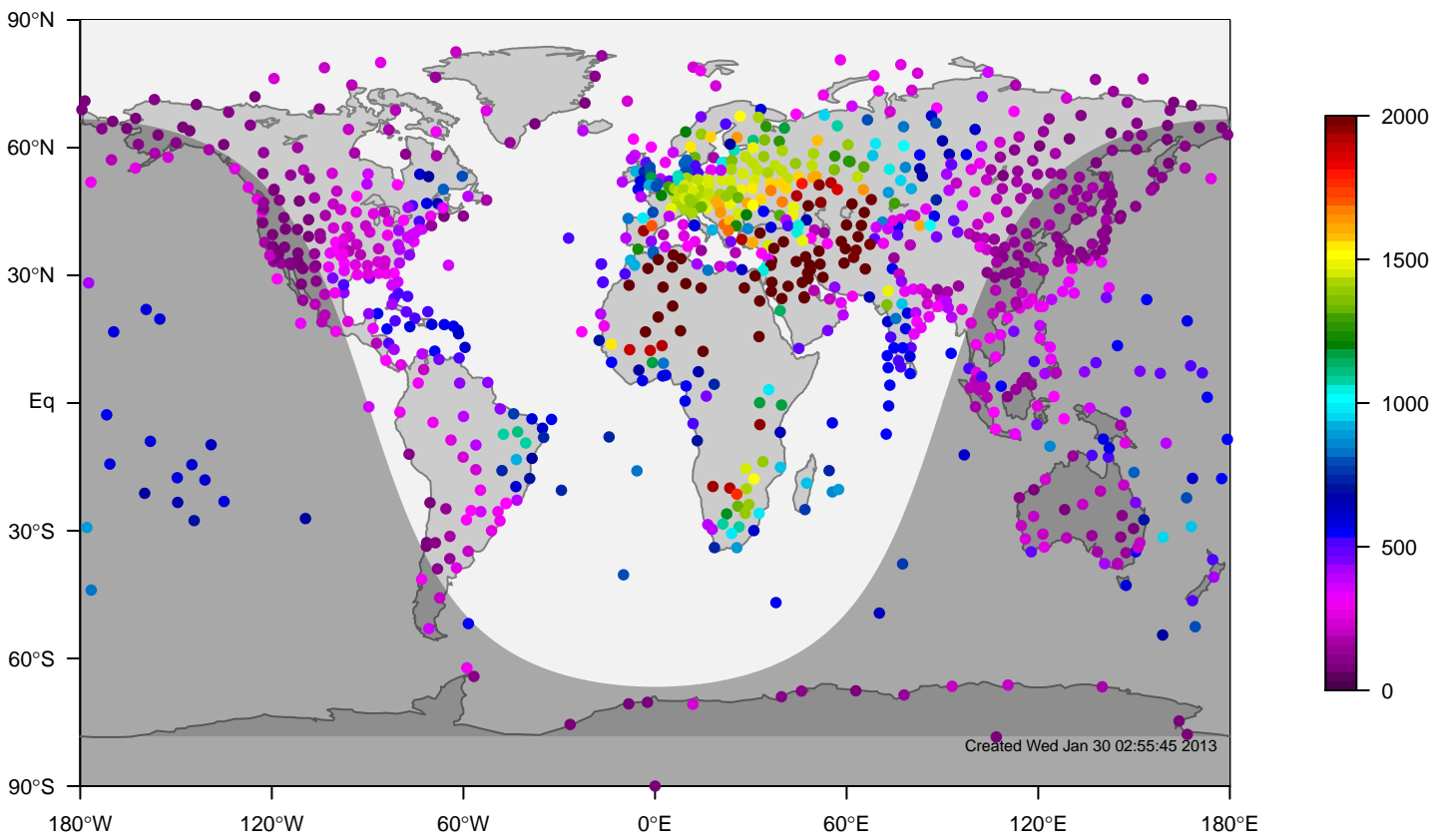
internal-TM5-ei-glb3x2 mixing height at 12UTC for June (1995-2011)
