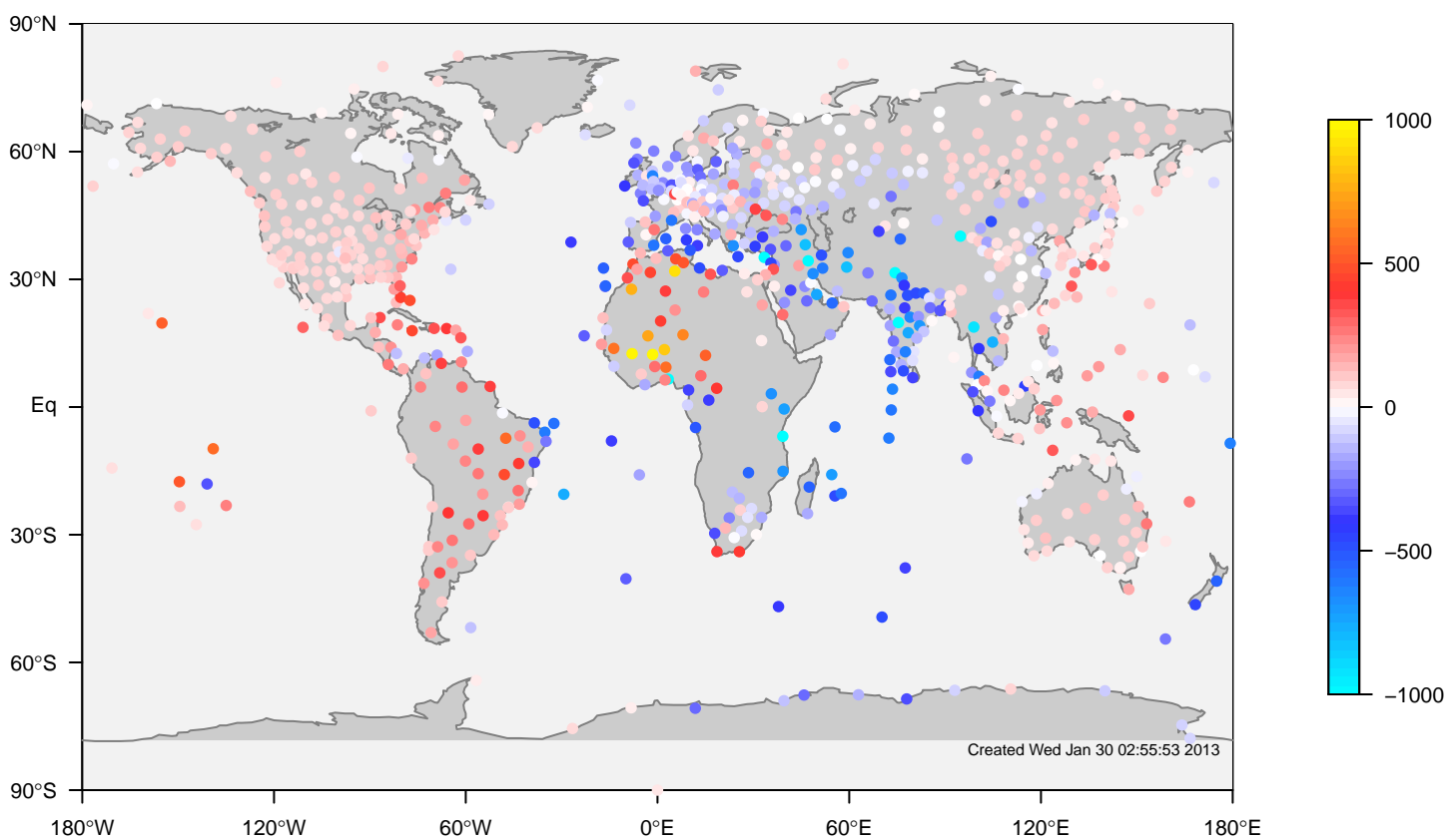
internal-TM5-ei-glb3x2 minus IGRA all-season bias at 12UTC (1995 - 2011)
