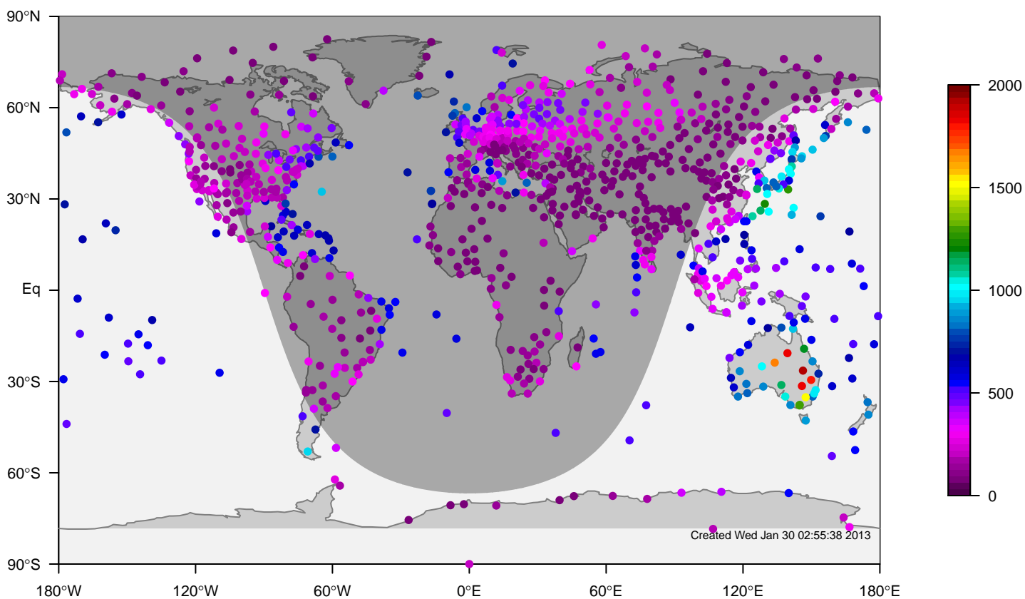
internal-TM5-ei-glb3x2 mixing height at 0UTC for December (1995-2011)
