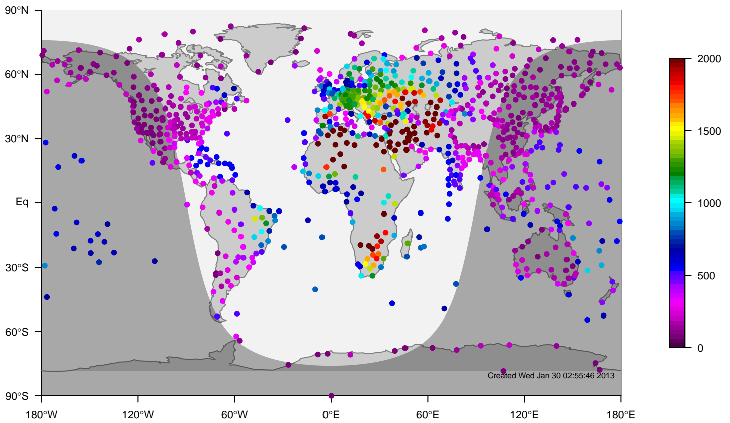
internal-TM5-ei-glb3x2 mixing height at 12UTC for August (1995-2011)
