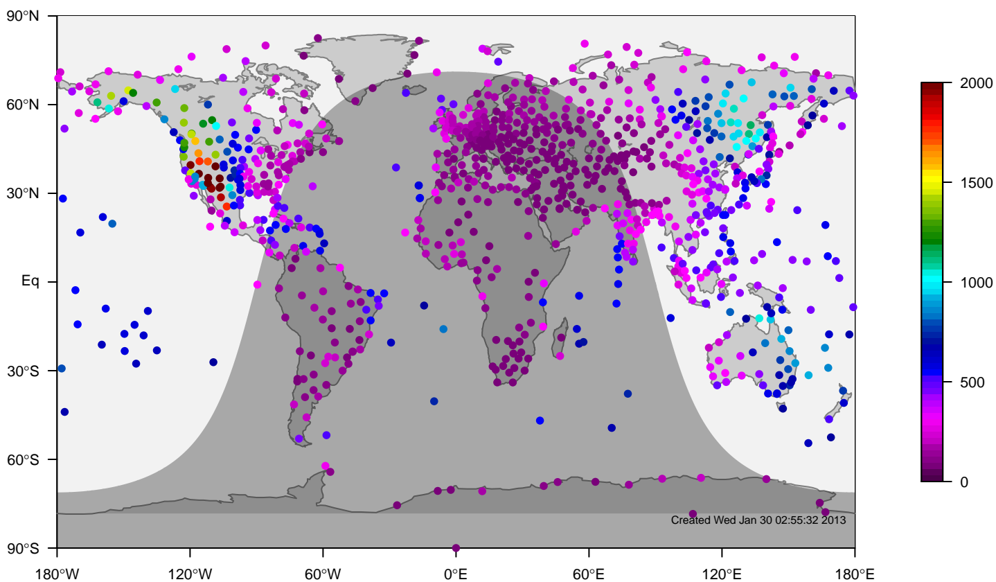
internal-TM5-ei-glb3x2 mixing height at 0UTC for May (1995-2011)
