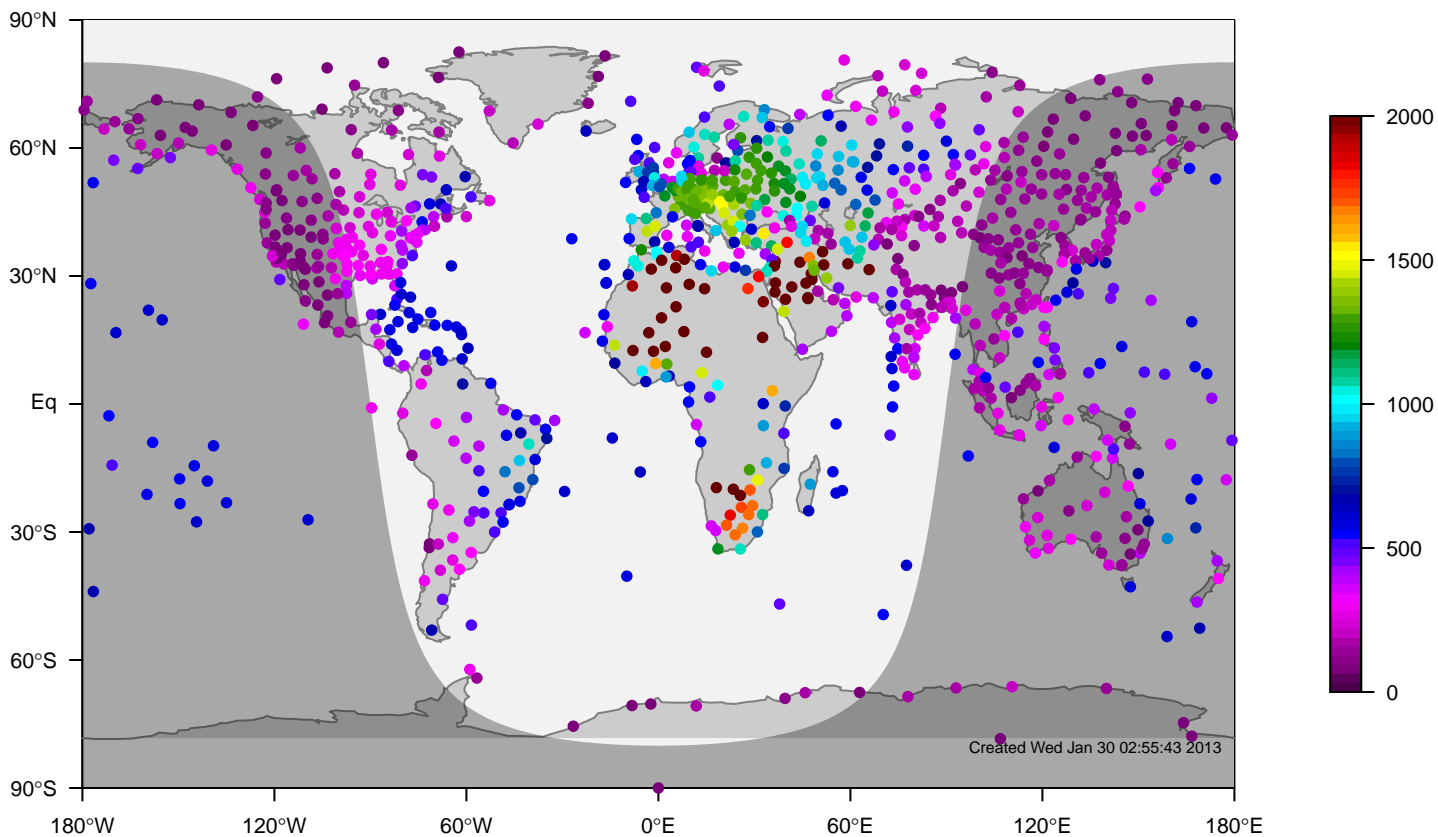
internal-TM5-ei-glb3x2 mixing height at 12UTC for April (1995-2011)
