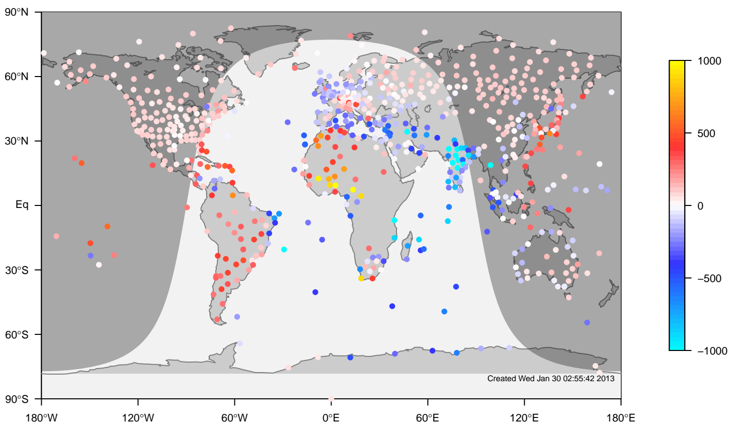
internal-TM5-ei-glb3x2 minus IGRA bias at 12UTC for February (1995-2011)
