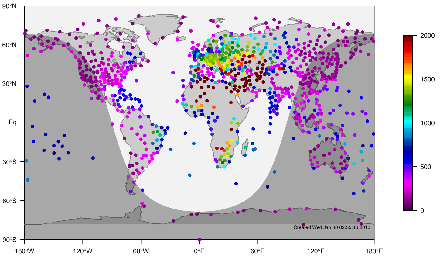
internal-TM5-ei-glb3x2 mixing height at 12UTC for July (1995-2011)
