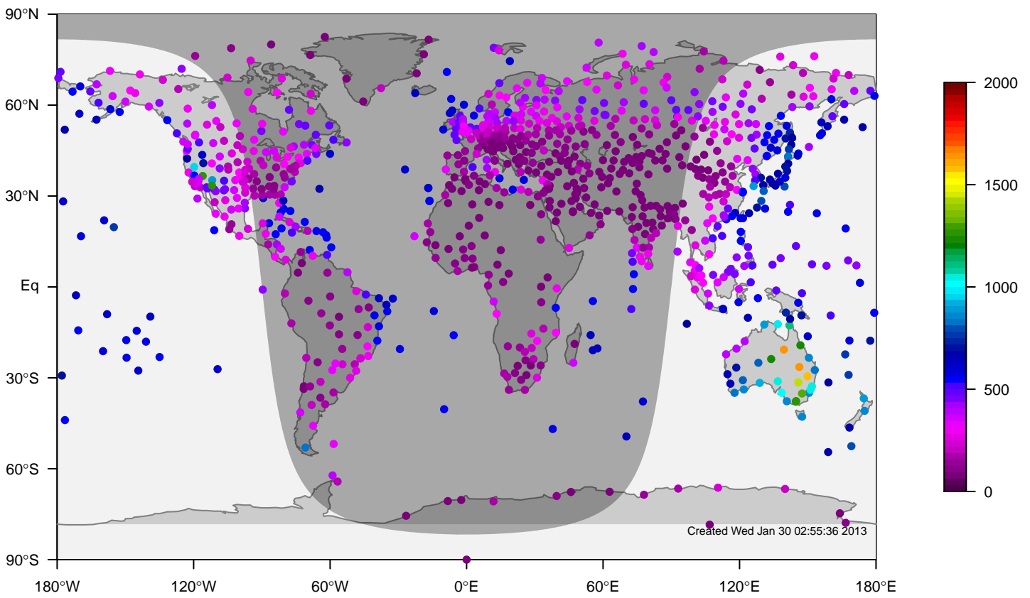
internal-TM5-ei-glb3x2 mixing height at 0UTC for October (1995-2011)
