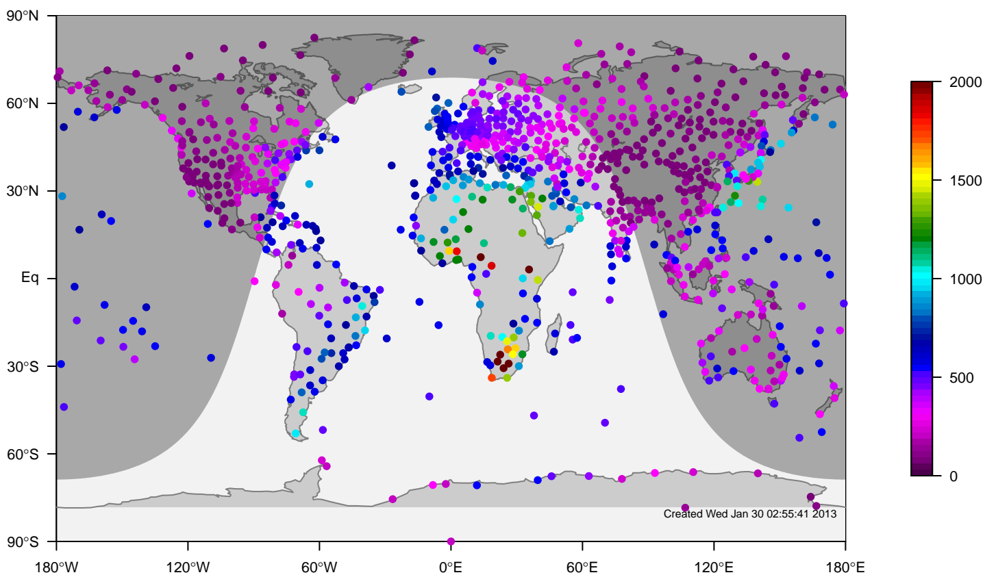
internal-TM5-ei-glb3x2 mixing height at 12UTC for January (1995-2011)
