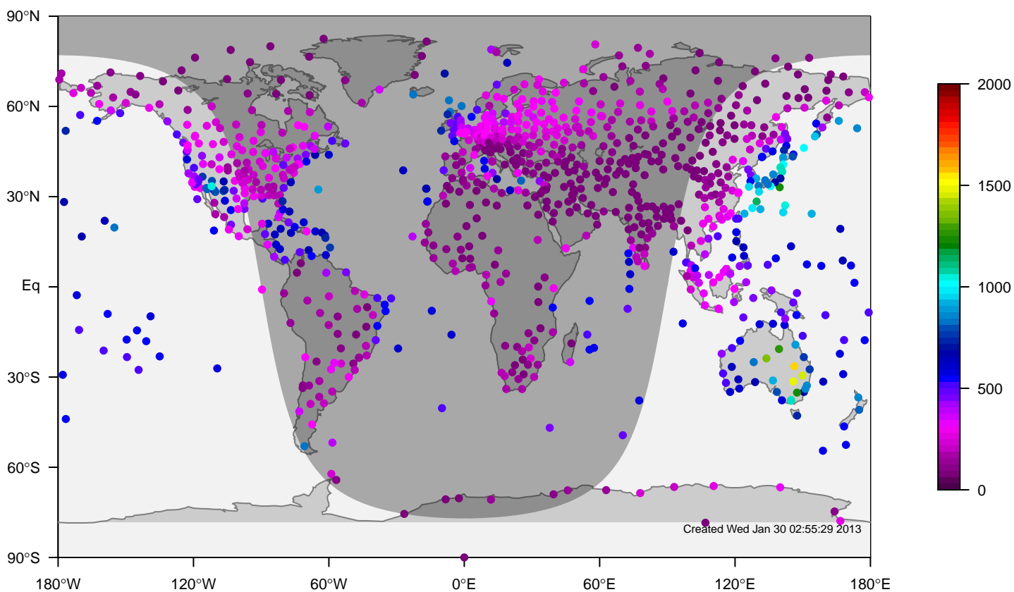
internal-TM5-ei-glb3x2 mixing height at 0UTC for February (1995-2011)
