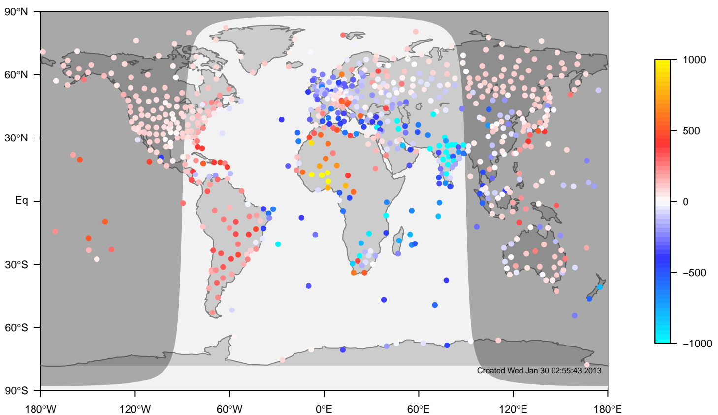
internal-TM5-ei-glb3x2 minus IGRA bias at 12UTC for March (1995-2011)
