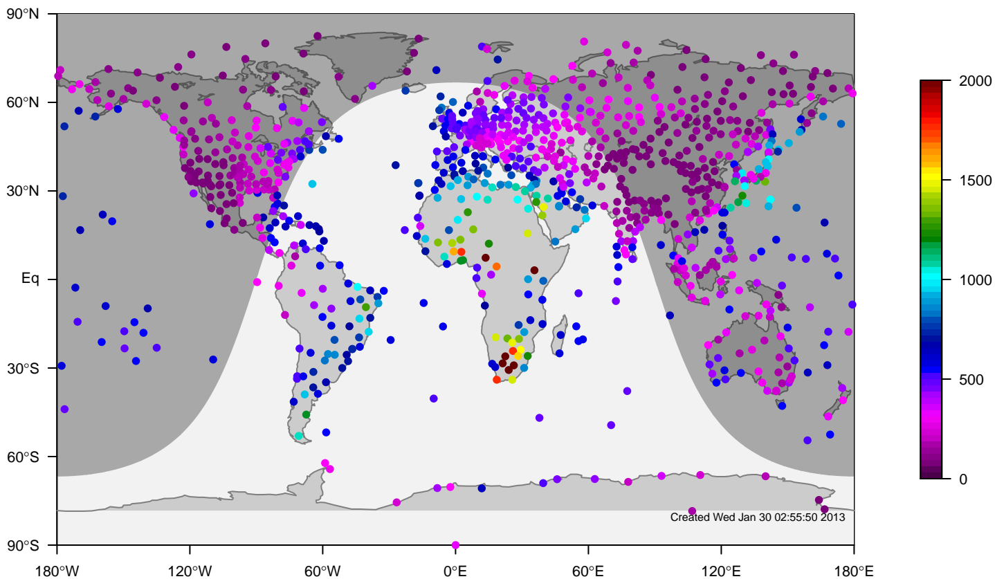
internal-TM5-ei-glb3x2 mixing height at 12UTC for December (1995-2011)
