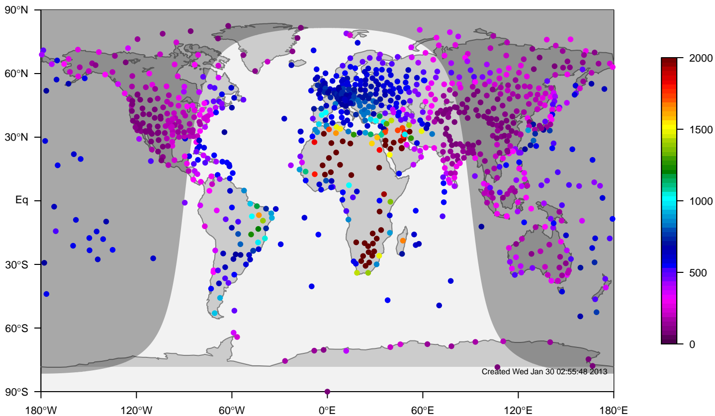
internal-TM5-ei-glb3x2 mixing height at 12UTC for October (1995-2011)
