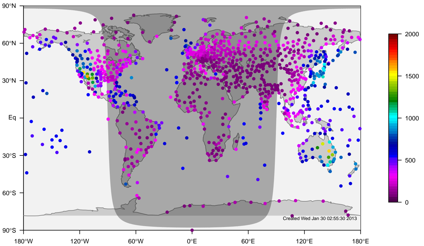
internal-TM5-ei-glb3x2 mixing height at 0UTC for March (1995-2011)
