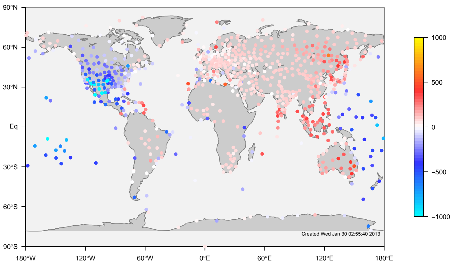
internal-TM5-ei-glb3x2 minus IGRA all-season bias at OUTC (1995 - 2011)
