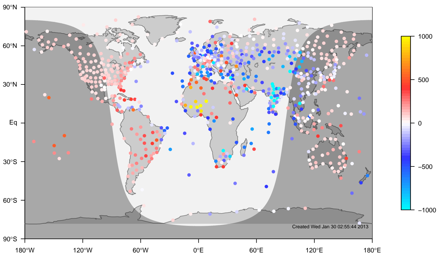
internal-TM5-ei-glb3x2 minus IGRA bias at 12UTC for April (1995-2011)
