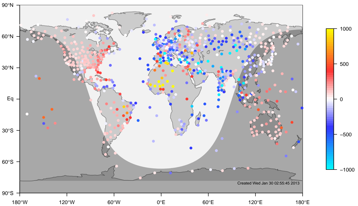
internal-TM5-ei-glb3x2 minus IGRA bias at 12UTC for June (1995-2011)
