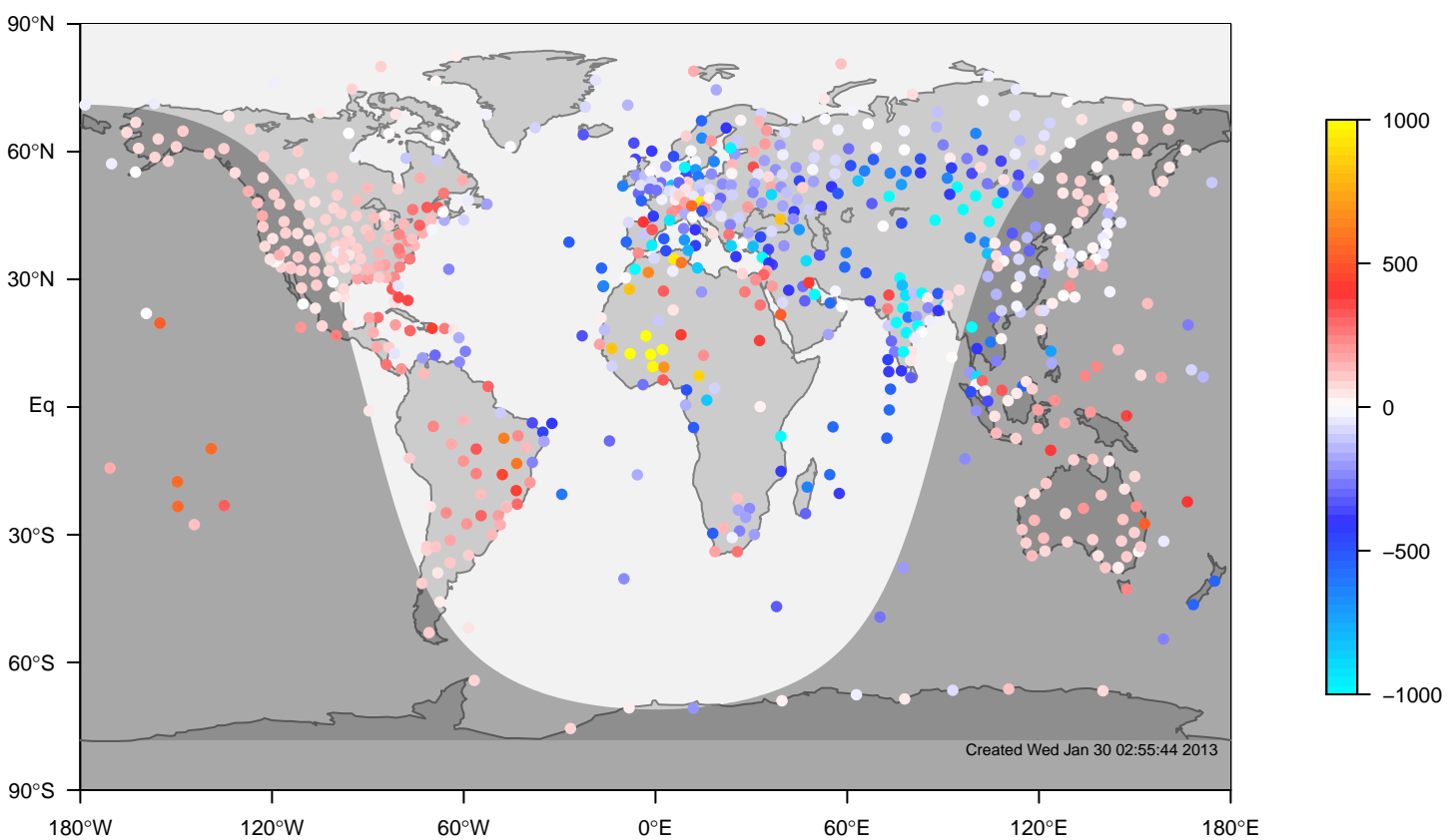
internal-TM5-ei-glb3x2 minus IGRA bias at 12UTC for May (1995-2011)
