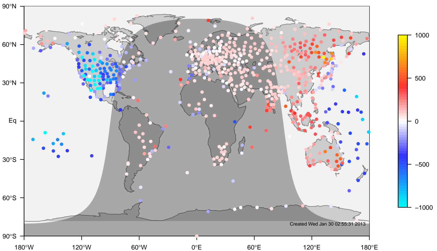
internal-TM5-ei-glb3x2 minus IGRA bias at 0UTC for April (1995-2011)
