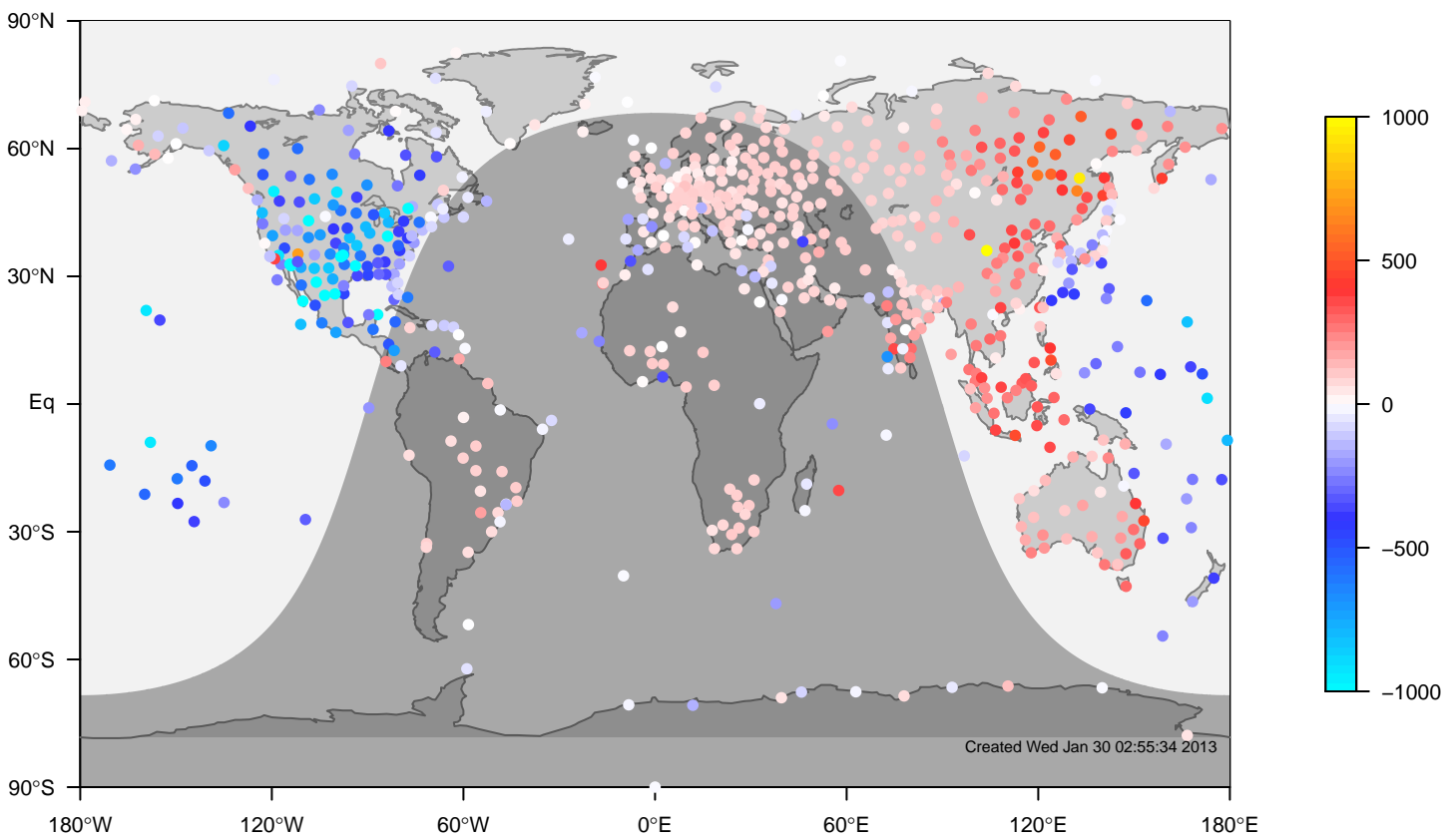
internal-TM5-ei-glb3x2 minus IGRA bias at 0UTC for July (1995-2011)
