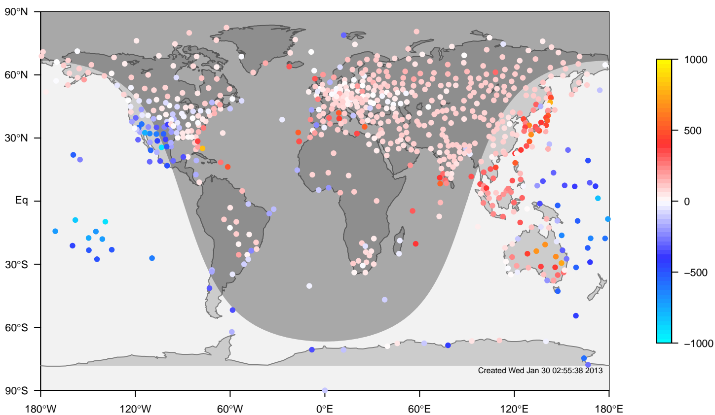
internal-TM5-ei-glb3x2 minus IGRA bias at 0UTC for December (1995-2011)
