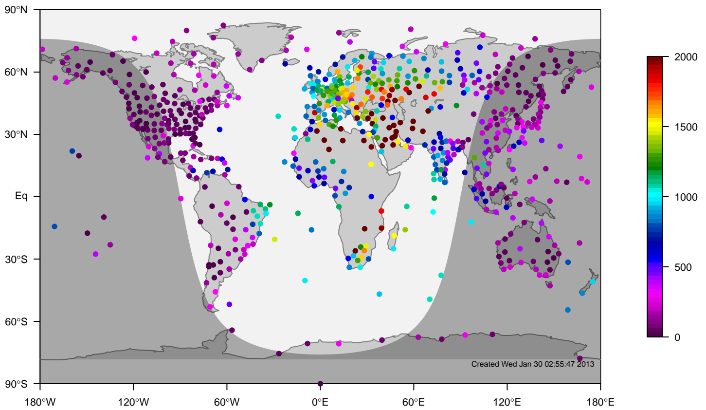
IGRA mixing height at 12UTC for August (1995-2011)
