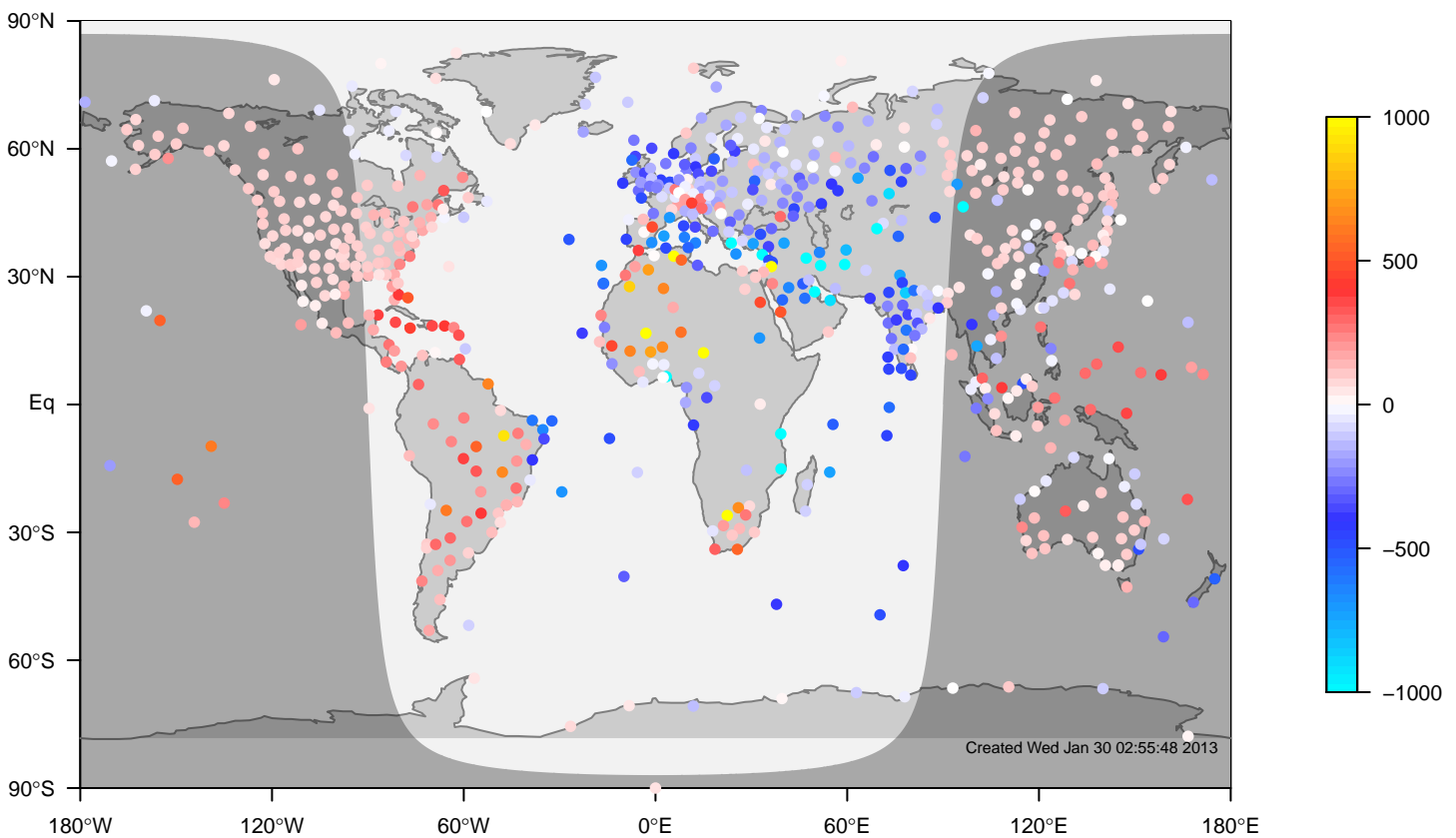
internal-TM5-ei-glb3x2 minus IGRA bias at 12UTC for September (1995-2011)
