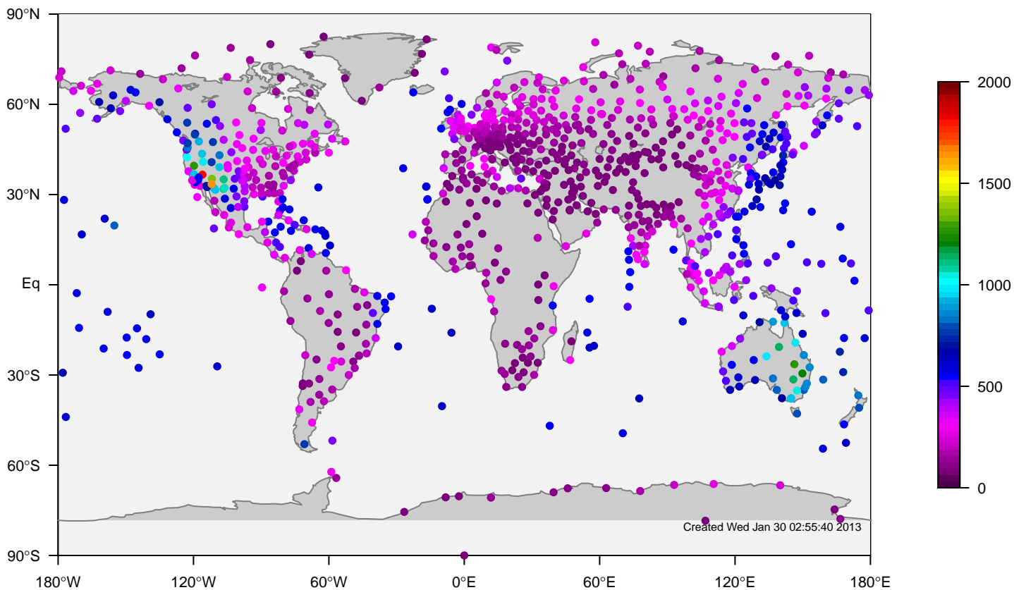
internal-TM5-ei-glb3x2 all-season mixing height at OUTC (1995-2011)
