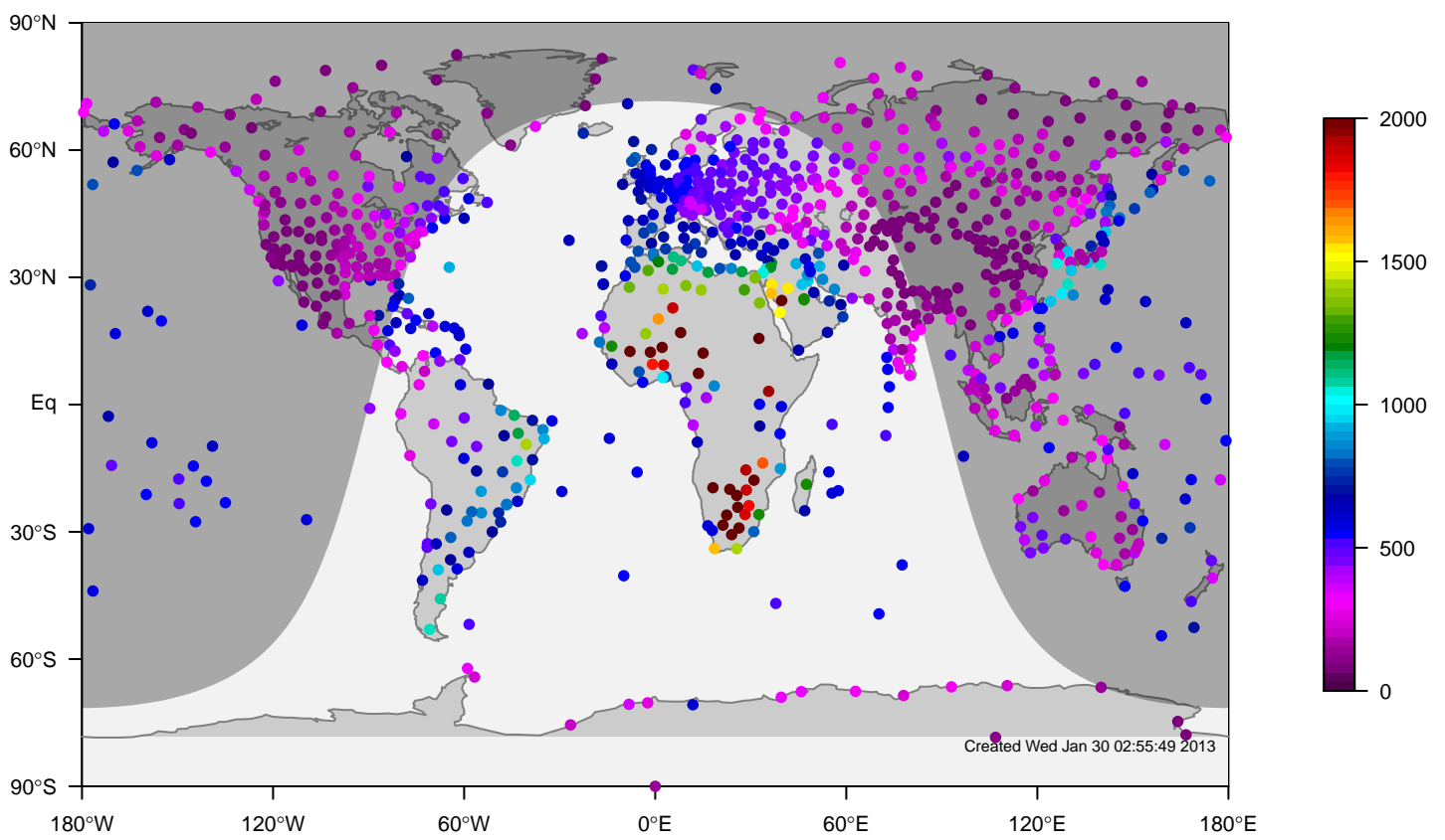
internal-TM5-ei-glb3x2 mixing height at 12UTC for November (1995-2011)
