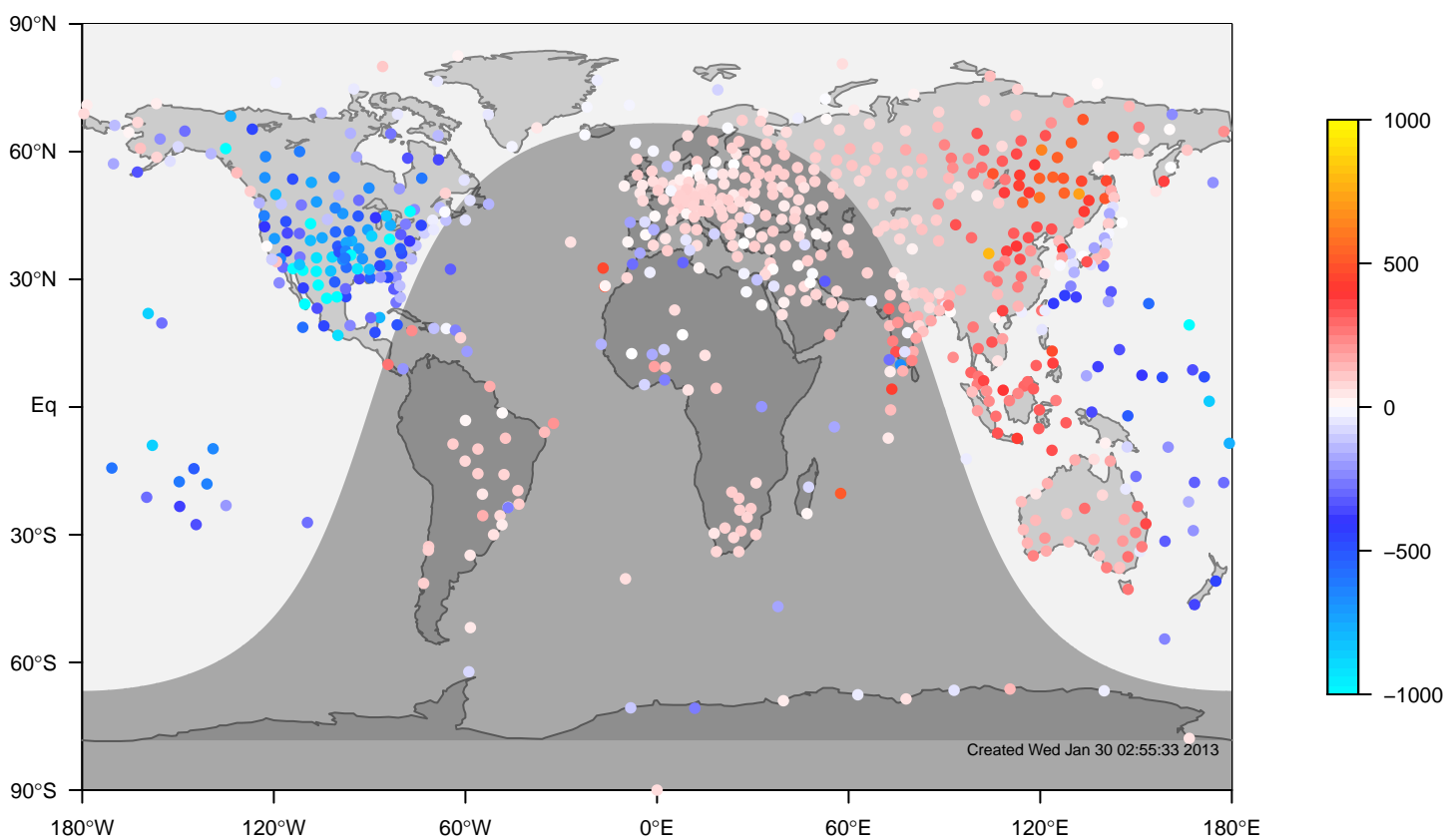
internal-TM5-ei-glb3x2 minus IGRA bias at 0UTC for June (1995-2011)
