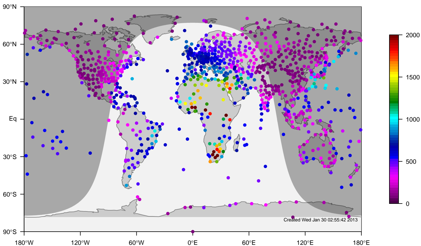
internal-TM5-ei-glb3x2 mixing height at 12UTC for February (1995-2011)
