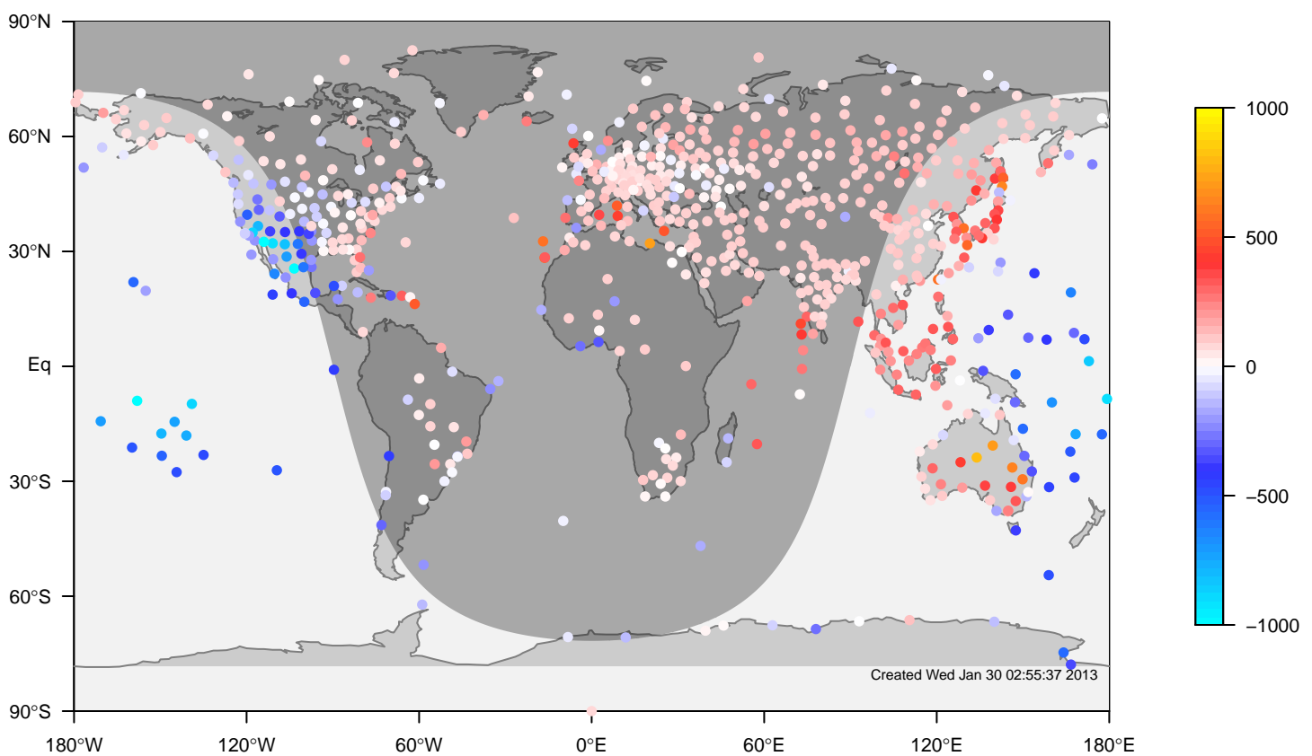
internal-TM5-ei-glb3x2 minus IGRA bias at 0UTC for November (1995-2011)
