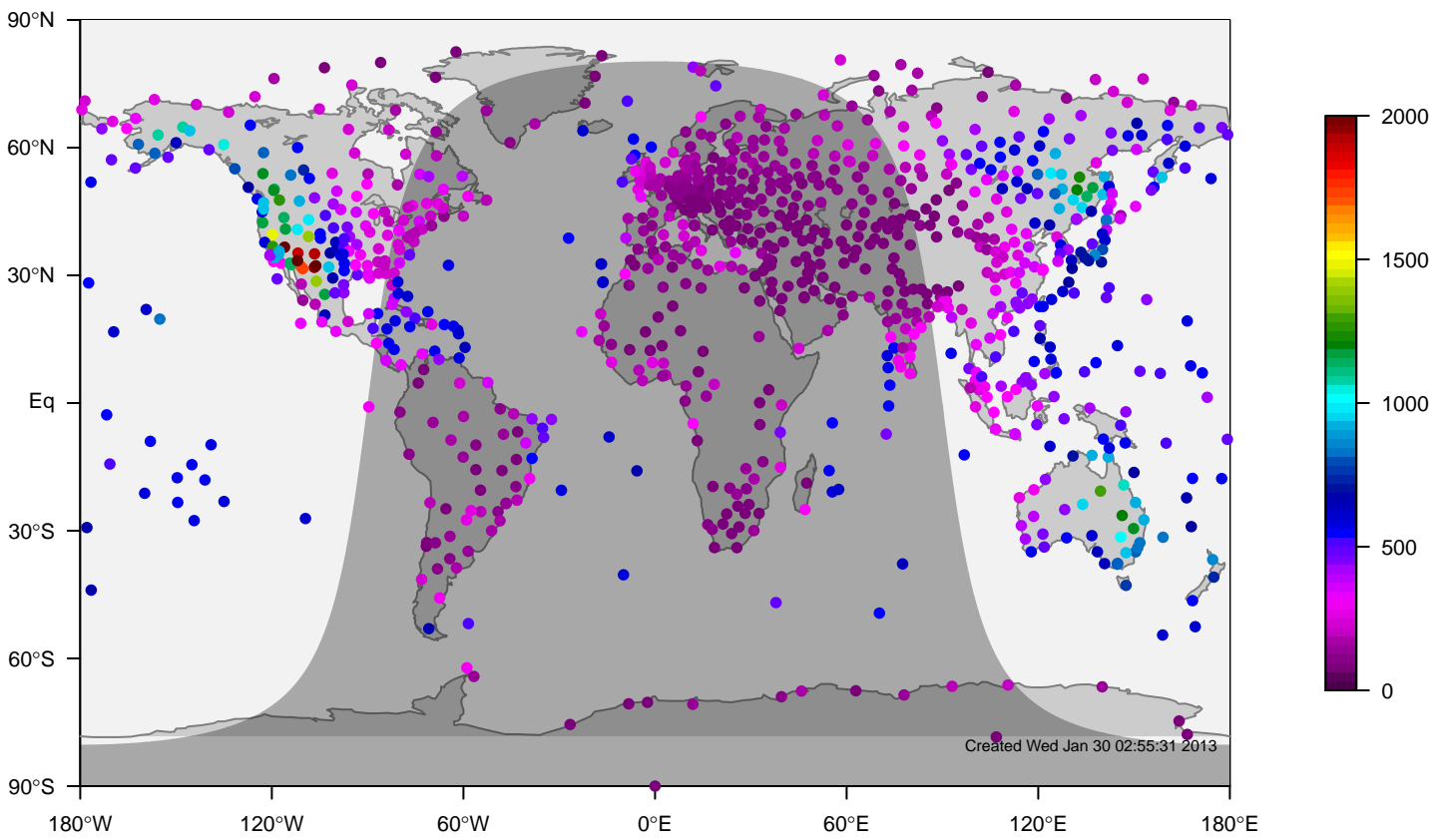
internal-TM5-ei-glb3x2 mixing height at 0UTC for April (1995-2011)
