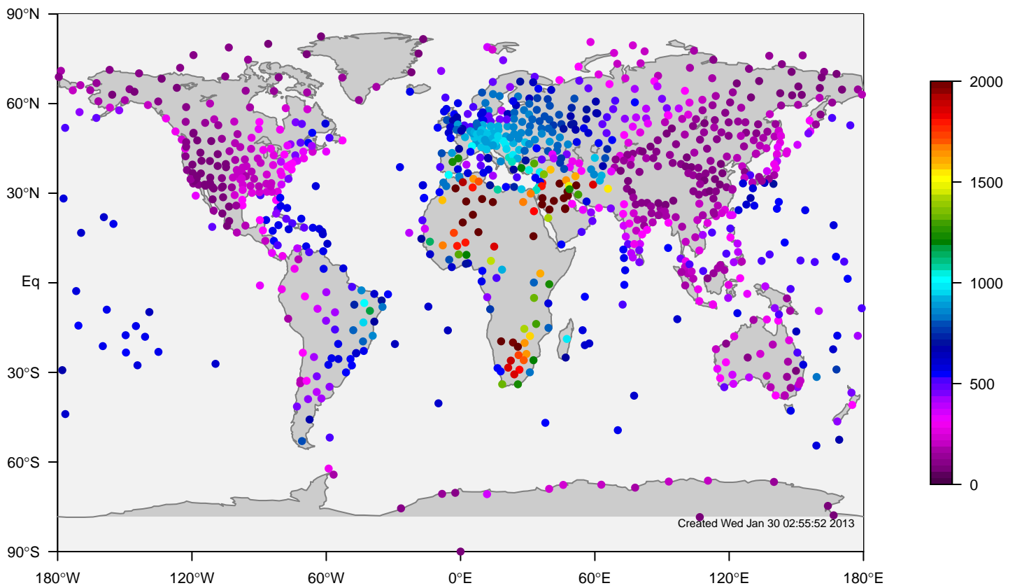
internal-TM5-ei-glb3x2 all-season mixing height at 12UTC (1995-2011)
