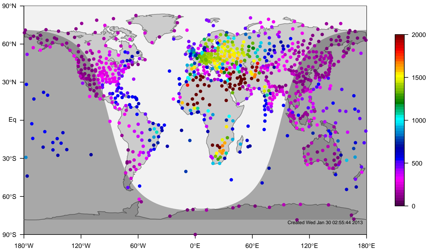
internal-TM5-ei-glb3x2 mixing height at 12UTC for May (1995-2011)
