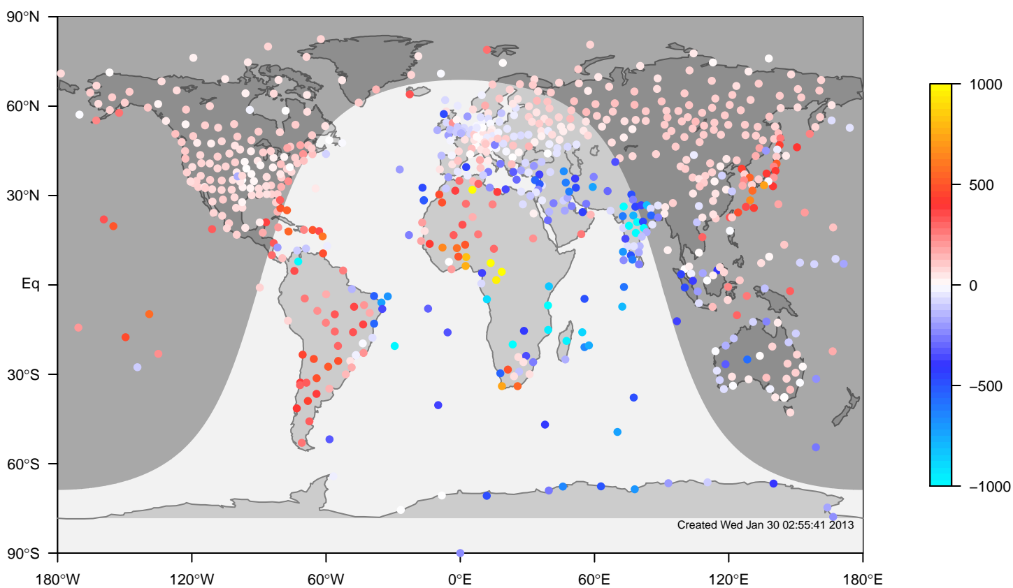
internal-TM5-ei-glb3x2 minus IGRA bias at 12UTC for January (1995-2011)
