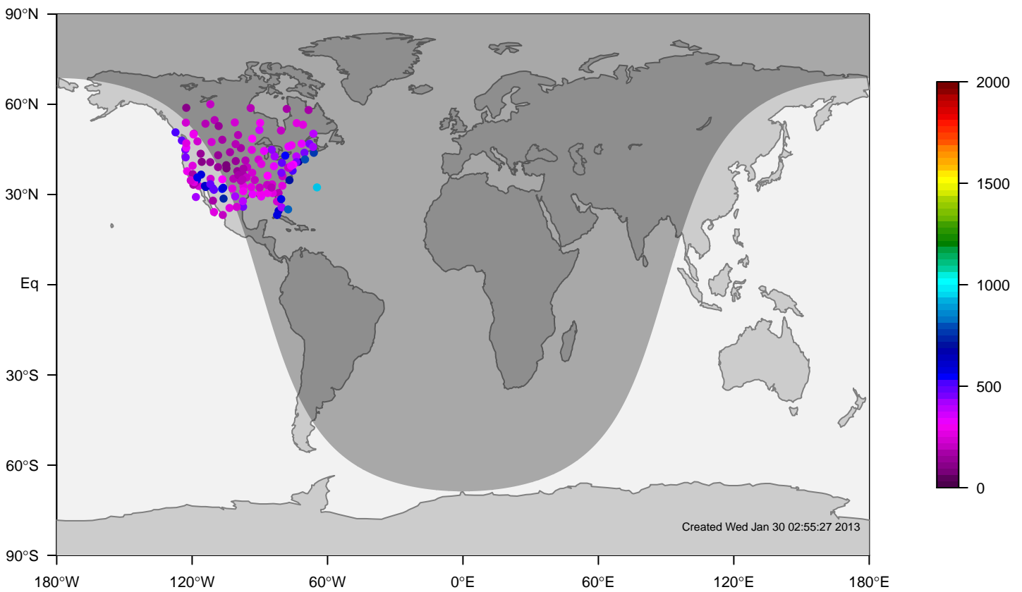
internal-TM5-od-tmpp-nam1x1 mixing height at UTC for January (2000-2011)
