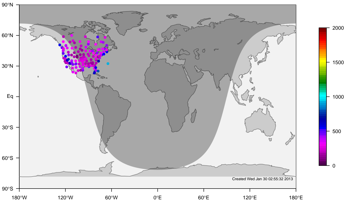
internal-TM5-od-tmpp-nam1x1 mixing height at 0UTC for November (2000-2011)
