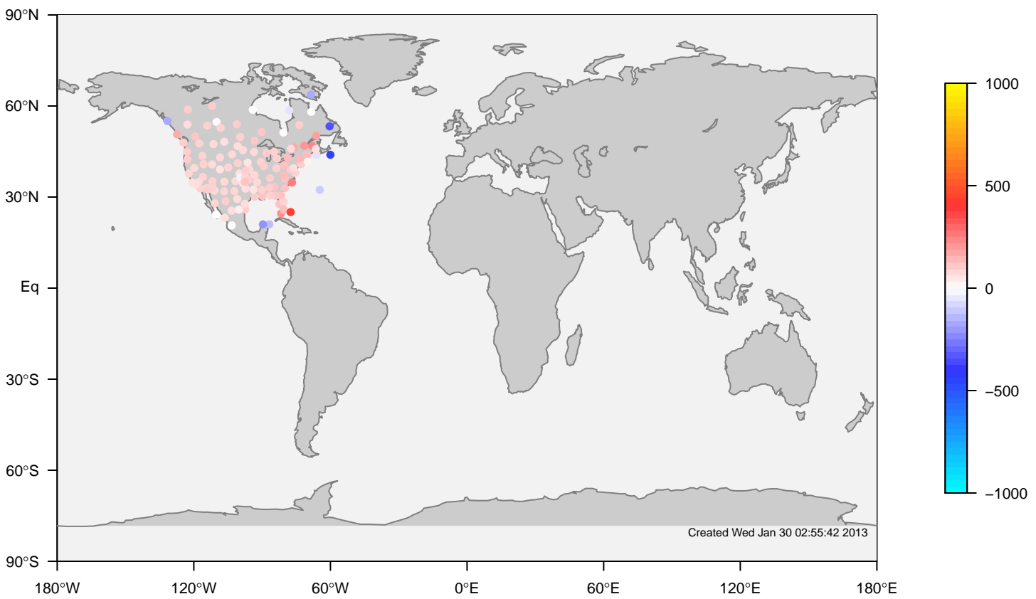
internal-TM5-od-tmpp-nam1x1 minus IGRA all-season bias at 12UTC (2000 - 2011)
