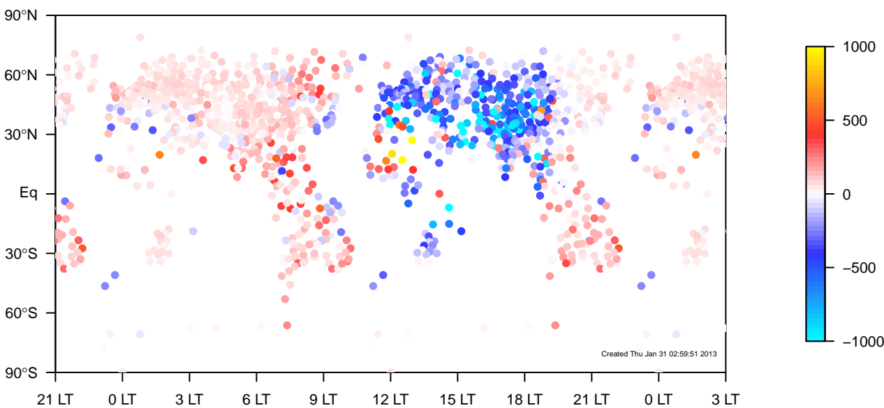
TM5-ei-glb3x2 minus IGRA land-only JJA mixing height median (1995–2011)
