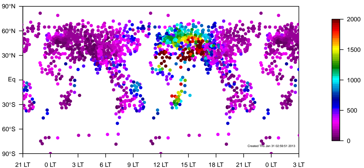
TM5-ei-glb3x2 land-only JJA mixing height median (1995–2011)
