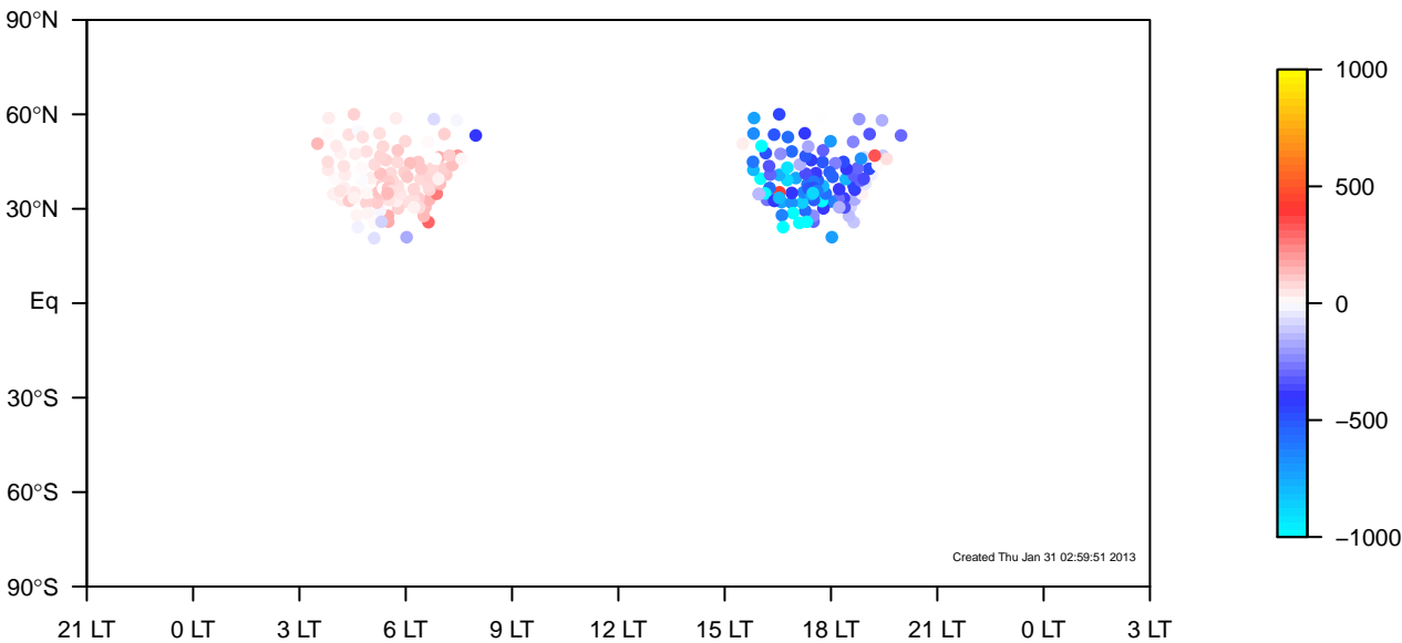
TM5-ei-nam1x1 minus IGRA land-only JJA mixing height median (1995–2011)
