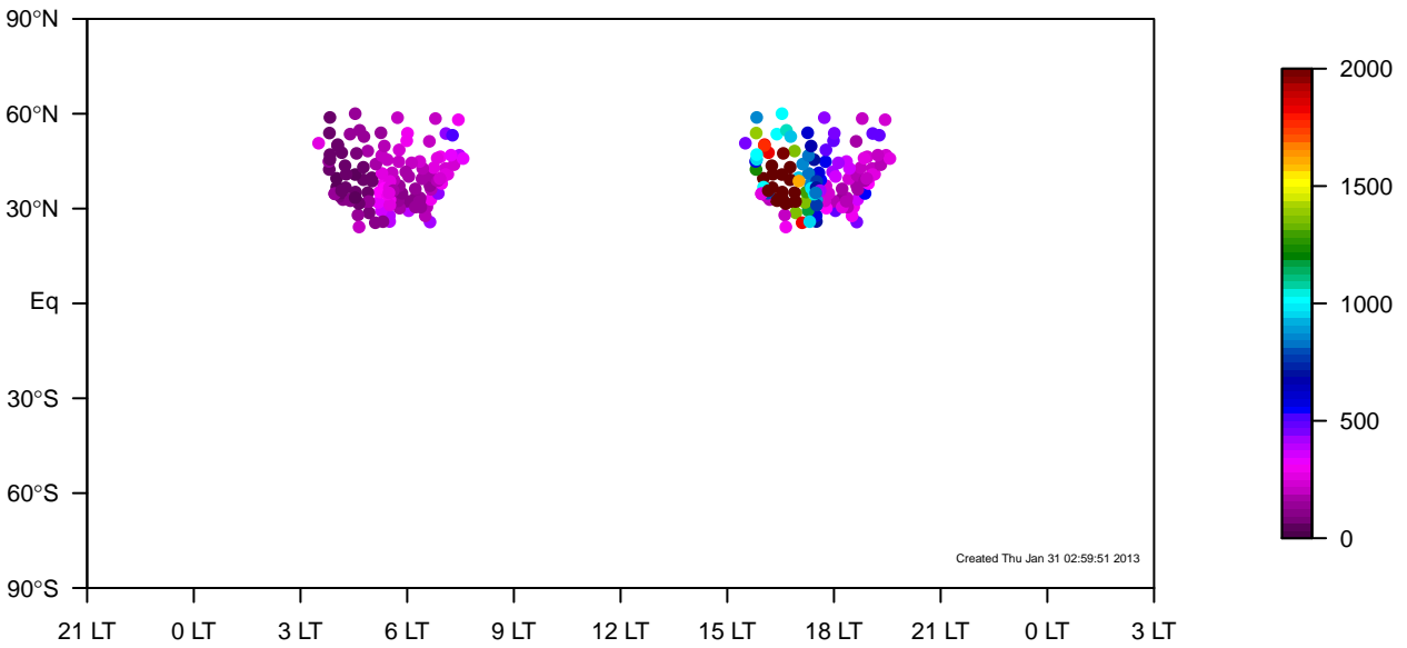
TM5-ei-nam1x1 land-only JJA mixing height median (1995–2011)
