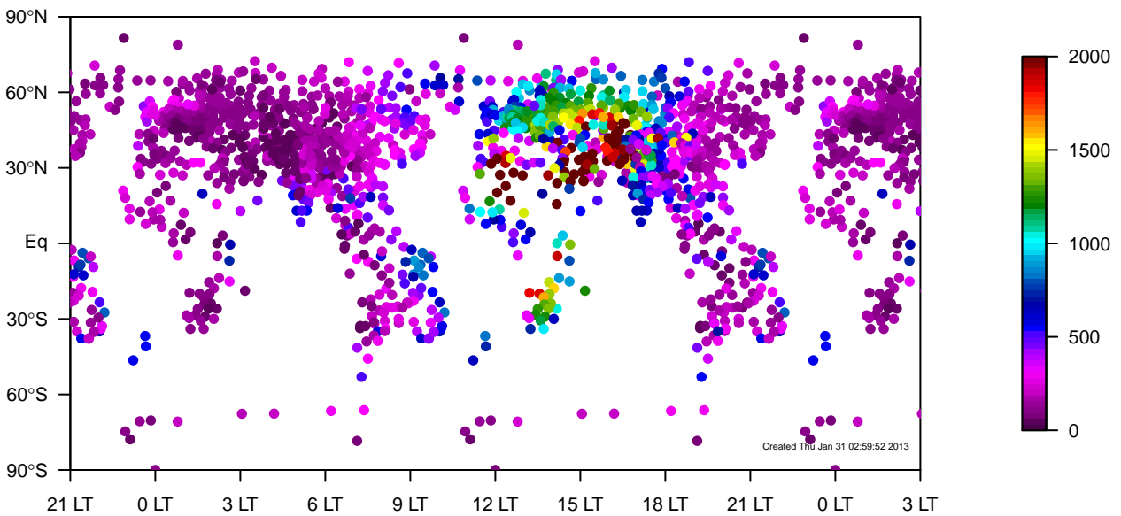
TM5-od-tmpp-glb3x2 land-only JJA mixing height median (2000–2011)
