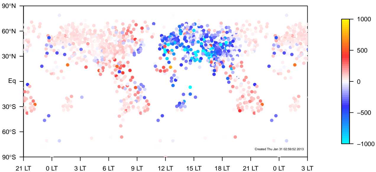
TM5-od-tmpp-glb3x2 minus IGRA land-only JJA mixing height median (2000–2011)
