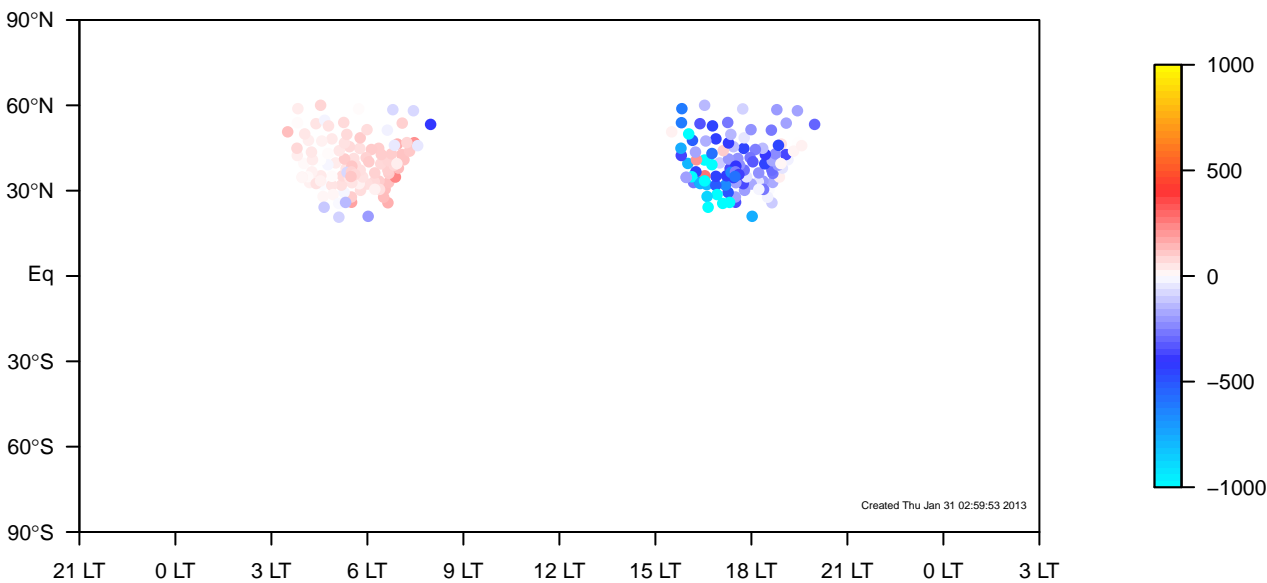
TM5-od-tmpp-nam1x1 minus IGRA land-only JJA mixing height median (2000–2011)
