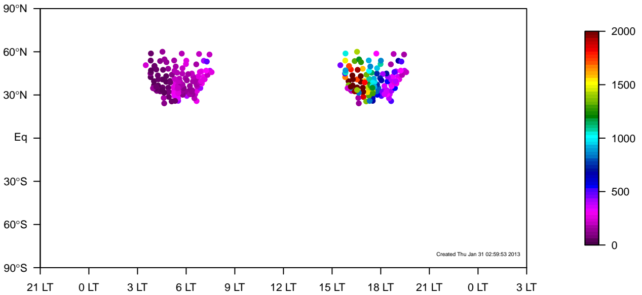
TM5-od-tmpp-nam1x1 land-only JJA mixing height median (2000–2011)
