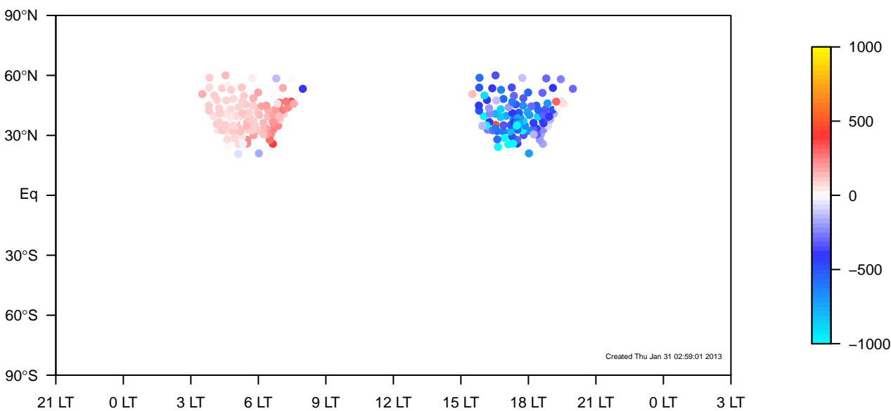
internal-TM5-ei-nam1x1 minus IGRA land-only JJA mixing height median (1995–2011)
