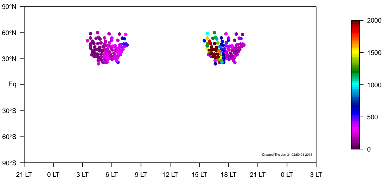
internal-TM5-ei-nam1x1 land-only JJA mixing height median (1995–2011)
