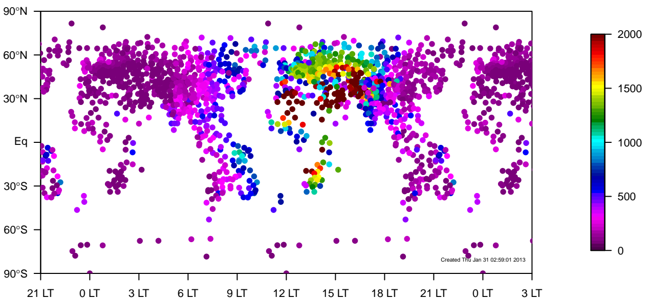
internal-TM5-od-tmpp-glb3x2 land-only JJA mixing height median (2000–2011)
