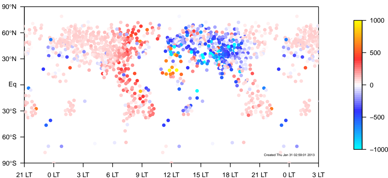
internal-TM5-od-tmpp-glb3x2 minus IGRA land-only JJA mixing height median (2000–2011)
