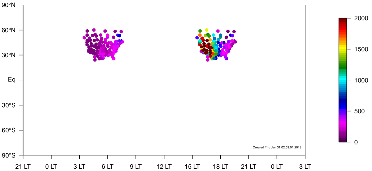
internal-TM5-od-tmpp-nam1x1 land-only JJA mixing height median (2000–2011)
