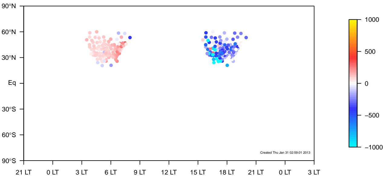
internal-TM5-od-tmpp-nam1x1 minus IGRA land-only JJA mixing height median (2000–2011)
