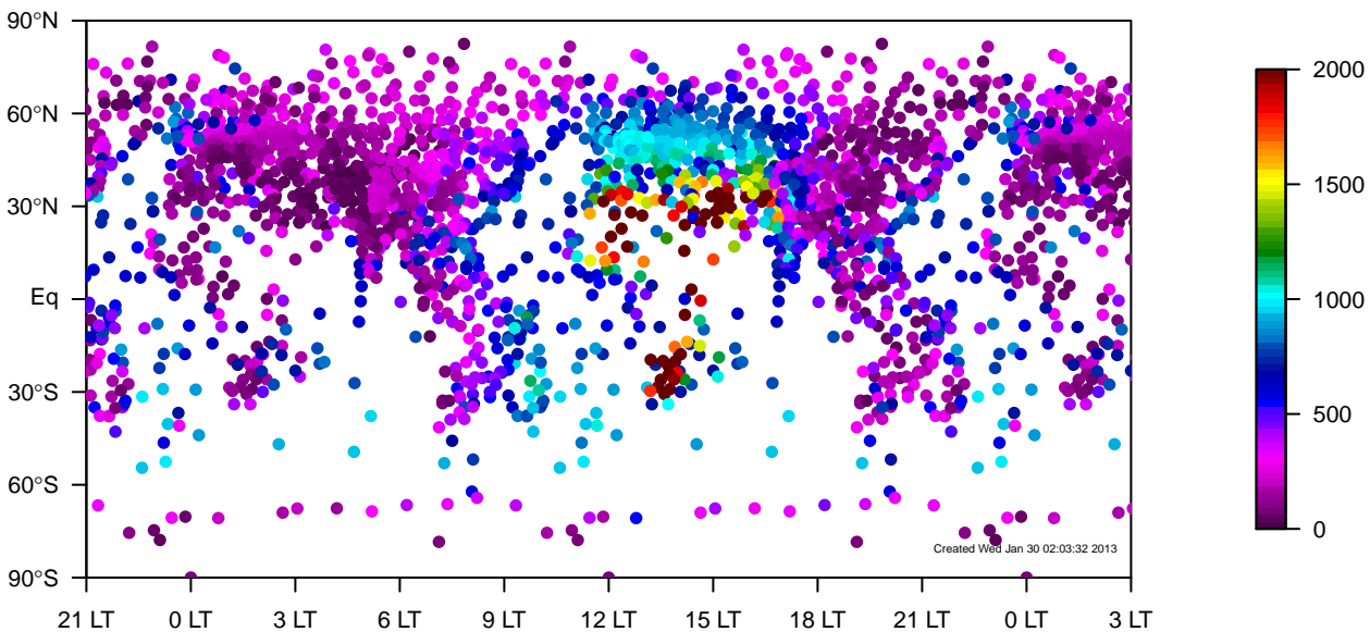
ERA-i all-season mixing height median (1981–2006)
