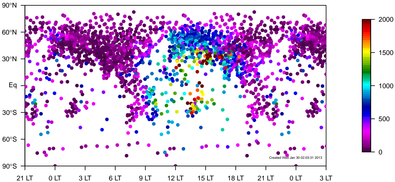
IGRA all-season mixing height median (1981–2006)
