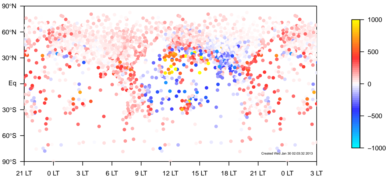
ERA-i minus IGRA all-season mixing height median (1981–2006)
