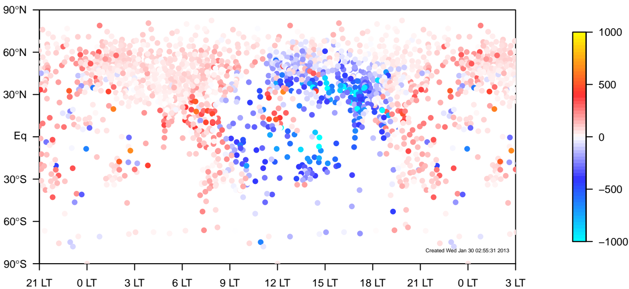
TM5-ei-glb3x2 minus IGRA all-season mixing height median (1995–2011)
