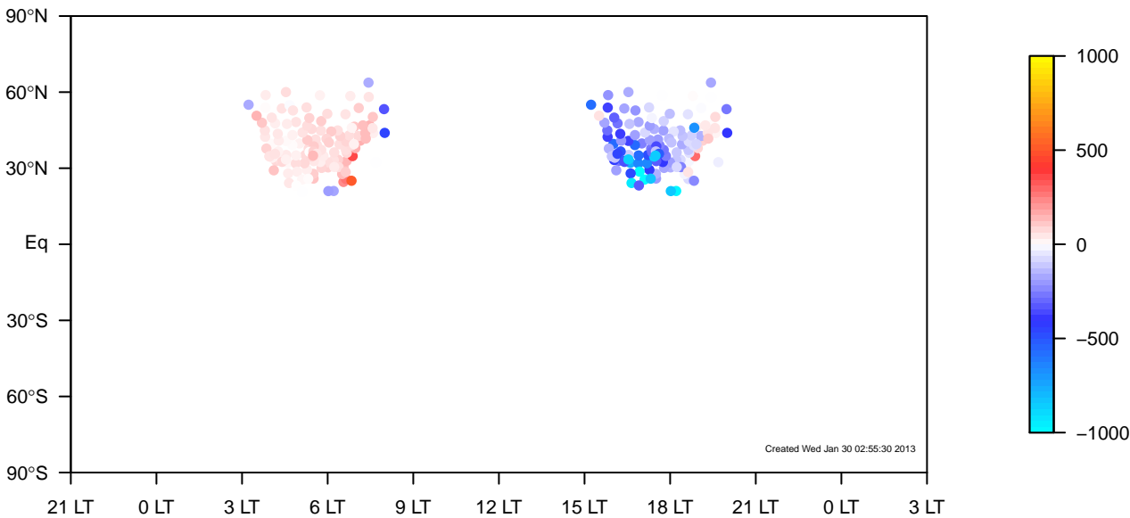
TM5-ei-nam1x1 minus IGRA all-season mixing height median (1995–2011)
