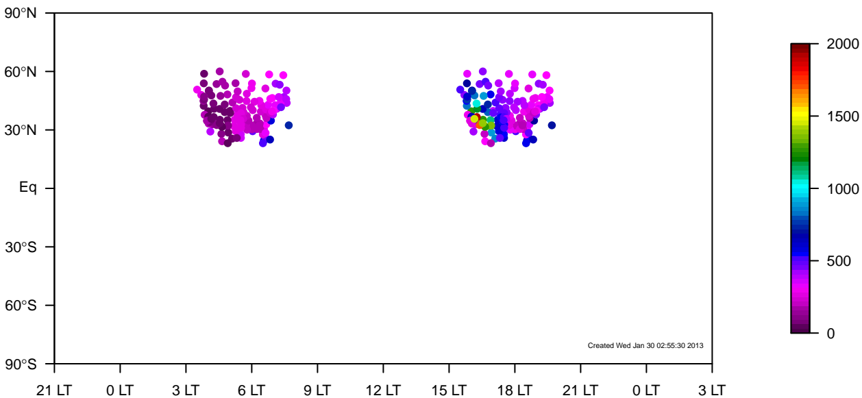
TM5-ei-nam1x1 all-season mixing height median (1995–2011)
