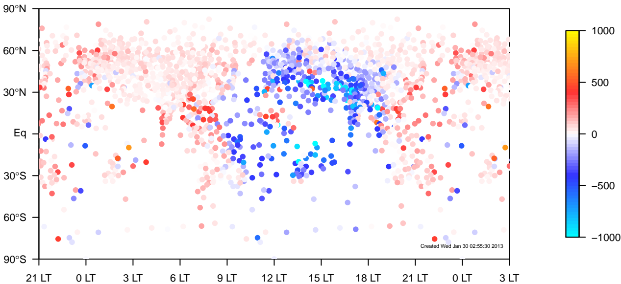
TM5-od-tmpp-glb3x2 minus IGRA all-season mixing height median (2000–2011)
