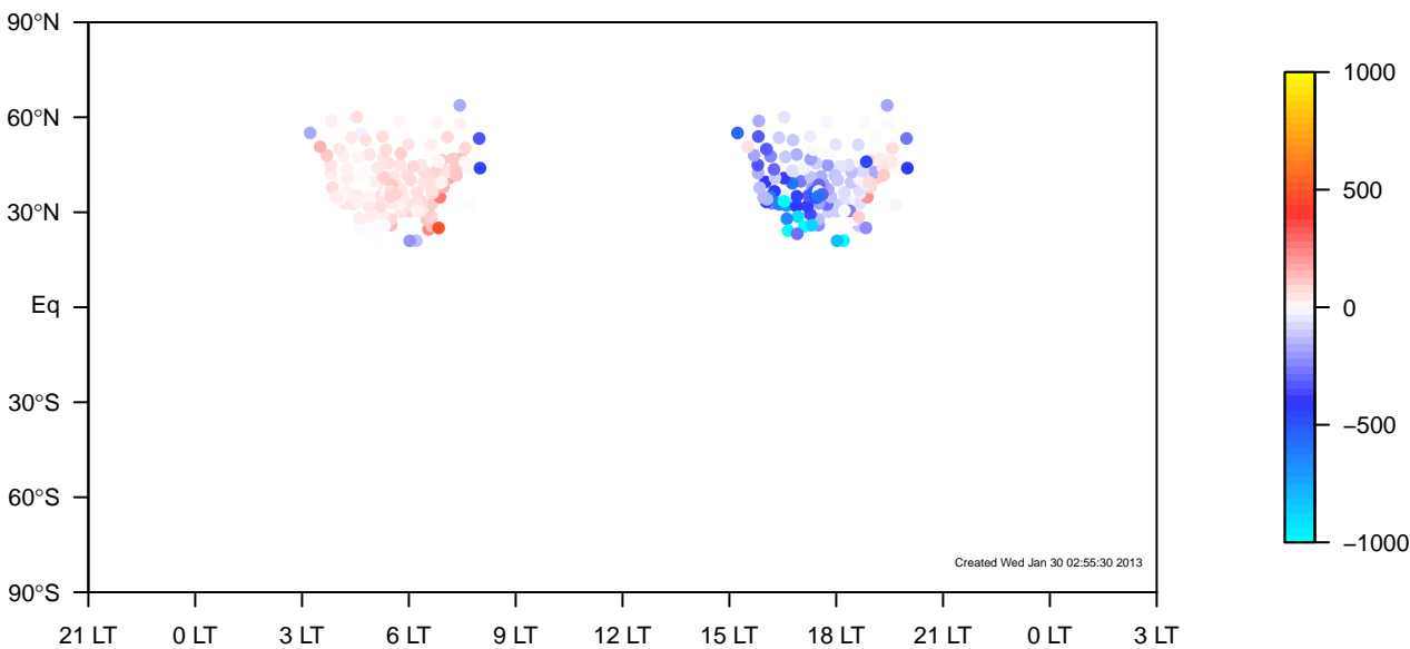
TM5-od-tmpp-nam1x1 minus IGRA all-season mixing height median (2000–2011)
