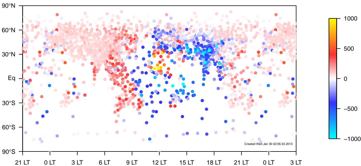
internal-TM5-ei-glb3x2 minus IGRA all-season mixing height median (1995–2011)
