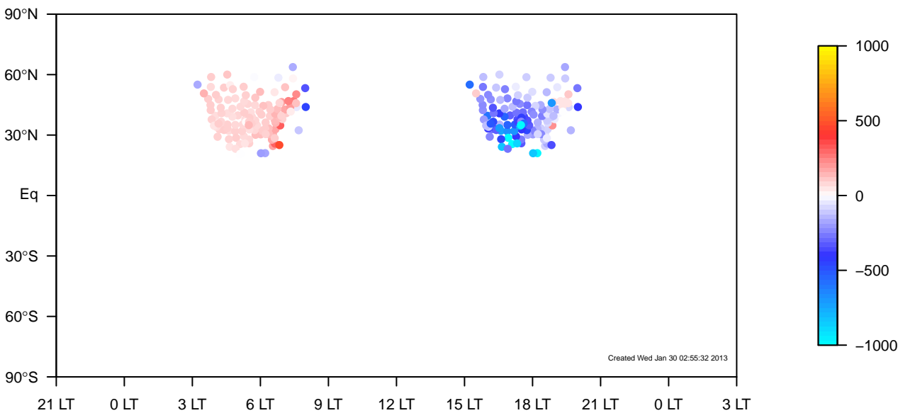
internal-TM5-ei-nam1x1 minus IGRA all-season mixing height median (1995–2011)
