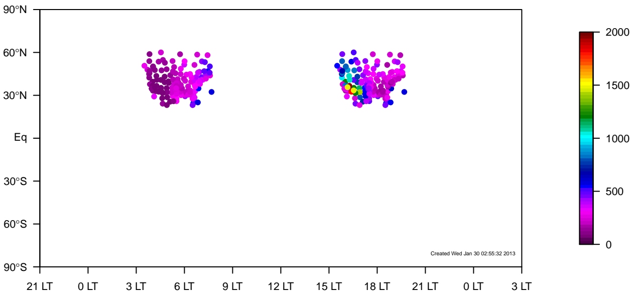
internal-TM5-ei-nam1x1 all-season mixing height median (1995–2011)
