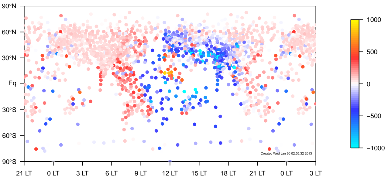
internal-TM5-od-tmpp-glb3x2 minus IGRA all-season mixing height median (2000–2011)
