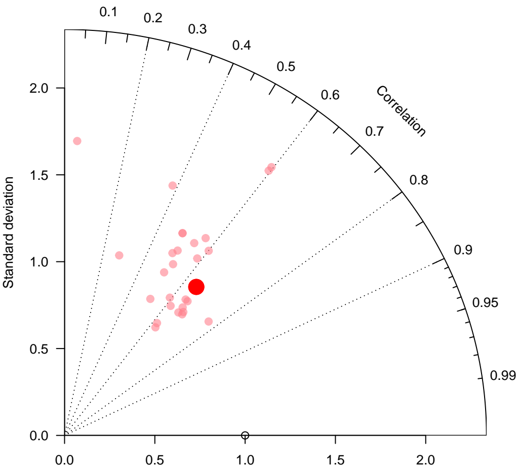
ERA-i for 0 local solar time +/- 3 hours
