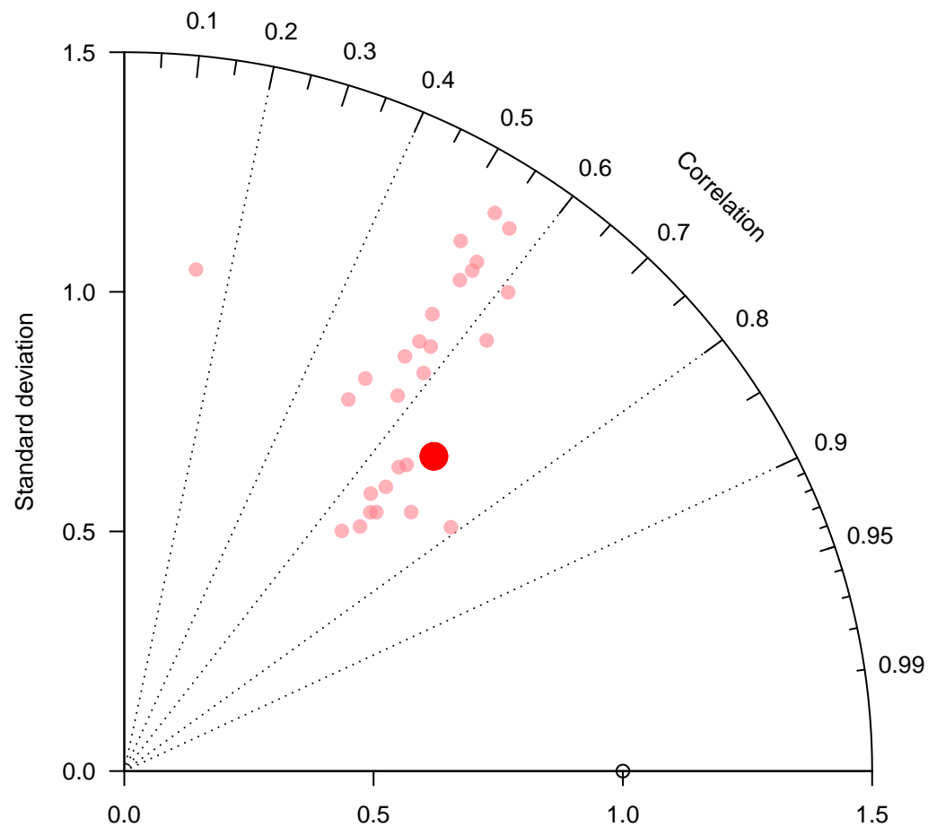
ERA-i for 12 local solar time +/- 3 hours
