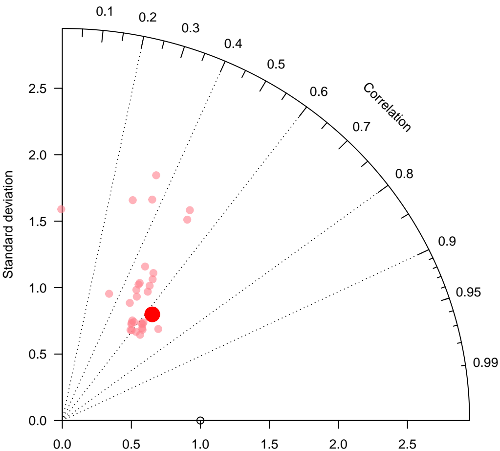
ERA-i for 6 local solar time +/- 3 hours
