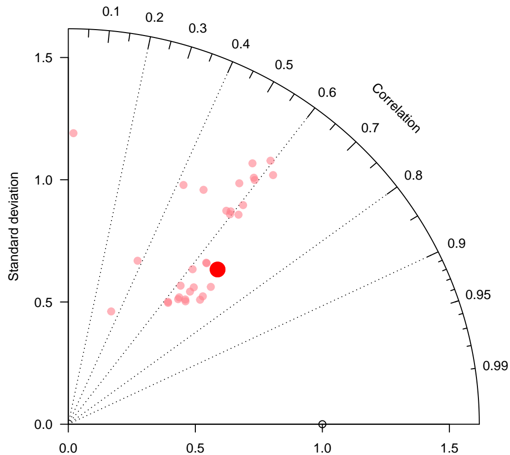
ERA-i for 18 local solar time +/- 3 hours
