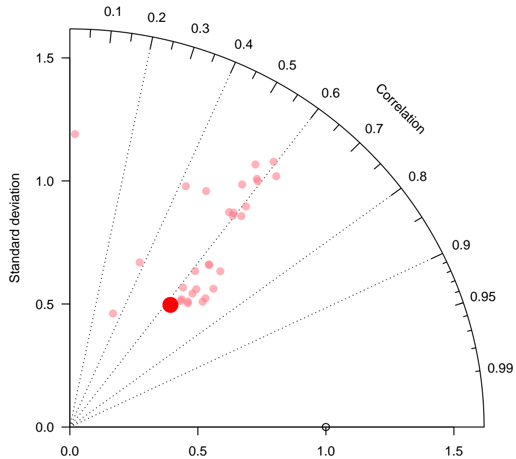
TM5-ei-glb3x2 for 18 local solar time +/- 3 hours
