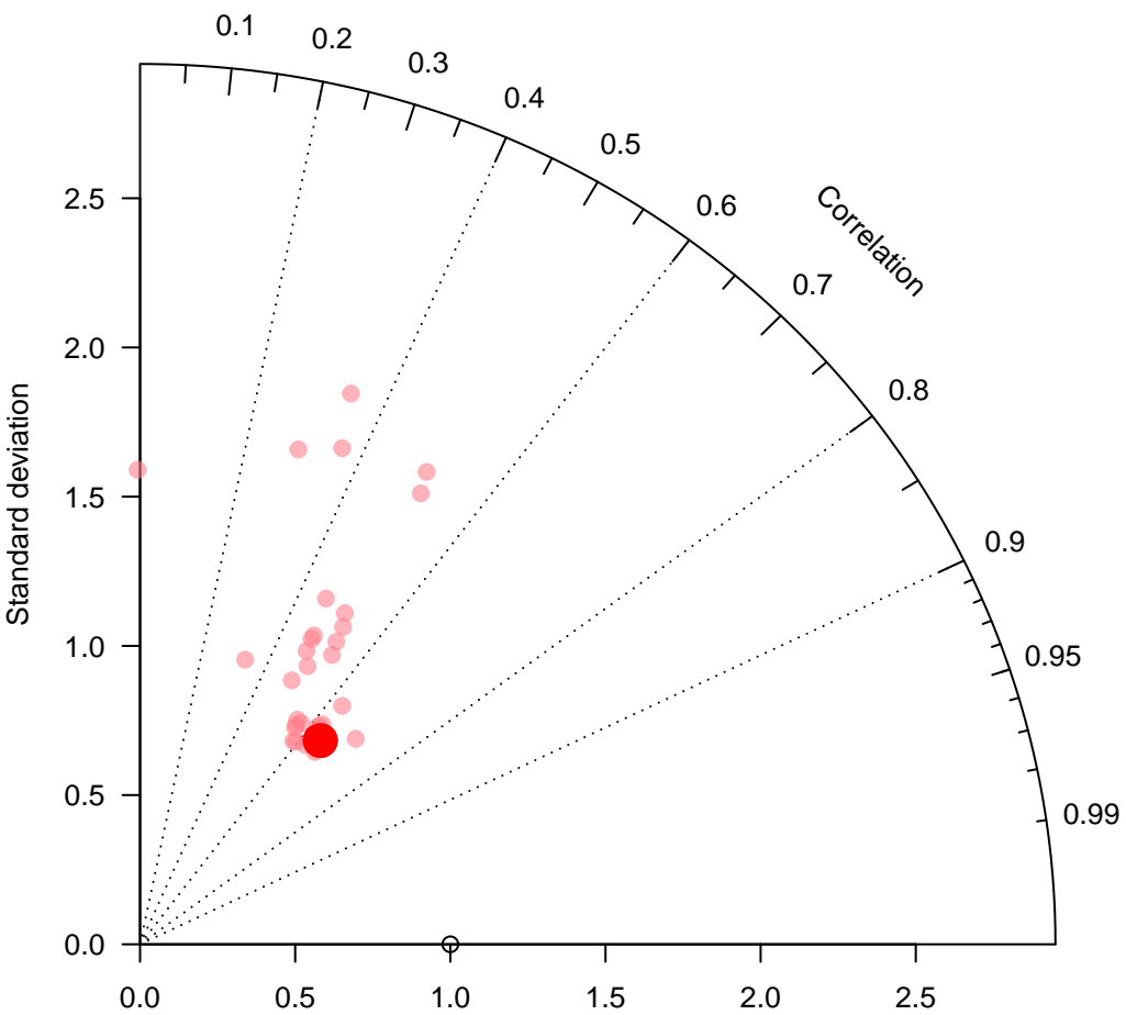
TM5-ei-glb3x2 for 6 local solar time +/- 3 hours
