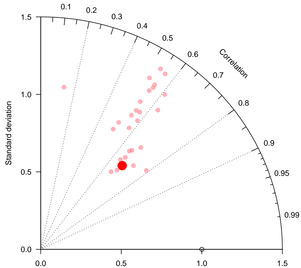
TM5-ei-glb3x2 for 12 local solar time +/- 3 hours
