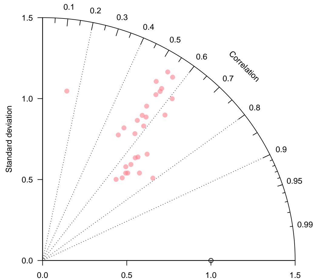
internal-TM5-ei-nam1x1 for 12 local solar time +/- 3 hours
