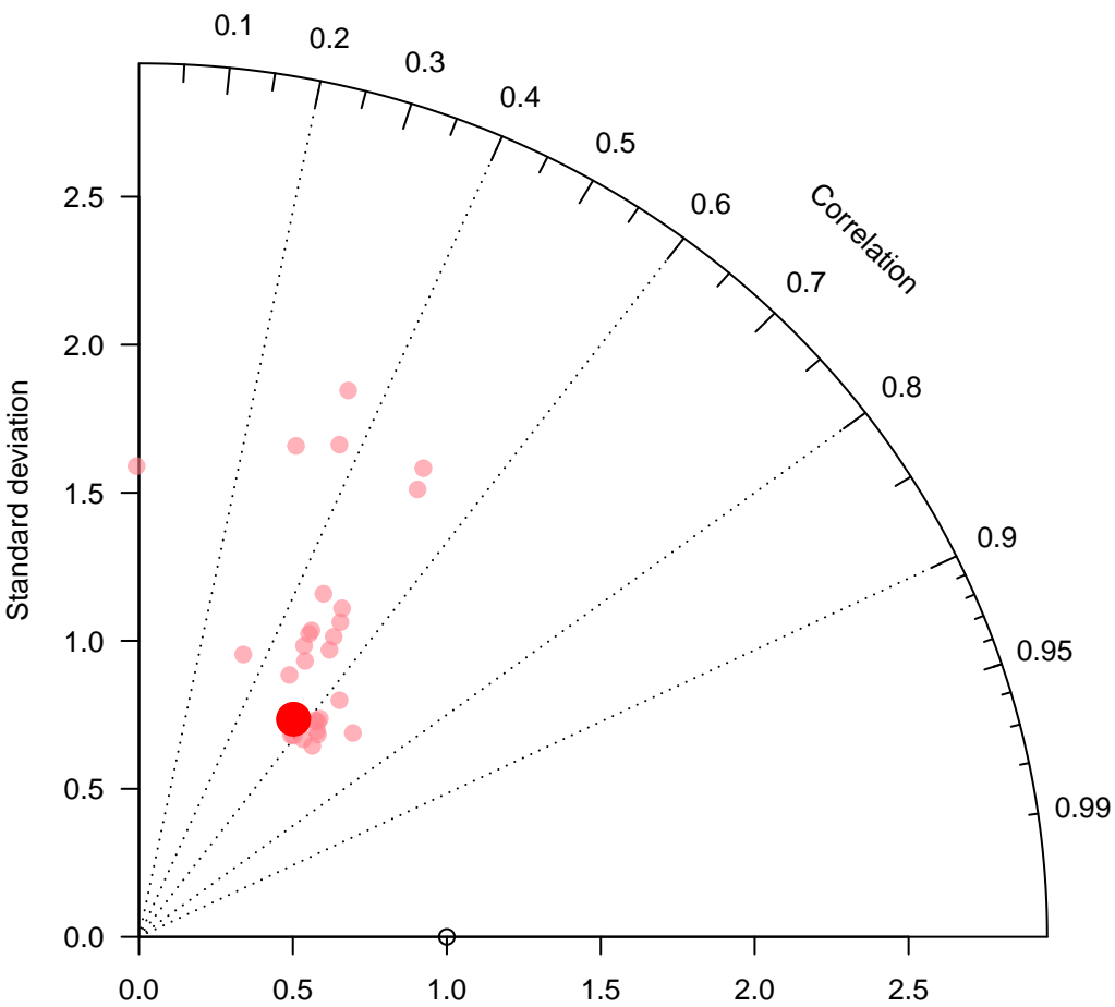
internal-TM5-ei-nam1x1 for 6 local solar time +/- 3 hours
