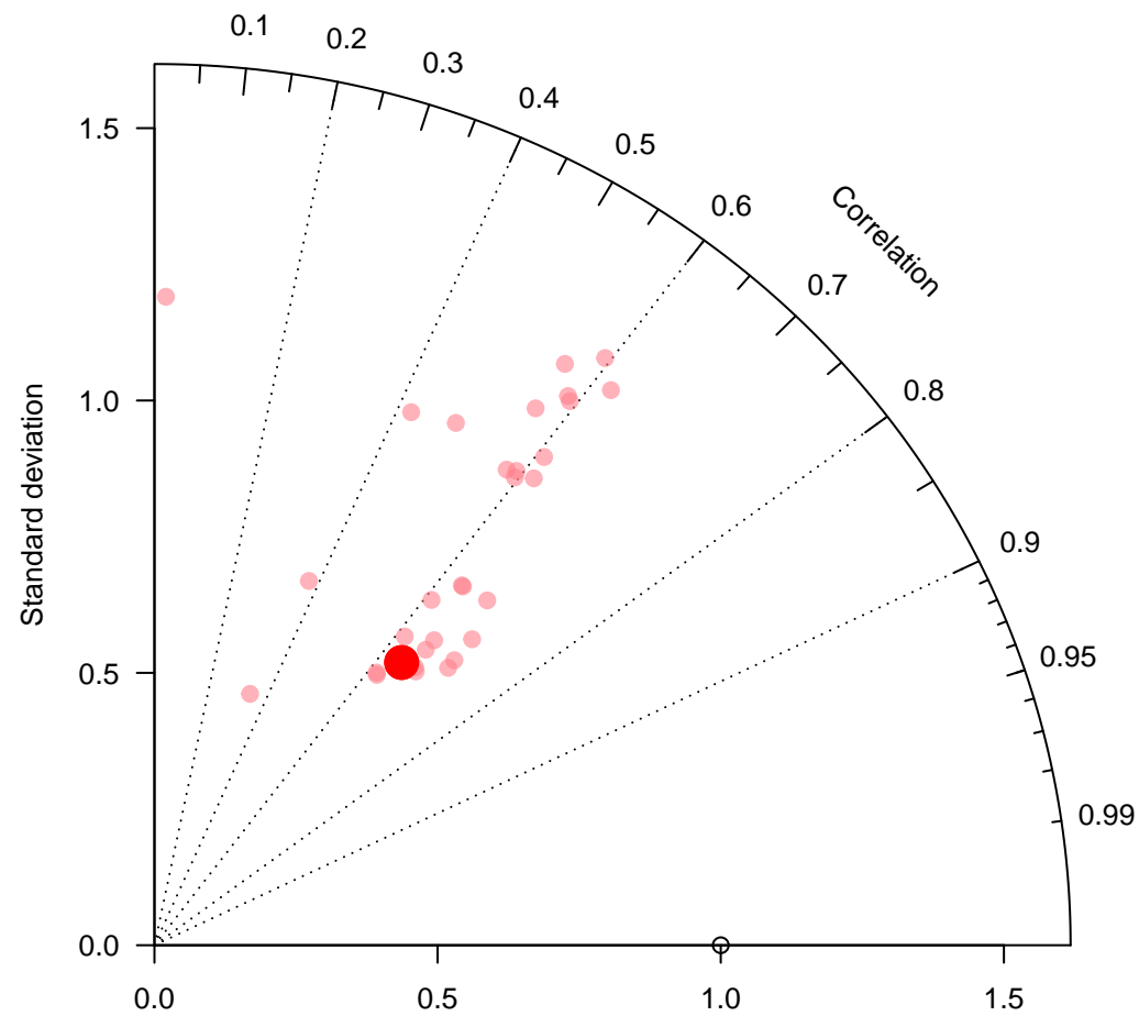
internal-TM5-ei-nam1x1 for 18 local solar time +/- 3 hours
