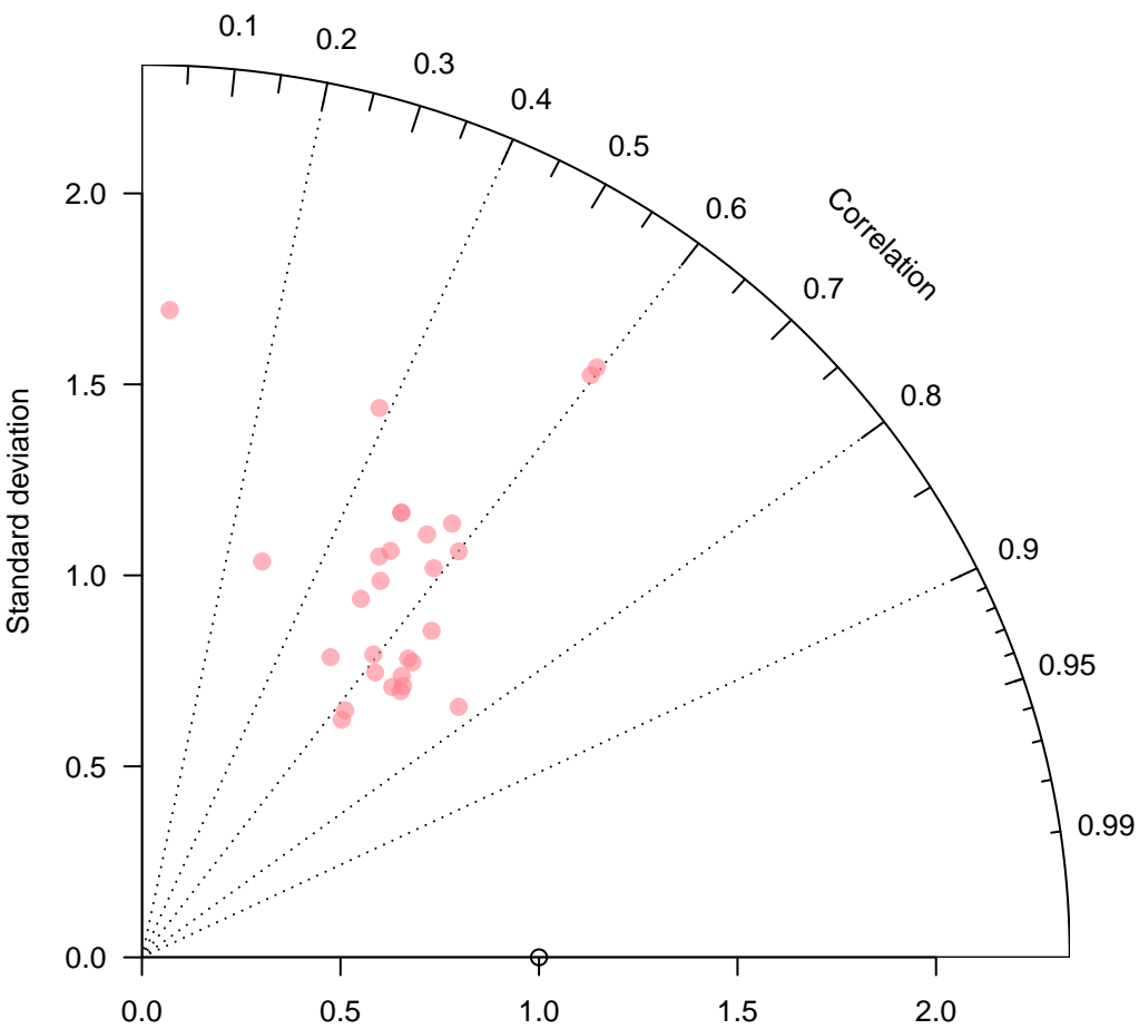
internal-TM5-ei-nam1x1 for 0 local solar time +/- 3 hours
