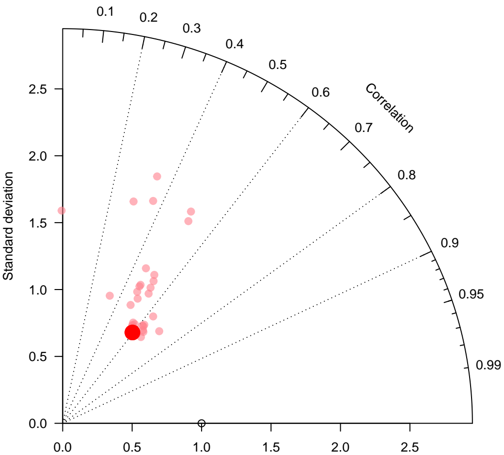
internal-TM5-od-tmpp-glb3x2 for 6 local solar time +/- 3 hours
