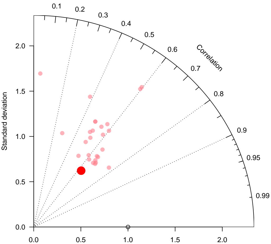
internal-TM5-od-tmpp-glb3x2 for 0 local solar time +/- 3 hours
