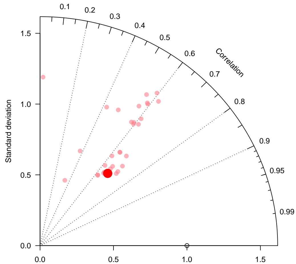
internal-TM5-od-tmpp-glb3x2 for 18 local solar time +/- 3 hours
