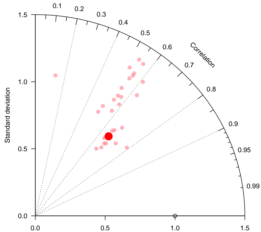
internal-TM5-od-tmpp-glb3x2 for 12 local solar time +/- 3 hours
