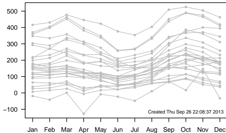
12UTC model-IGRA MHs, stations centered on dateline
