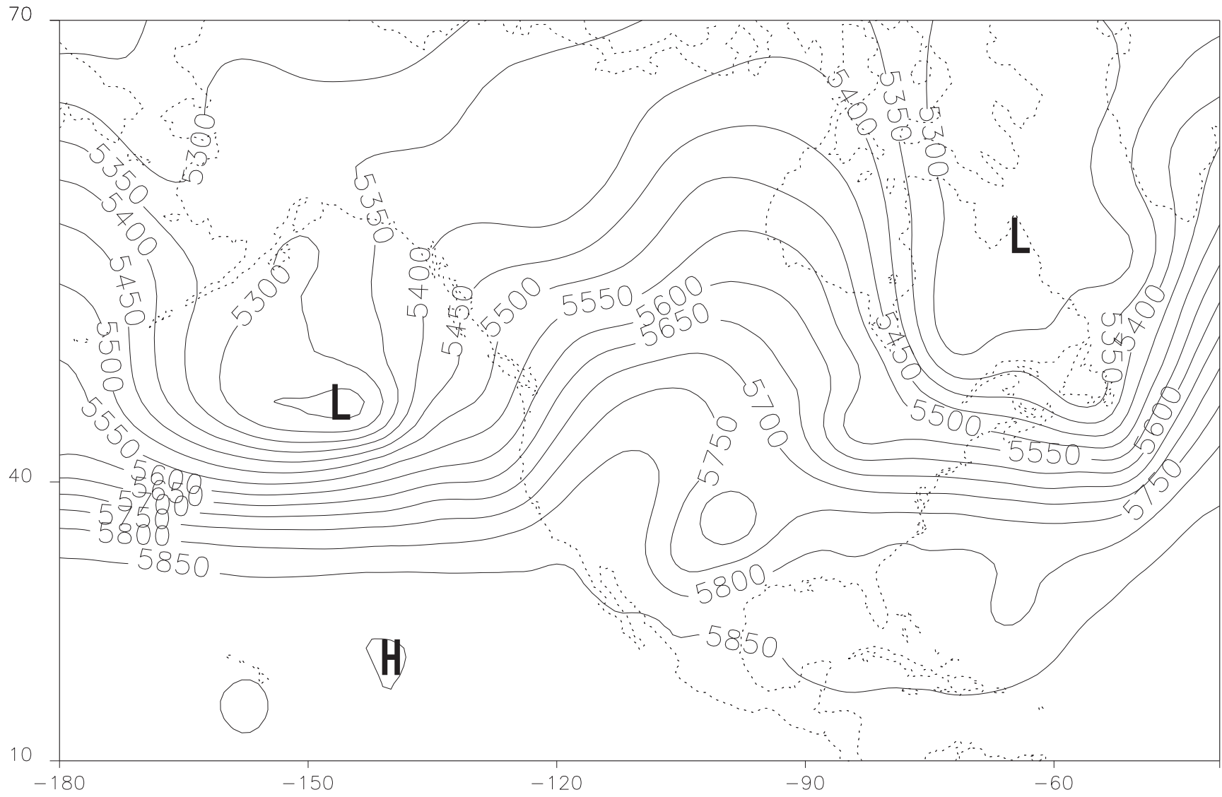
Elevation (m) of the 500 hPa Surface on 2000/5/2 at 0UT
