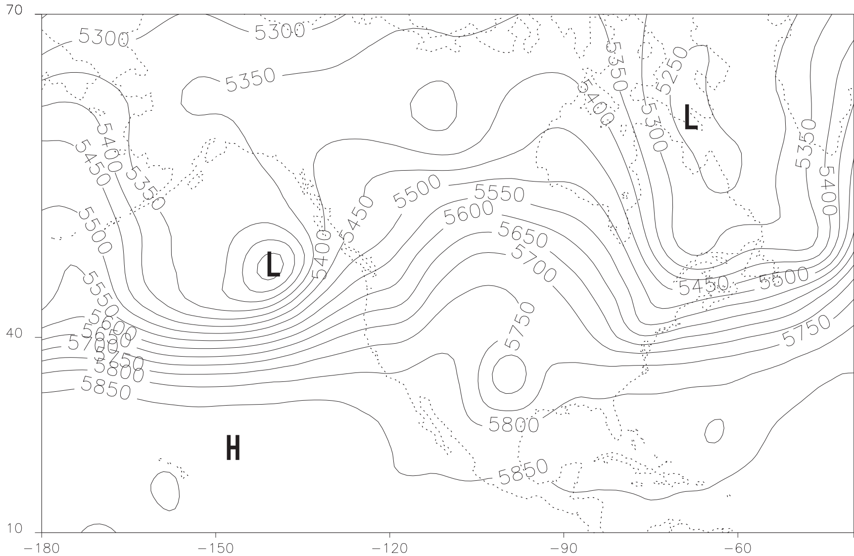
Elevation (m) of the 500 hPa Surface on 2000/5/2 at 12UT
