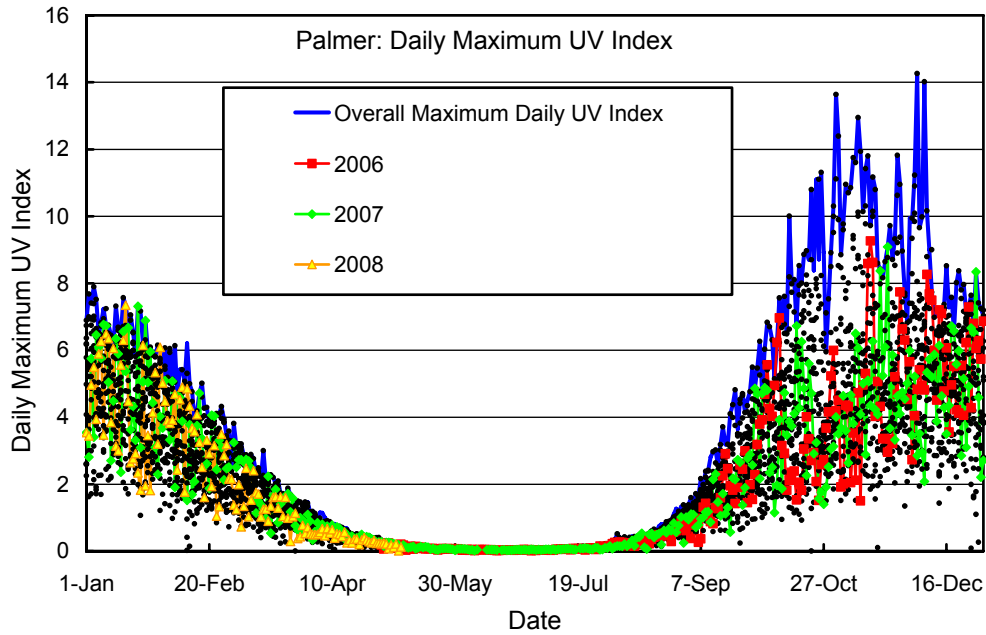
Figure 7.2.3. The daily maximum UV Indices at Palmer Station measured between 2006 and 2008 are compared with UV Indices measured between 1991 and 2005. The overall maximum daily UV Indices are also highlighted.
