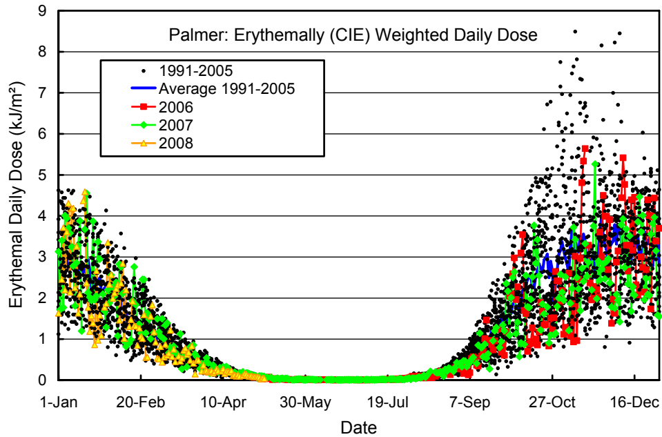
Figure 7.2.5. Daily erythemal dose for Palmer. Volume 16 and Volume 17 measurements from the years 2006-2008 are compared with individual data points and the average of measurements taken between 1991 and 2005.
