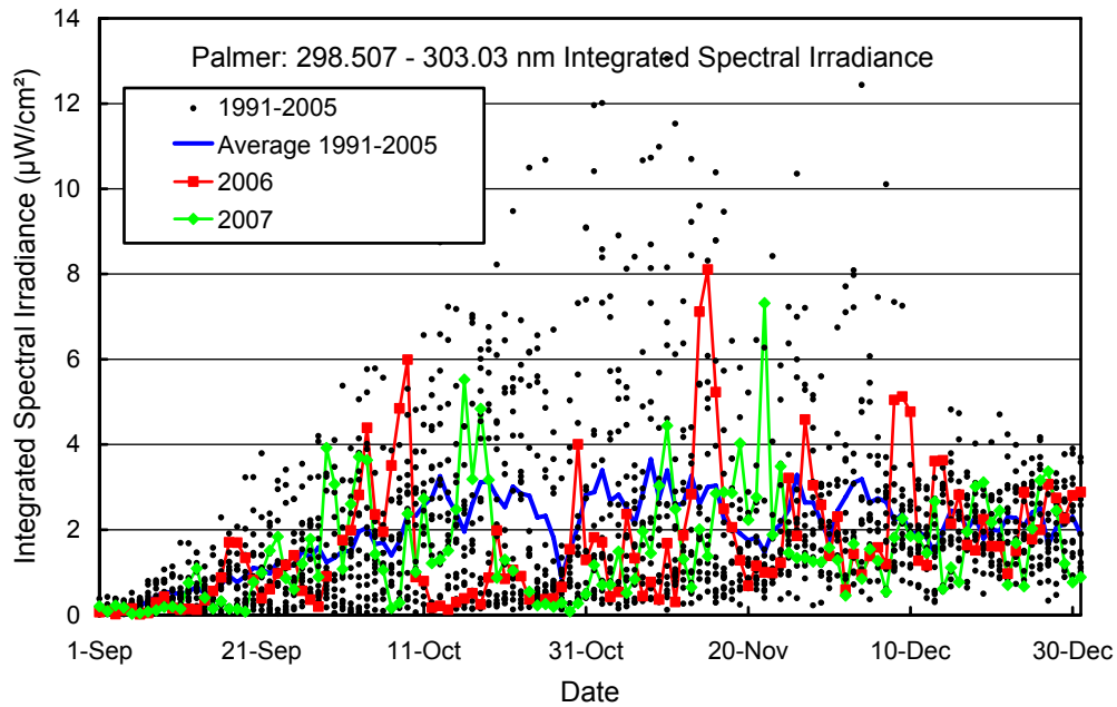
Figure 7.2.2. Noontime integrated spectral UV irradiance (298.51 - 303.03 nm) at Palmer. Measurements from 2006 and 2007 are compared with individual data points and the average of measurements taken between 1991 and 2005.
