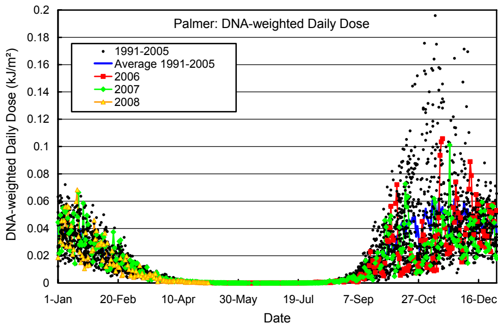
Figure 7.2.4. Daily DNA-weighted dose for Palmer. Volume 16 and Volume 17 measurements from the years 2006-2008 are compared with individual data points and the average of measurements taken between 1991 and 2005.
