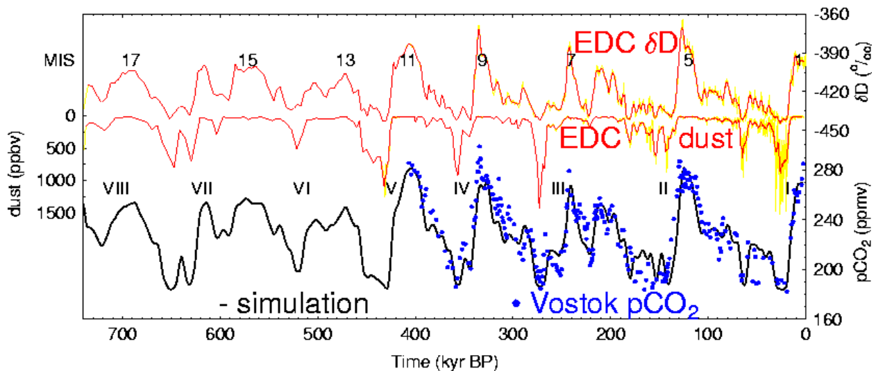
Fig. 1. Simulated and measured atmospheric p\text{CO}_2 over the EDC period. Additionally EDC deuterium and dust records are shown [EPICA community members, 2004]. Vostok p\text{CO}_2 data [Petit et al., 1999] plotted on the orbitally tuned age scale [Shackleton, 2000]. Marine Isotope Stage (MIS) during interglacials and Terminations I to VIII are labeled.
