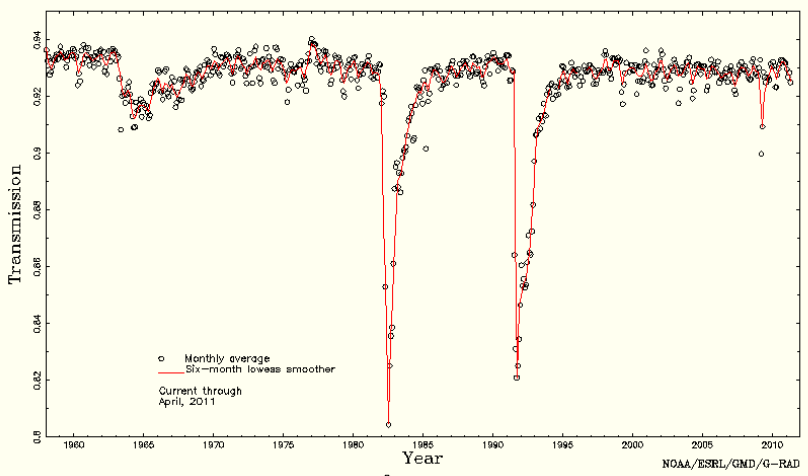
Mauna Loa Apparent Transmission (Preliminary)
