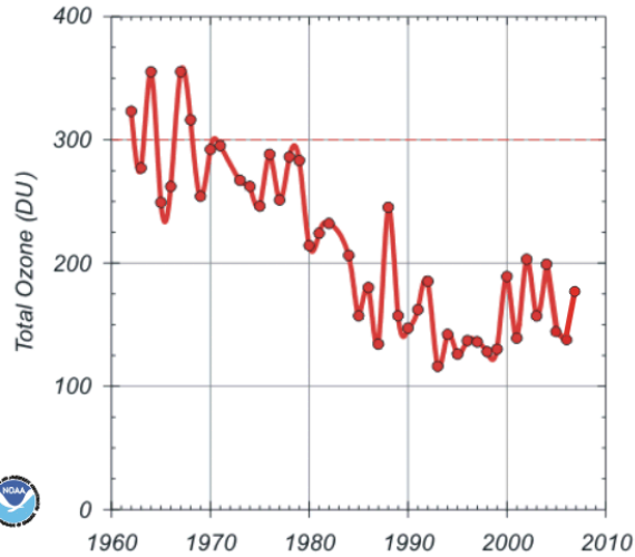
South Pole Dobson Ozone Spectrophotometer October 15-31 Average
