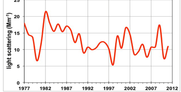
Arctic Haze at Barrow (April average)
