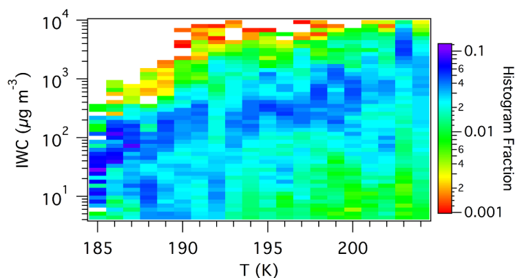
Figure 1. Distribution of observed TTL cirrus ice water content as a function of temperature during the ATTREX campaign. Values were typically less than 1 \text{ mg m}^{-3} and frequently below 50 \mu\text{g m}^{-3} at colder temperatures. The ATTREX data set provides an outstanding basis to study the mass-dimensional relationship of TTL cirrus in this important region.
